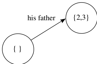
Figure 6.2: Lattice generation: each node in the source-aligned lattice corresponds to a set of source words that have been translated (coverage vector). An arc corresponds to a translation of one or more source words, be it a word or a longer phrase. All paths leading to the same node have exactly translated the same set of source words.
