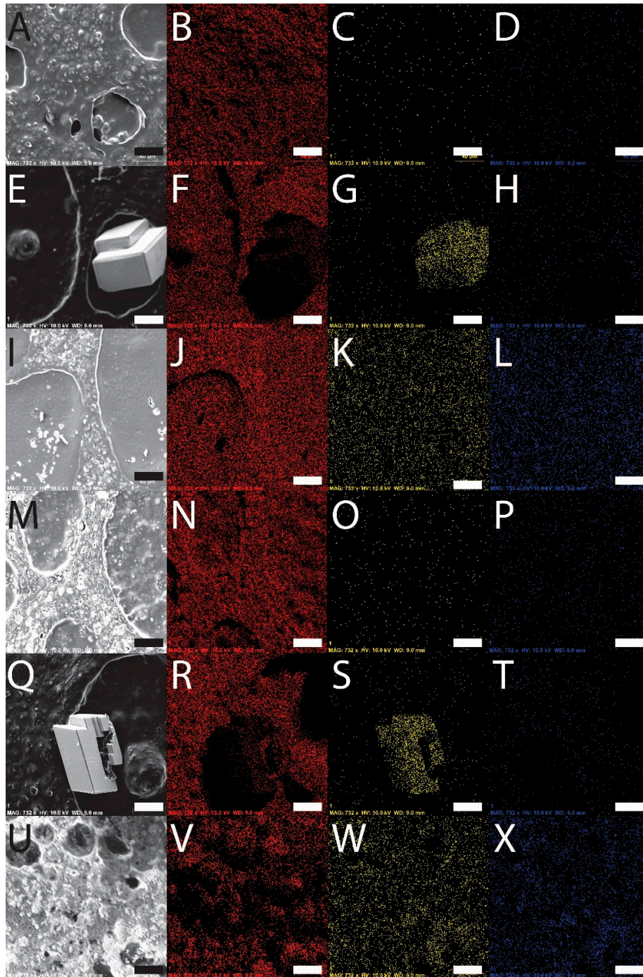
Figure 2. SEM-EDS analysis of films. (A–D) PBT-50; (E–H) PBT-50- \text{CaCO}_3 ; (I–L) PBT-50- \text{CaPO}_4 ; (M–P) PBTAT-50; (Q–T) PBTAT-50- \text{CaCO}_3 ; (U–X) PBTAT-50- \text{CaPO}_4 ; (A,E,I,M,Q,U) secondary electron SEM image; (B,F,J,N,R,V) carbon, red; (C,G,K,O,S,W) calcium, yellow; (D,H,L,P,T,X) phosphorous, blue. The scale bar represents 40 \mu\text{m} .
