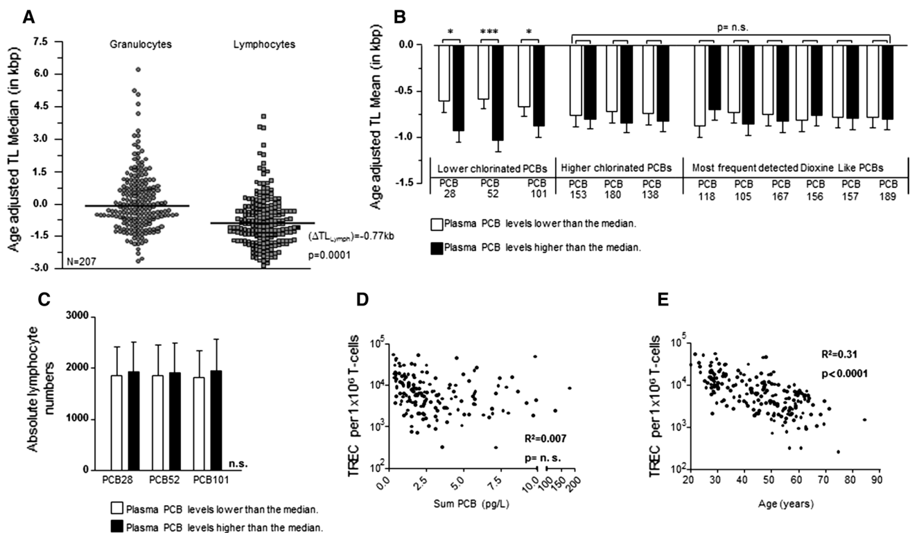
Fig. 1 a Median loss of TL in the peripheral blood of PCB-exposed individuals measured by flow-FISH. TL is expressed as age-adjusted telomere length ( \Delta Tel) and was calculated based on the TL of 104 unexposed individuals reported on previously. b Mean \pm SD \Delta Tel of lymphocytes for individual indicator PCBs depending on plasma concentration. Lower and higher concentrated plasma PCB levels were separated using the median value as cutoff. c Total lymphocyte numbers as determined by automated blood counting according to plasma
