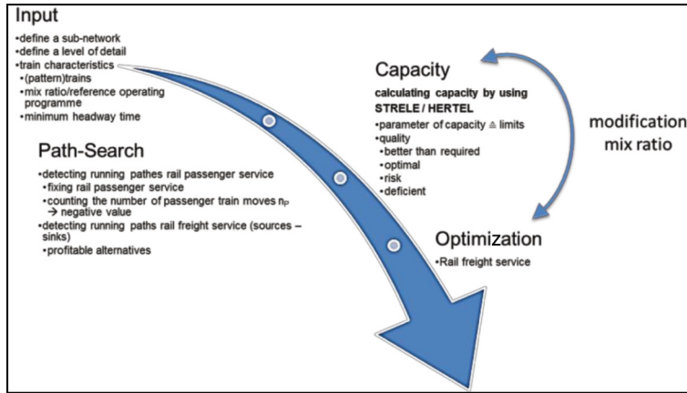
Figure 4: Optimization flowchart.
