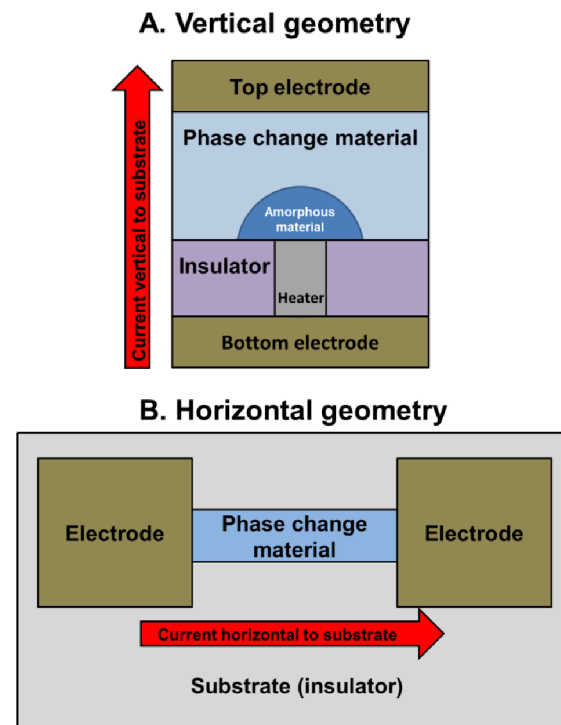
Figure 14: Electronic phase change memory cell layouts are showing two main layouts. (A) In vertical geometry the current flows orthogonal to the substrate surface. (B) In horizontal cells the current flows parallel to the substrate surface (Lankhorst et al., 2005; Kau et al., 2009; Raoux, 2009; Oosthoek, 2014a).
