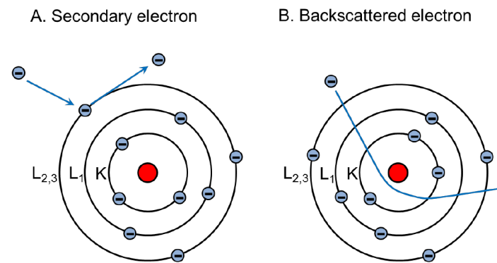
Figure 18: Shown are the schematic drawings of the creation of secondary electrons (A) and backscattered electrons (B). Secondary electrons are leaving their shell after energy transfer from a high energetic electron. Backscattered electrons are high energetic electrons that get scattered back by the nuclei of the sample atoms.
