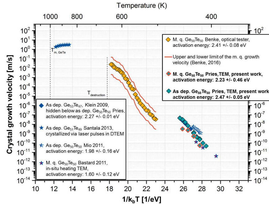
Figure 91: Shown are measured and simulated growth velocities of as deposited and melt quenched GeTe performed by different methods in comparison (Klein, 2009; Bastard et al., 2011; Mio et al., 2011; Santala et al., 2012; Pries, 2015; Benke, 2017). Image reprinted and amended with permission from the thesis of J. Benke (Benke, 2017).
