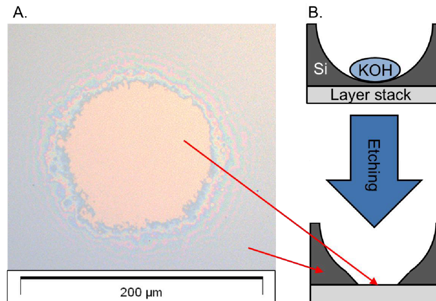
Figure 46: (A) Shown is a light microscope image of a typical electron transparent specimen window. (B) Shown is a schematic drawing of the specimen before and after the etching process. The red arrows connect the related regions between the light microscope image and the scheme.
