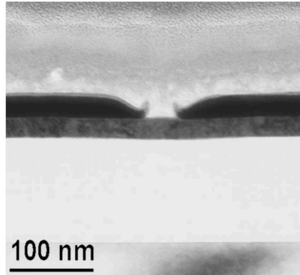
Figure 71: Shown is a closer look at the gap between the electrodes of the reference line cell. Even at this magnification dark Bragg contrast of grains can be seen through the whole AIST layer.
