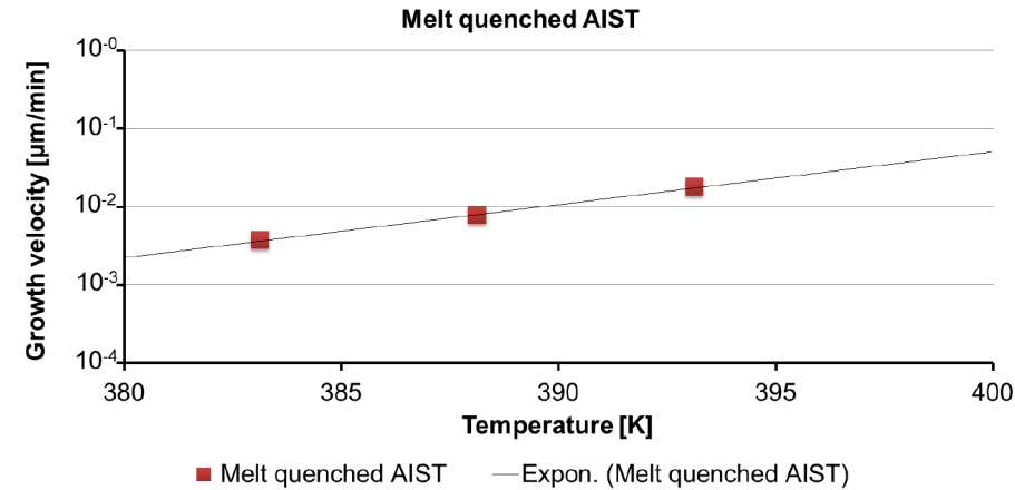
Figure 56: The growth velocity of melt quenched AIST shows Arrhenius like behaviour and increases with increasing temperature. Error bars are hidden behind the markers.
