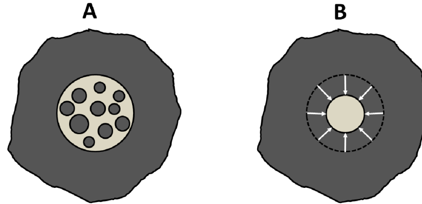
Figure 8: Schematic drawing of the two crystallization mechanisms of nucleation dominated phase change materials and growth dominated phase change materials. (A) Nucleation dominated phase change materials transform a given amorphous area by nucleation and followed growth of the nuclei. (B) Growth dominated phase change materials transform this amorphous area by crystal growth of the crystalline rim into the centre before significant nucleation can occur (Zhou, 2001).
