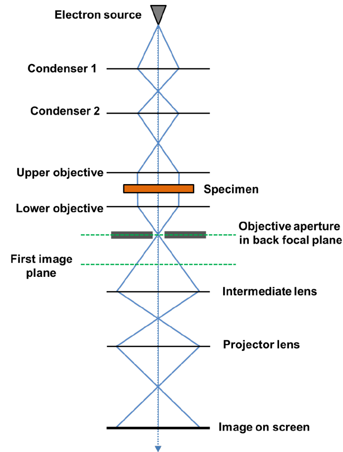
Figure 25: Shown is the schematic beam path of an uncorrected TEM.
