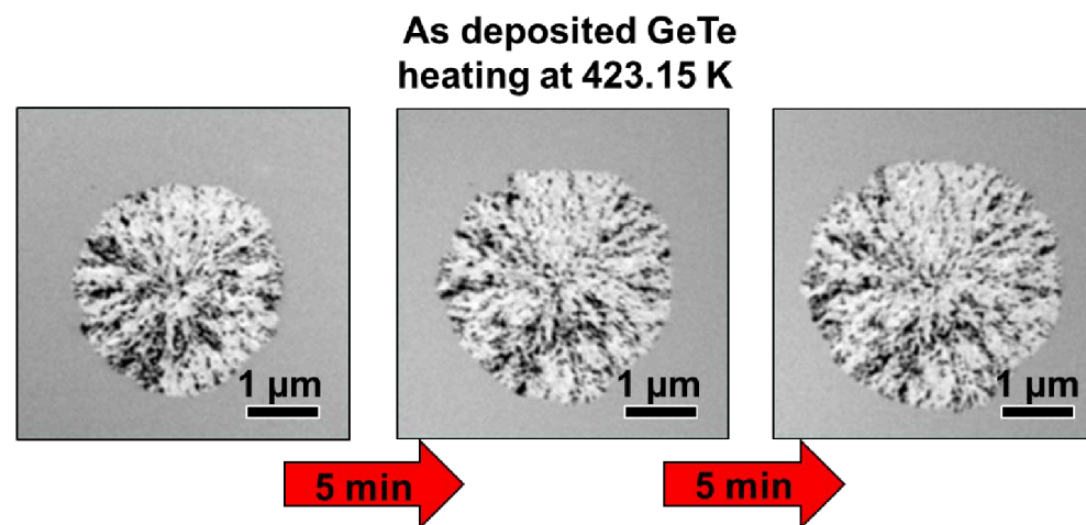
Figure 58: Shown is a single grain in as deposited GeTe growing from ex situ heating.
