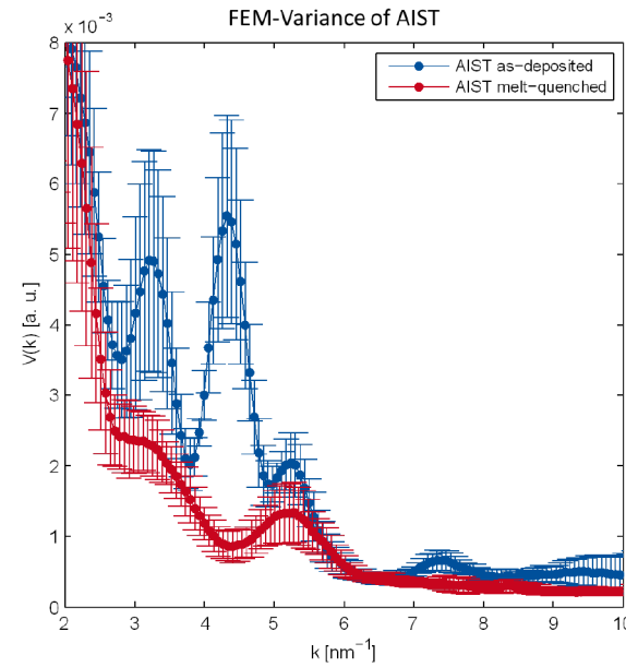
Figure 67: The thickness corrected variance in relation to the scattering vector k shows increased MRO in the as deposited state of AIST.
