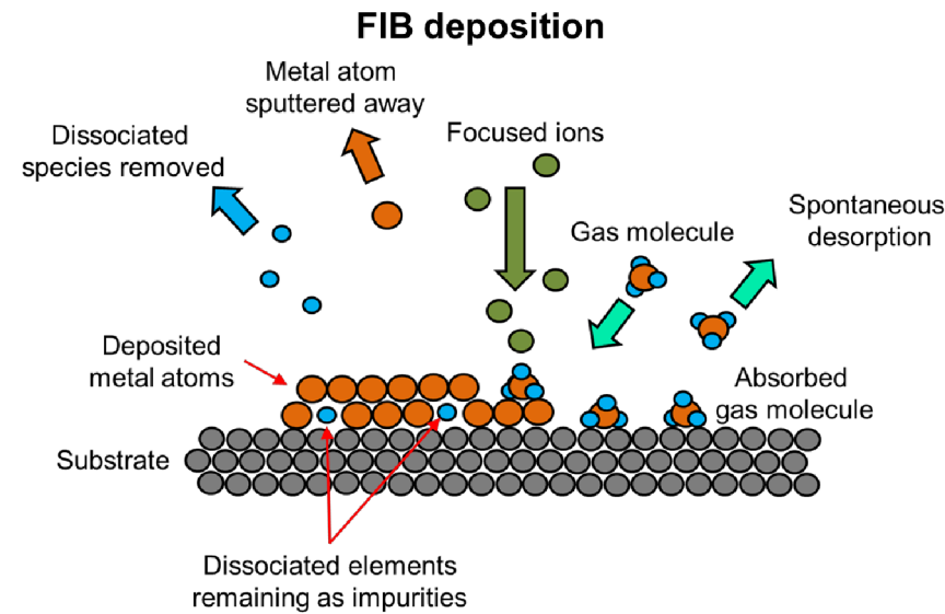
Figure 23: Shown is a schematic drawing of metal deposition by cracking a precursor gas with gallium ions. The gallium ions crack the precursor gas into the metal atoms and a volatile species. The metal ions are deposited on the sample surface while the volatile species is pumped away.
