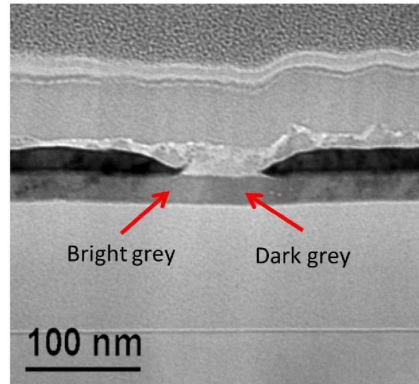
Figure 74: Shown is a closer look at the gap between the electrodes. The AIST layer beneath the electrode lacks dark Bragg contrast of orientated grains. The grey of the AIST material beneath the gap is on the left hand side brighter than on the right hand side.
