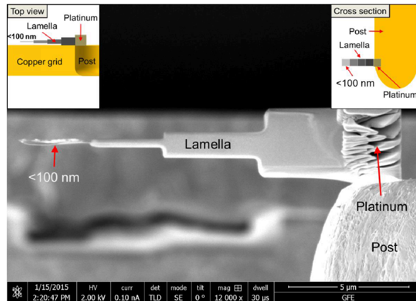
Figure 49: In this top view of a finished cross section TEM lamella from a step by step thinning is shown. The thinnest part of the lamella on the left is a very thin (thickness < 100 nm) foil. A slight bending of the foil is observable. Schematic drawings of the cross section and top view of the thinned lamella are shown to explain the geometry.
