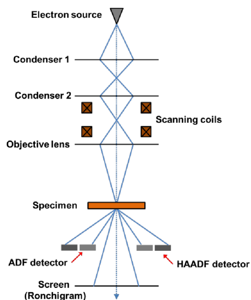
Figure 29: Shown is the scheme of an uncorrected STEM.
