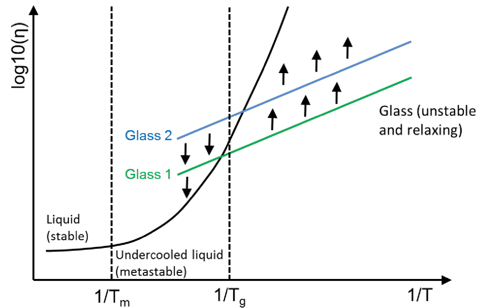
Figure 12: Schematic graph of the viscosity related to the reciprocal temperature. Above the melting temperature T_m the phase change material is in the liquid state. Below T_m the phase change material becomes an undercooled liquid with high enough mobility of the atoms to maintain a metastable equilibrium. When the mobility of the atoms gets too low around the glass transition temperature T_g the phase change material freezes as an amorphous non-equilibrium glass. Faster cooling of the phase change material causes an earlier freezing of the material in the glassy state (Glass 1). Slower cooling causes a delayed transition (Glass 2). At indefinitely slow cooling the metastable equilibrium keeps intact and the material stays in the undercooled liquid state. The glass is not stable and the configuration of the atoms relaxes in direction of the metastable equilibrium of the undercooled liquid indicated by the arrows (Raoux, 2009).
