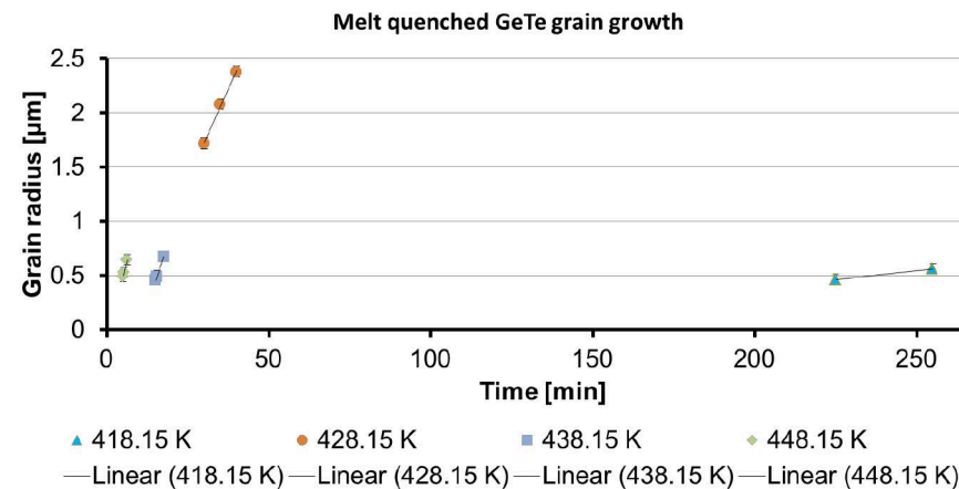
Figure 62: Shown are examples of the growing melt quenched GeTe grain radii over heating time. The linear fits are used to calculate the slopes and therefore the growth velocities of the grains. The starting point of a measurement of a grain is the first time the grain was found in the TEM after a heating cycle. Error bars are partly hidden behind the markers.
