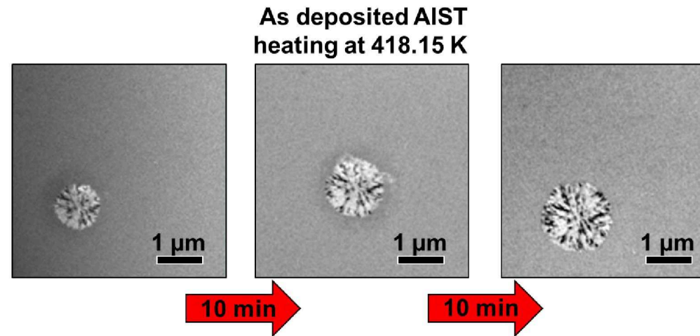
Figure 51: Shown is a single grain in as deposited AIST growing from ex situ heating.
