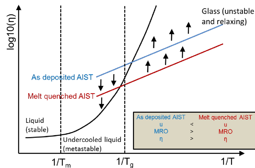
Figure 93: For AIST the melt quenched state is the state with the higher growth velocity u , has less amount of MRO, and is a less relaxed glassy state with lower viscosity \eta . Our as deposited state has a lower growth velocity u , higher amounts of MRO and is a more relaxed glass with a higher viscosity \eta .
