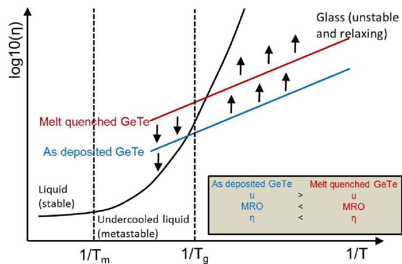
Figure 94: For GeTe our as deposited state is the state with the higher growth velocity u , has less amount of MRO, and is a less relaxed glassy state with lower viscosity \eta . The melt quenched state has a lower growth velocity u , higher amounts of MRO and is a more relaxed glass with a higher viscosity \eta .
