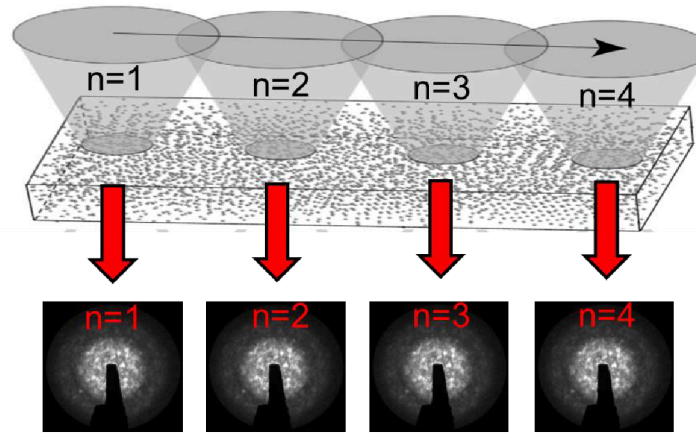
Figure 36: In FEM an electron probe scans over a sample acquiring a NAED pattern at every chosen spot. Higher order correlations of the atoms in the thin sample lead to intensity fluctuations in the NAED patterns.
