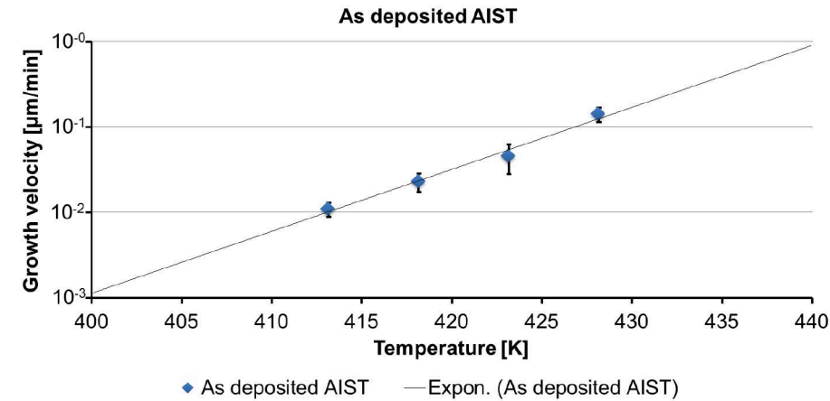
Figure 53: The growth velocity of as deposited AIST shows Arrhenius like behaviour with increasing temperature.
