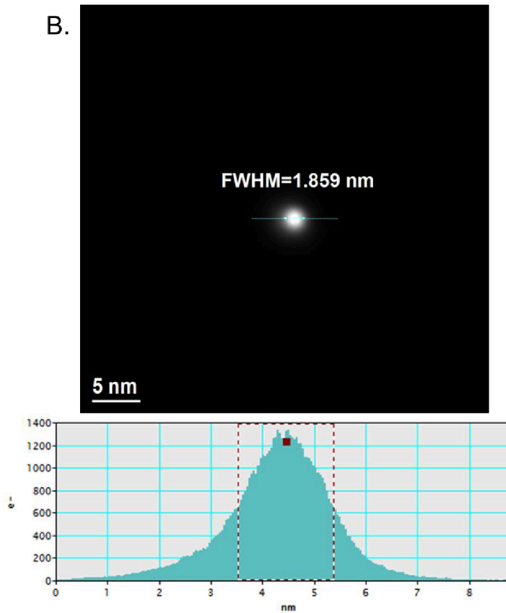
Figure 34: The size of the FWHM of the focused probe used for NAED can be measured after the calibration through the HRTEM images.
