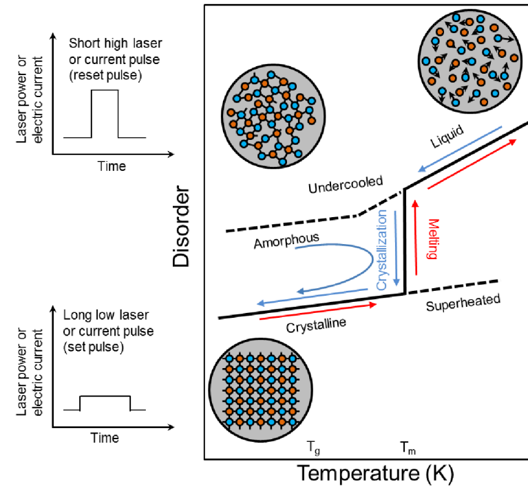
Figure 1: A phase change material is melted by a short high power laser or high electric current pulse (reset pulse; top left) which heats the phase change material above the melting temperature T_m . After the heating pulse rapid cooling freezes the phase change material in the amorphous phase. The amorphous phase change material is crystallized by a longer pulse (set pulse; bottom left). This pulse is lower in laser power or lower in electric current. The set pulse heats the phase change material to a temperature between the glass transition temperature T_g and T_m where rapid crystallization can occur (Wuttig & Yamada, 2007).
