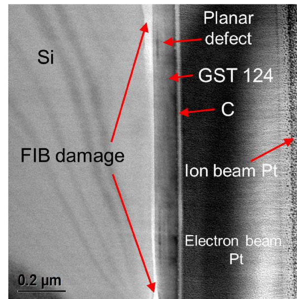
Figure 83: Bright field TEM image shows additional FIB damage artifacts. Also a planar defect can be seen in the GST 124 layer that runs through the whole lamella with uniform thickness. Image reprinted with acknowledgment from the publication of H. Hardtdegen and co-workers (Hardtdegen et al., 2016).
