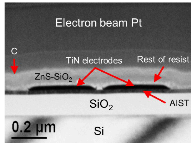
Figure 70: Shown is an overview bright field TEM image of the reference line cell. The different materials are clearly visible and labeled.
