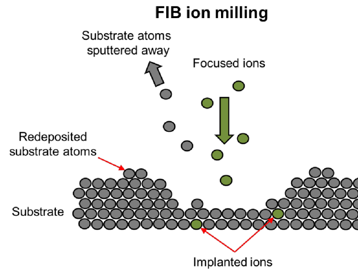
Figure 22: Shown is a schematic drawing of the process of sputtering away material of the sample with the focused gallium ions. The high energetic gallium ions transfer enough energy to the sample atoms to leave the sample surface. Some of these atoms redeposit on a different location on the sample. Some of the gallium ions also implant themselves into the sample.
