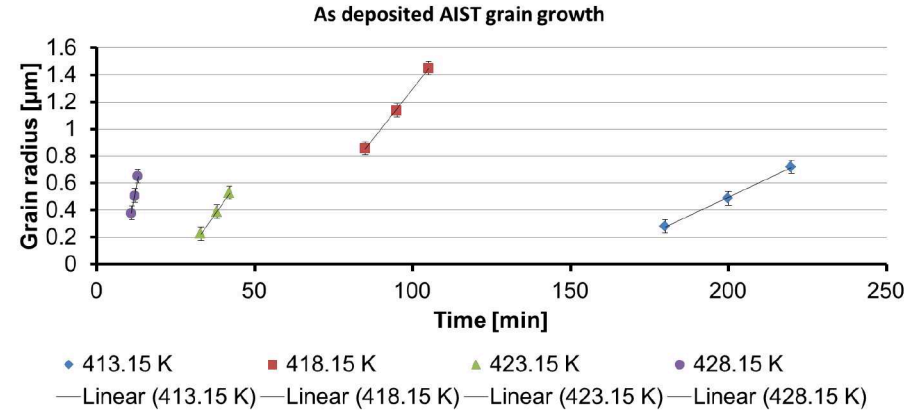
Figure 52: Shown are examples of the as deposited AIST grain radii over heating time. The linear fits are used to calculate the slopes and therefore the growth velocities of the grains. The starting point of a measurement of a grain is the first time the grain was found in the TEM after a heating cycle.
