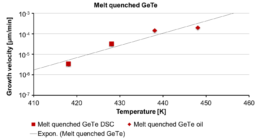
Figure 63: The growth velocity of melt quenched GeTe shows Arrhenius like behavior and increases with increasing temperature. The DSC and oil bath method are in good agreement. Error bars are behind the markers.
