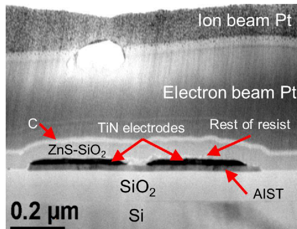
Figure 73: Shown is an overview bright field TEM image of the electrically switched line cell. The different materials are clearly visible and labelled.
