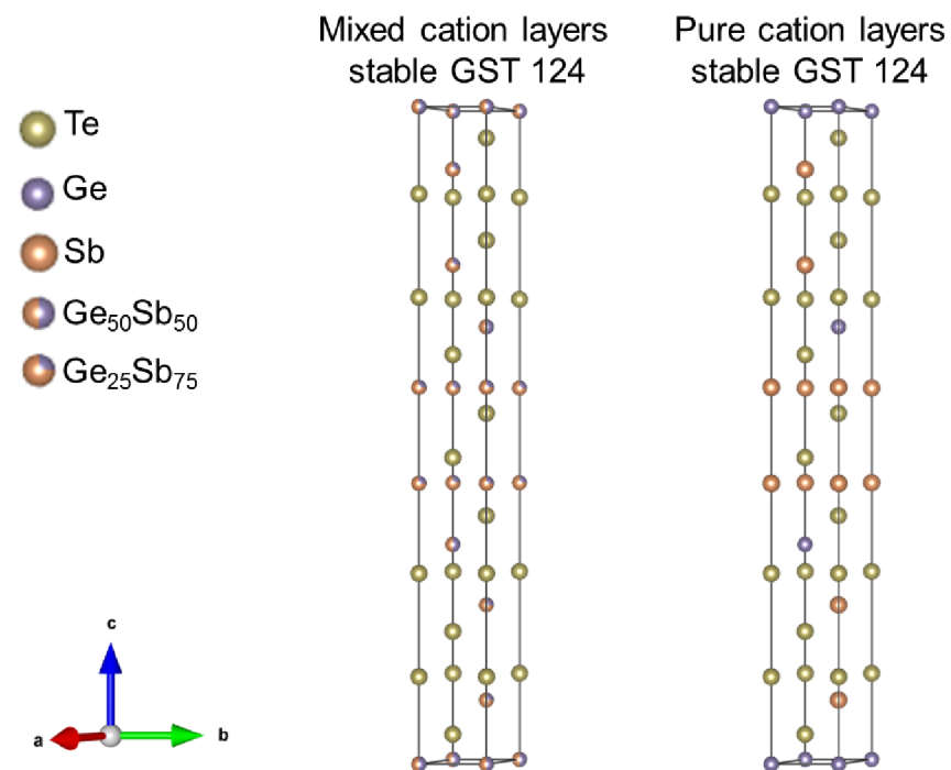
Figure 96: Shown are the both most commonly assumed stable hexagonal GST 124 structures (Matsunaga & Yamada, 2004; Da Silva et al., 2008) visualized by the 3D software VESTA (Momma & Izumi, 2011).
