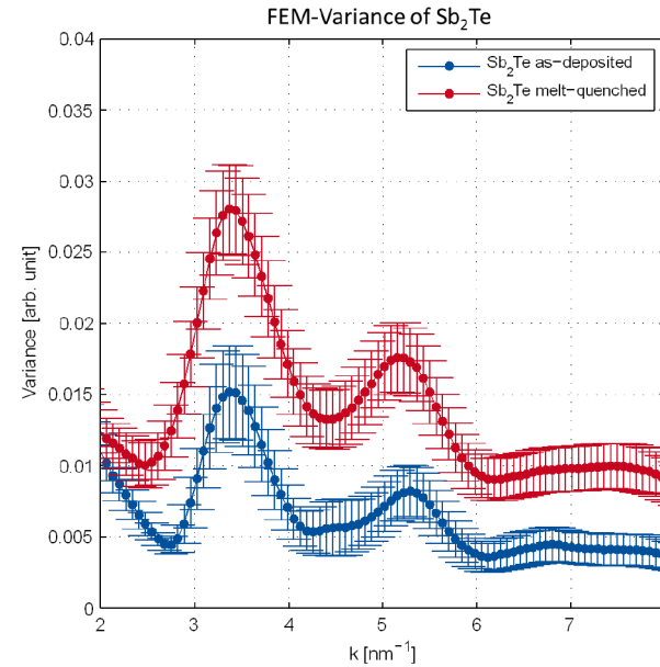
Figure 37: Shown are the variance plots in relation to the scattering vector k of as deposited and melt quenched \text{Sb}_2\text{Te} . Both graphs show an offset to each other.
