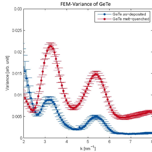
Figure 68: The variance of as deposited and melt quenched GeTe in relation to the scattering vector k . A comparison of peak heights is difficult because of an offset caused by thickness variations.
