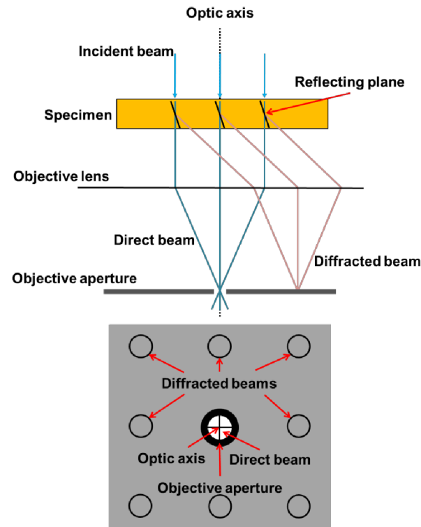
Figure 27: Shown is the working principle of the Bragg diffraction contrast in bright field images. Diffracted beams forming a diffraction pattern in the back focal plane are filtered out by the objective aperture.
