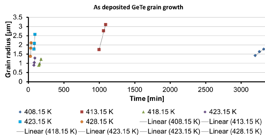
Figure 59: Shown are examples of the growing as deposited GeTe grain radii over heating time. The linear fits are used to calculate the slopes and therefore the growth velocities of the grains. The starting point of a measurement of a grain is the first time the grain was found in the TEM after a heating cycle. Error bars are partly hidden behind the markers.
