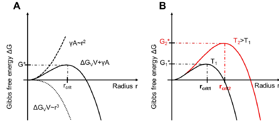
Figure 9: Graphs of the relation of the Gibbs free energy \Delta G and the radius r of an agglomeration of atoms with crystalline order. (A) If the radius of a nucleus is smaller than the critical radius r_{crit} it is energetically more favorable for the sub critical nucleus to decay. If the radius of the nucleus is larger than the critical radius r_{crit} it is energetically more favorable for the nucleus to grow. (B) The critical radius r_{crit} increases with increasing temperature T (Gibbs, 1906; Christian, 1965; Kelton, 1991; Friedrich, 2000; Raoux, 2009).
