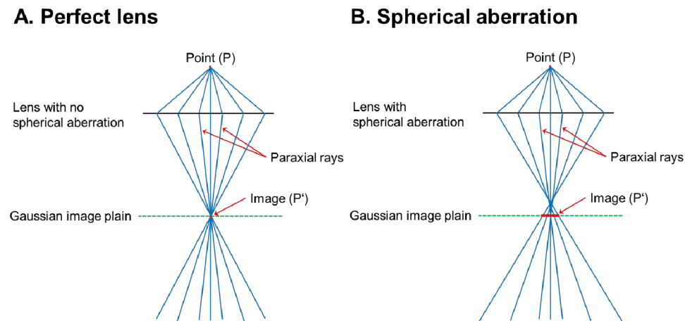
Figure 15: (A) In a perfect aberration free lens all beam rays image a point P in the Gaussian image plane as point P'. (B) Spherical aberration leads to differences in the beam path of the beam rays imaging a point P depending of their distance to the optical axis. Only paraxial rays which are very close to the optical axis meet at the Gaussian image plane correctly. Rays further away from the optical axis have a different focus point leading to blurring of the focus in the Gaussian image plane (Reimer & Kohl, 2008; Williams & Carter, 2009).
