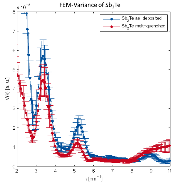
Figure 40: Shown are the corrected variance plots in relation to the scattering vector k of as deposited and melt quenched \text{Sb}_2\text{Te} . Both graph are now comparable and without an offset.
