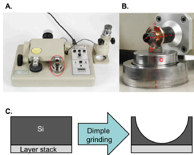
Figure 45: (A) A dimple grinder from Gatan is used to thin a sample mounted in the region marked by a red frame. (B) In closer view of the thinning process in the framed region it can be seen that the wheel (a) spins on top of the disc (b) which is mounted to a rotating table (c). The rotation axes are marked red. (C) The schematic drawing shows the part of the sample that got thinned away by the grinding process.
