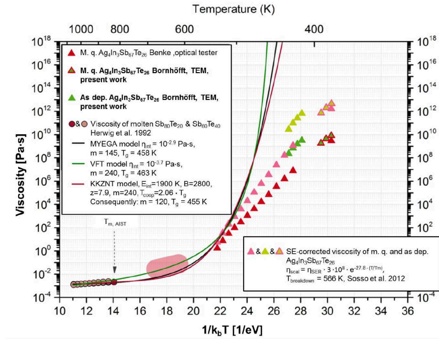
Figure 90: Shown are the calculated viscosities for as deposited and melt quenched AIST from the data of the optical tester, TEM and Kalb's AFM measurement (Kalb, 2006; Benke, 2017). Also shown are the calculated viscosity curves of AIST as a super cooled liquid on the basis of three different theoretical models. Image reprinted and amended with permission from the thesis of J. Benke (Benke, 2017).
