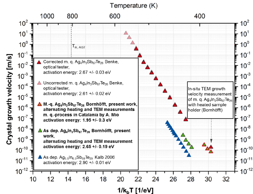
Figure 89: Shown are measured and calculated growth velocities of as deposited and melt quenched AIST performed by different methods in comparison (Kalb, 2006; Bornhöfft, 2012; Kaldenbach, 2012; Benke, 2017). Image reprinted and amended with permission from the thesis of J. Benke (Benke, 2017).
