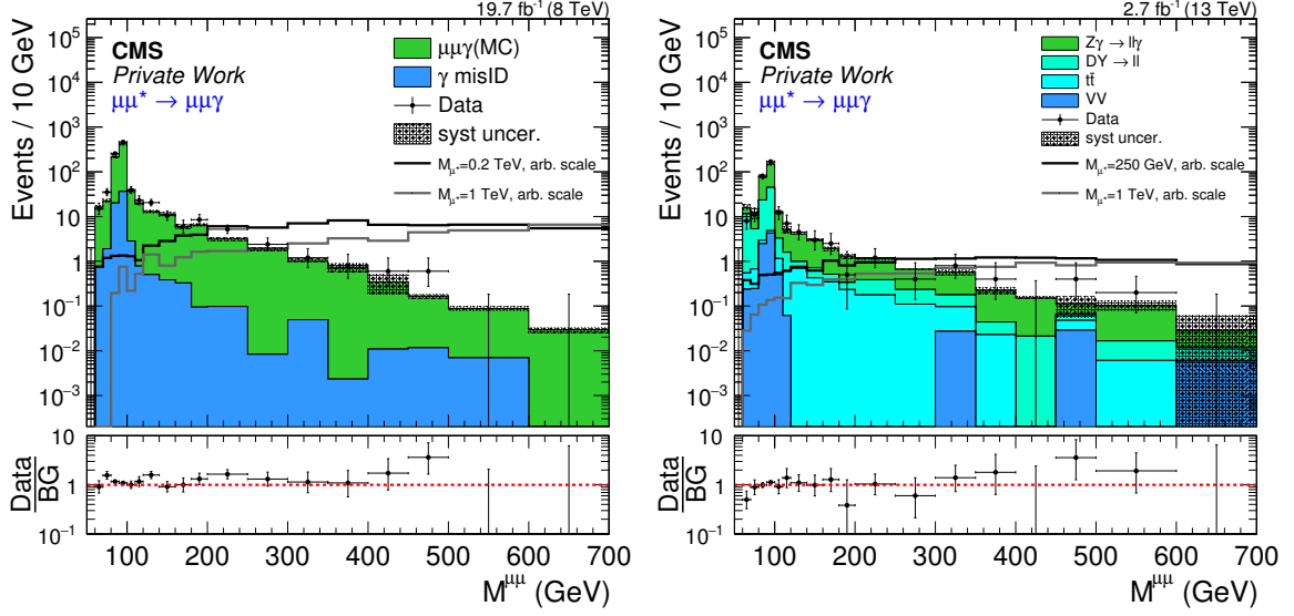
Figure 5.8: Distributions of the dimuon invariant mass M^{\mu\mu} in both analyses.
