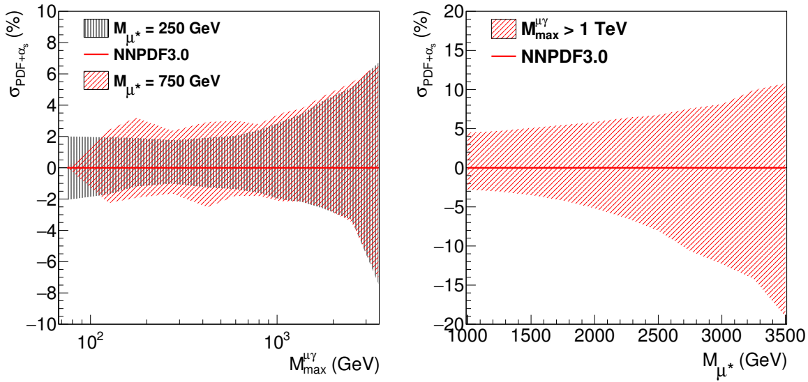
Figure 6.10: Left: PDF+ \alpha_s -uncertainties as a function of M_{\mu^*}^{\mu\gamma} for two signal samples with masses of 250 GeV and 750 GeV. Right: Evolution of PDF+ \alpha_s -uncertainties as a function of M_{\mu^*} , evaluated for masses M_{\mu^*}^{\mu\gamma} > 1 TeV.
