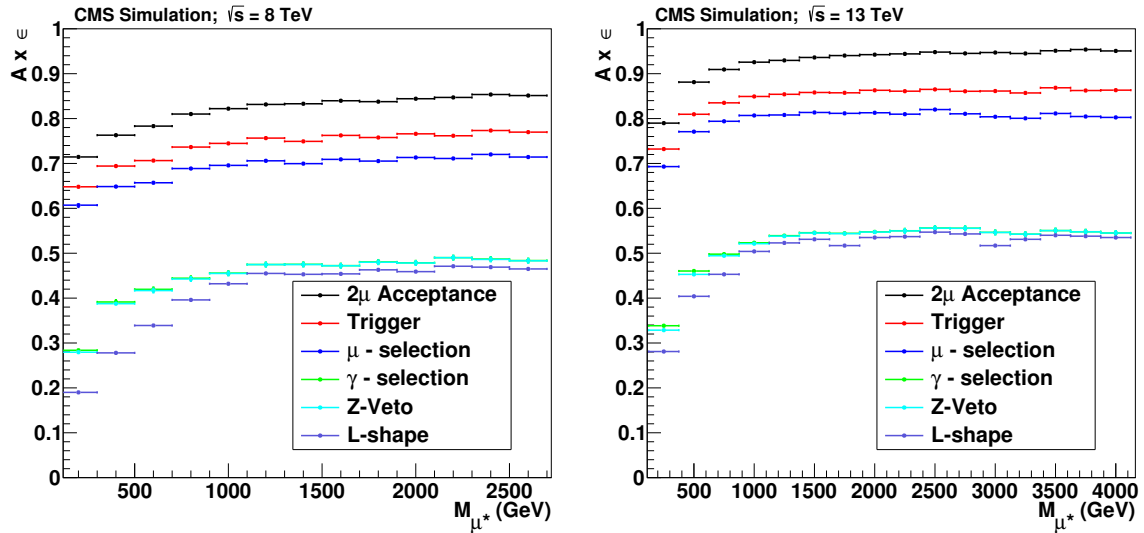
Figure 6.7: Overall signal selection efficiency after various selections for both analyses (analysis level, after reconstruction): After selecting two reconstructed muons within the acceptance, the requirement of the trigger, after applying the quality cuts on both muons, after selecting an additional photon with the respective ID, the negligible impact of the Z-veto, and after the final L-shape selection.
