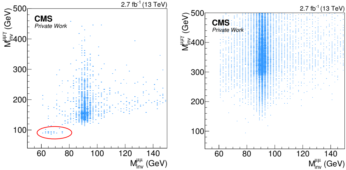
Figure 5.4: Two-dimensional distributions of the dimuon- and dimuon+photon invariant masses. The left plot shows the result from the inclusive sample of table 5.1, while the one on the right is derived from the sample with E_T^\gamma > 130 GeV. The red circle indicates the region where events with FSR-photons are expected to cluster. The events in both plots are not weighted to cross section and luminosity, the total scale of the distributions is in arbitrary units.
