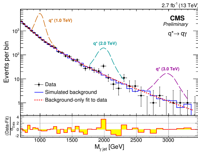
Figure 2.21: Spectrum of the \gamma -jet invariant mass from the search for excited quarks at \sqrt{s} = 13 TeV, as published by the CMS Collaboration in [46].
