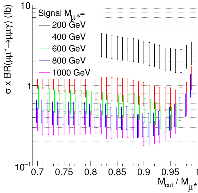
Figure 6.4: L-shape width optimization: Expected excluded signal cross section times branching ratio of different signal masses, as a function of the lower edge of the search region (compare text).
