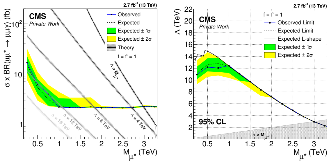
Figure 6.23: Cross section- and \Lambda -limits as derived from the three-body invariant mass, M^{\mu\mu\gamma} .
