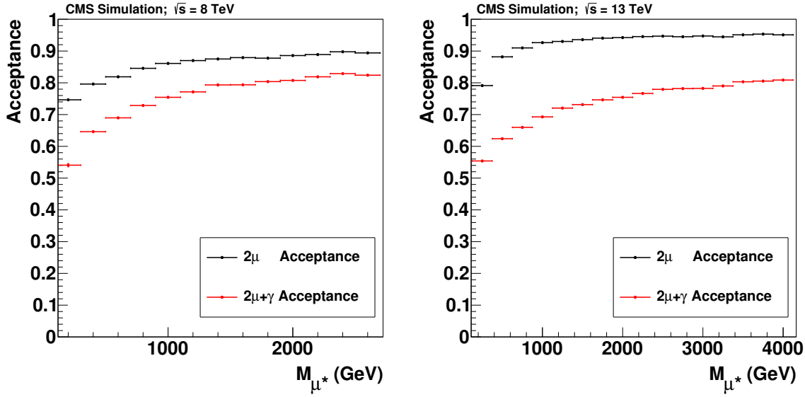
Figure 4.9: Relative amount of signal events, where two muons (black) and a photon (red) fulfill the kinematic requirements ( p_T^\mu/et^\gamma and \eta ) on generator level, depending on M_{\mu^*} .
