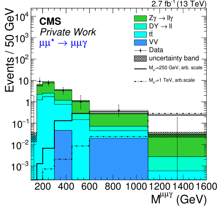
Figure 6.22: Distribution of the three-body invariant mass, M^{\mu\mu\gamma} , after all selections, including the Z-veto.
