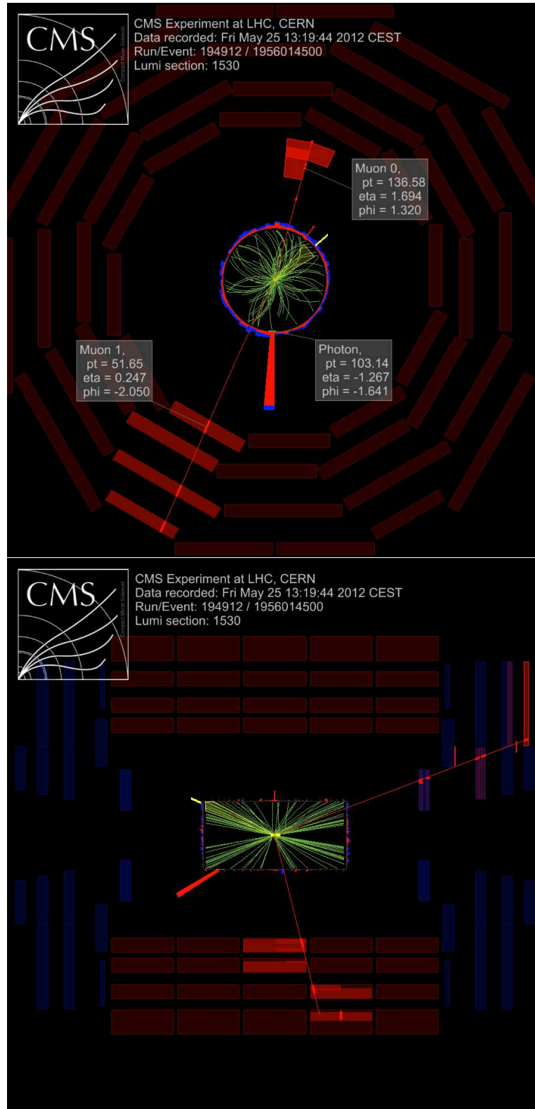
Figure 6.24: Event display of the \mu\mu\gamma -event with the highest maximum invariant mass ( M_{\max}^{\mu\gamma} = 548.3 \text{ GeV} ) as found in the Run I analysis, after applying all selections, including the Z-veto.
