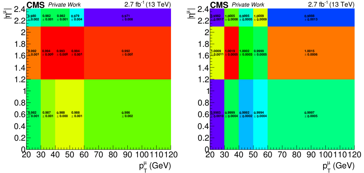
Figure B.4: Scalefactors for the High- p_T muon ID (left) and the relative tracker isolation for muons (right) as they are applied in Run II analyses. Additional systematic uncertainties of 1% for the ID and 0.5% for the isolation are applied [89].
