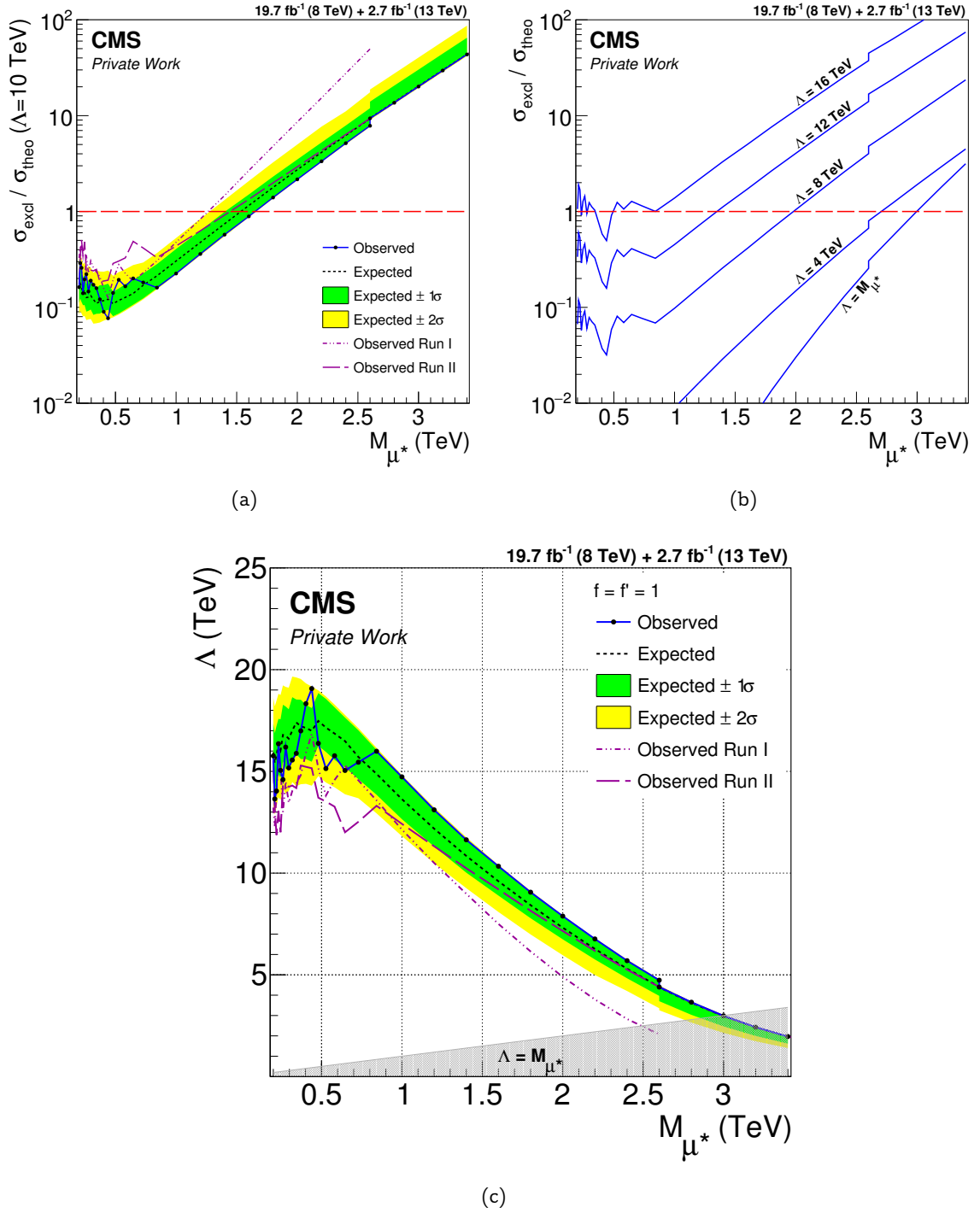
Figure 6.13: Combination of Run I and Run II results: (a) Ratio of the excluded cross section to the theoretical cross section with \Lambda = 10 \text{ TeV} . (b) Ratios of combined observed excluded cross sections to theoretical cross sections of different values of \Lambda . (c) Combined limit in the \Lambda - M_{\mu^*} -plane.
