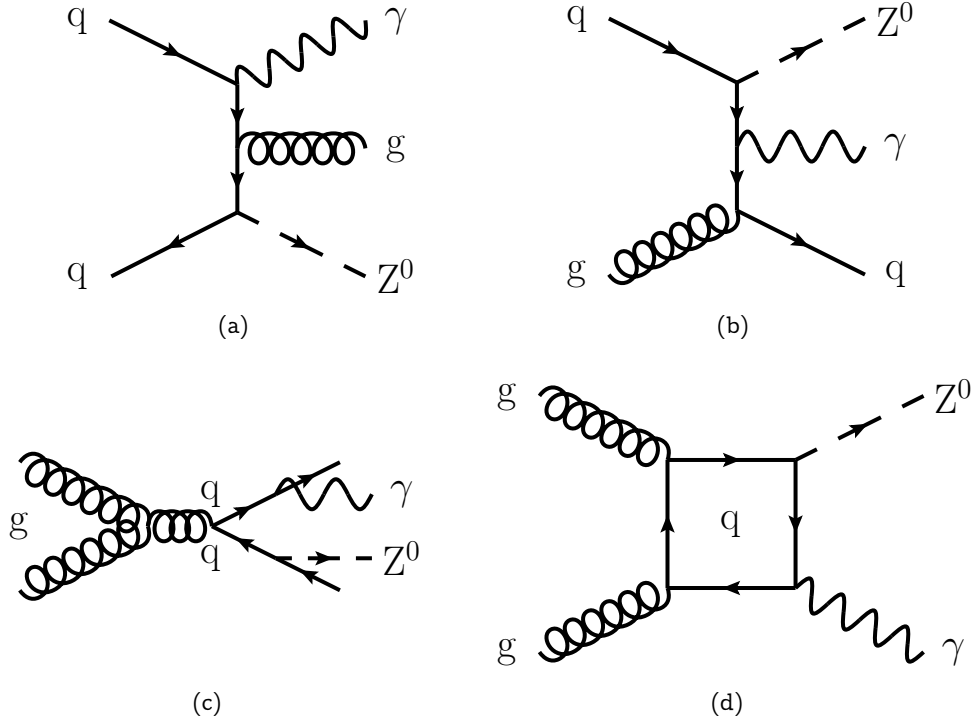
Figure 5.5: NLO (a,b) and NNLO (c,d) corrections to the Z\gamma -process.
