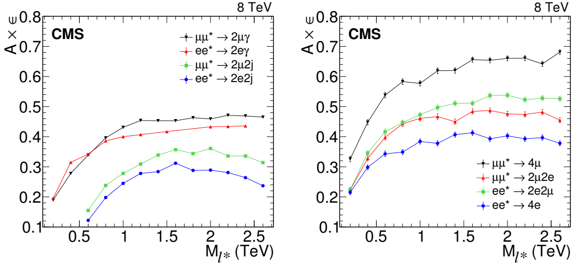
Figure 6.16: Signal acceptance times efficiency after all analysis requirements, including the final L-shape selection as a function of M_{l^*} for the different \ell\ell\gamma - and \ell\ell jj -channel on the left, and the 4\ell -channels on the right. Previously published in [3].
