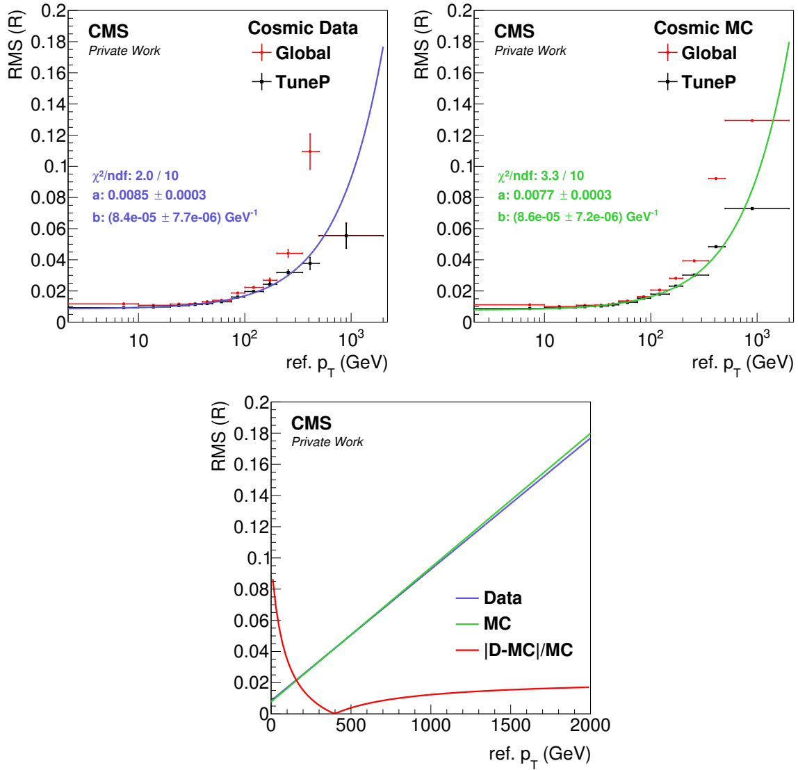
Figure 4.6: Upper two: RMS of the distributions of the residual R , as a function of the reference p_T from cosmic muon data (left) and MC (right) and for the global muon (red) and the TuneP reconstruction (black). Linear functions are fitted to the latter. Below: The results from the fits to Data and MC, as well as their relative difference.
