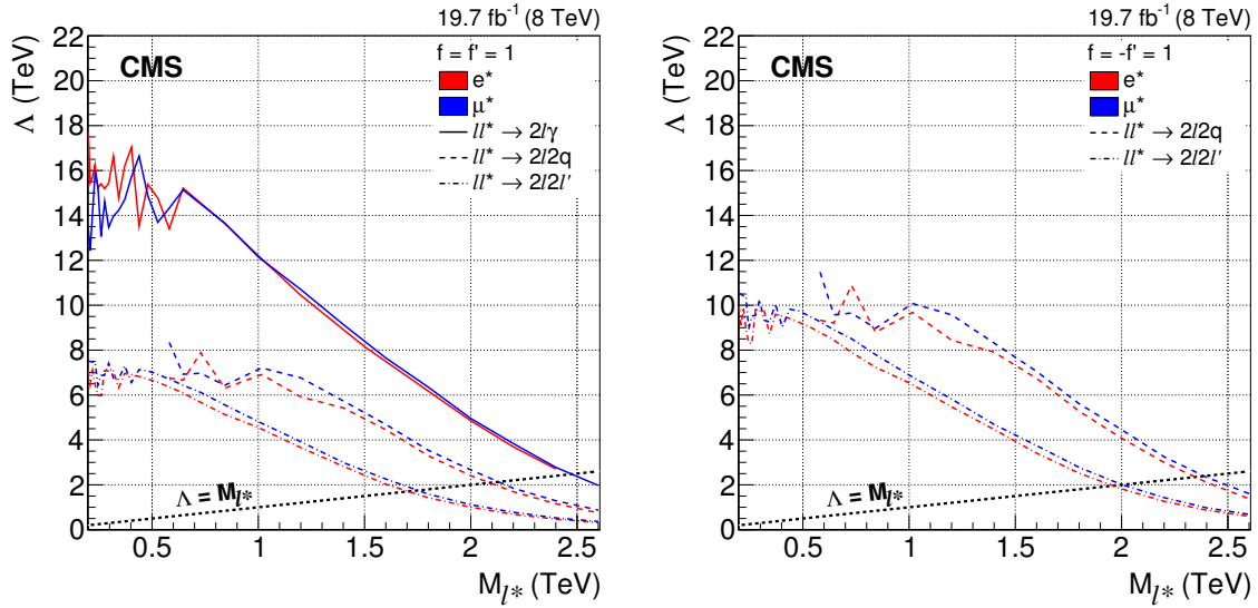
Figure 6.20: Limits on the compositeness scale \Lambda of all considered channels for the case f = f' = 1 (left) and f = -f' = 1 (right). In the latter case, the photon channels are suppressed. Limits of 4l -channels belonging to the same excited lepton flavor are combined. Previously published in [3].
