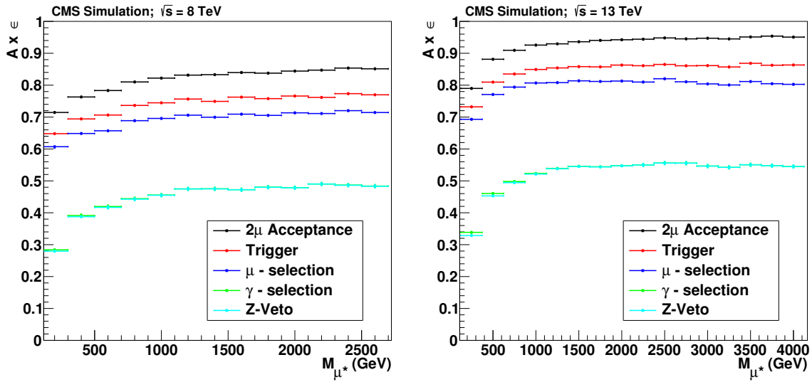
Figure 5.17: Total signal selection efficiency after various requirements on analysis level (after reconstruction) for both analyses: After selecting two reconstructed muons within the kinematic range, the requirement of the trigger, after applying the quality cuts on both muons, after selecting an additional photon with the respective ID, and the negligible impact of the Z-veto.
