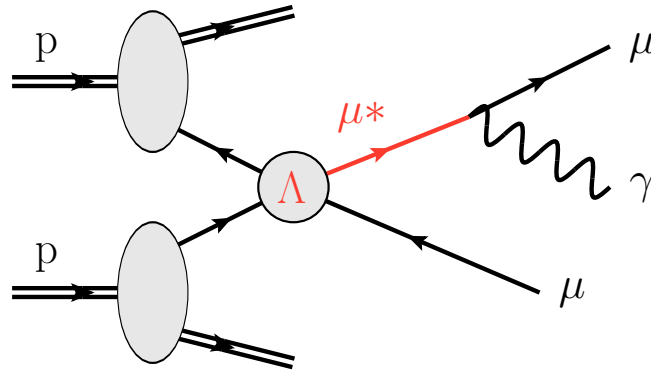
Figure 2.6: The relevant Feynman diagram for the analyses being presented in this thesis: Associated \mu^*\mu -production by four-fermion contact interaction with decay via photon radiation, leading to a \mu\mu\gamma -final state.
