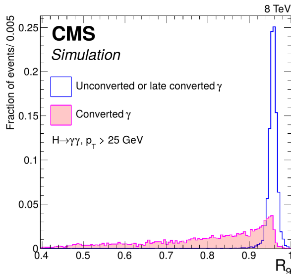
Figure 4.7: R_9 -distributions of converted and (almost) unconverted photons. Both are from simulation only. Taken from [62].
