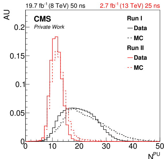
Figure 5.1: Number of pileup interactions as measured in data (solid lines) and as simulated in MC (dashed lines) for Run I (black) and Run II (red). All distributions are scaled to unit area.
