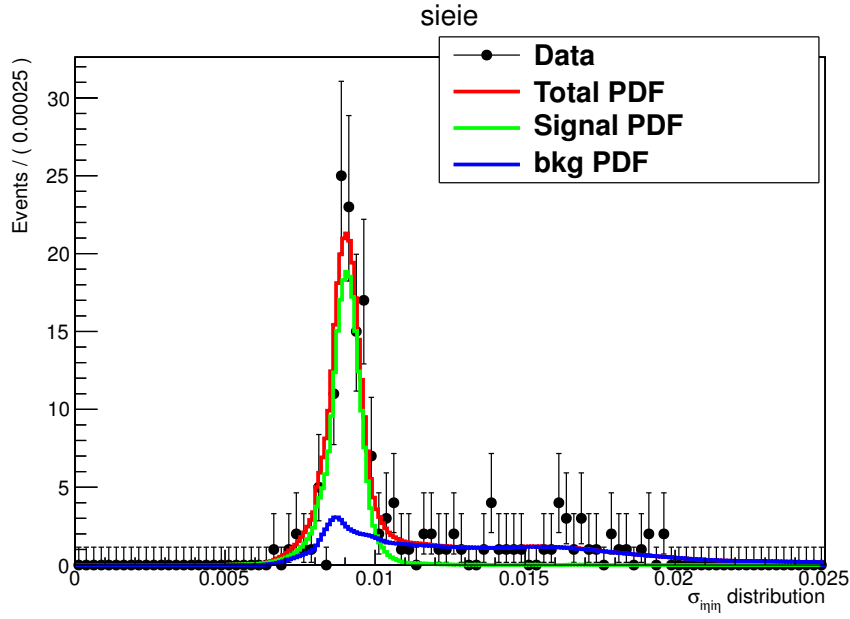
Figure 5.10: Template fit in the bin 35 \text{ GeV} < E_T^\gamma < 50 \text{ GeV} . Data are the black points, the signal of prompt photons (green) is estimated from MC. The background (blue) is from non-prompt photons estimated from a sideband of the charged hadron isolation. Taken from [132].
