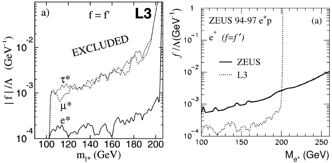
Figure 2.18: Left: Limits on excited charged leptons for the case f = f' , as obtained by L3 [37]. Right: Limit on e^* as obtained by ZEUS with a comparison to the L3-limit of the left figure [39].
