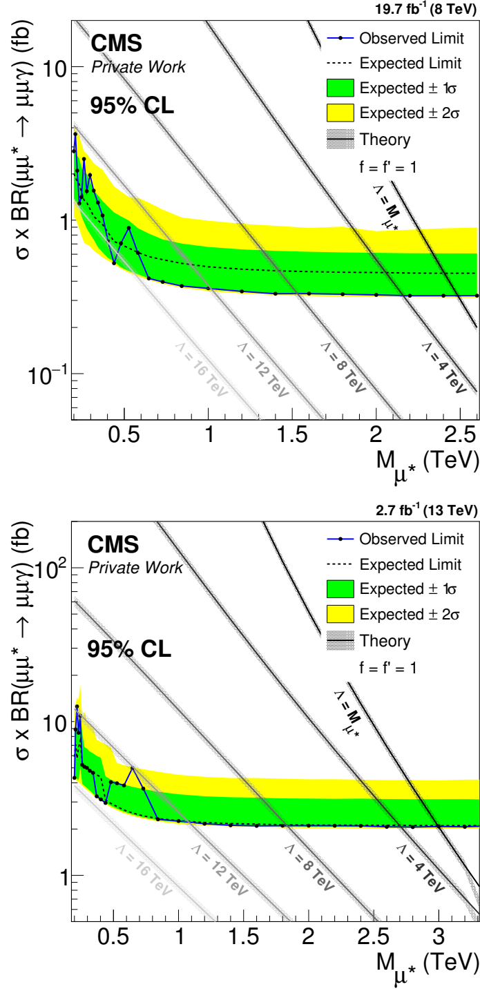
Figure 6.11: Limits on the signal cross section times branching ratio, at 95% CL, as a function of the excited lepton mass, M_{\mu^*} , as obtained from the Run I (upper plot) and Run II (lower plot) analyses. Median expected limits are given by a dashed black line, surrounded by the one- and two sigma bands in green and yellow, respectively. Observed limits have a solid blue line with black dots at the considered masses. Theory cross sections are shown for different values of \Lambda with the assigned 10% cross section uncertainty.
