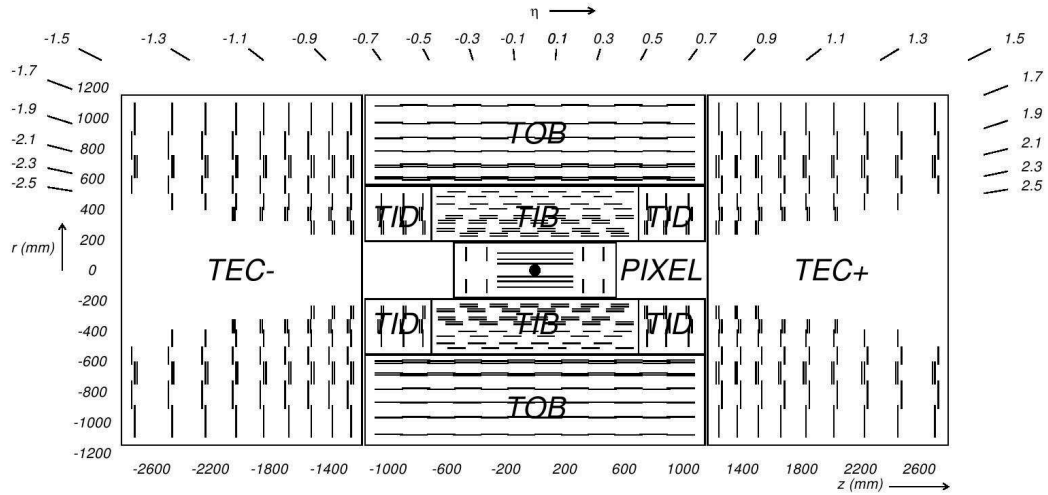
Figure 3.3: The CMS tracking system [52].
