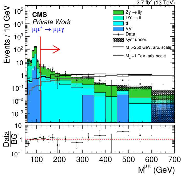
Figure 5.15: Invariant dimuon mass distribution of the Run II analysis showing the Z-veto, which is the requirement of M^{\mu\mu} > M^Z + 25 GeV. Only events in the region marked by the red arrow are considered for further analysis.
