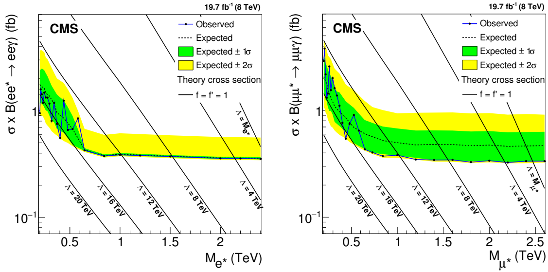
Figure 6.17: Cross section limit of the ee\gamma - (left) and \mu\mu\gamma - (right) channel. Previously published in [3].
