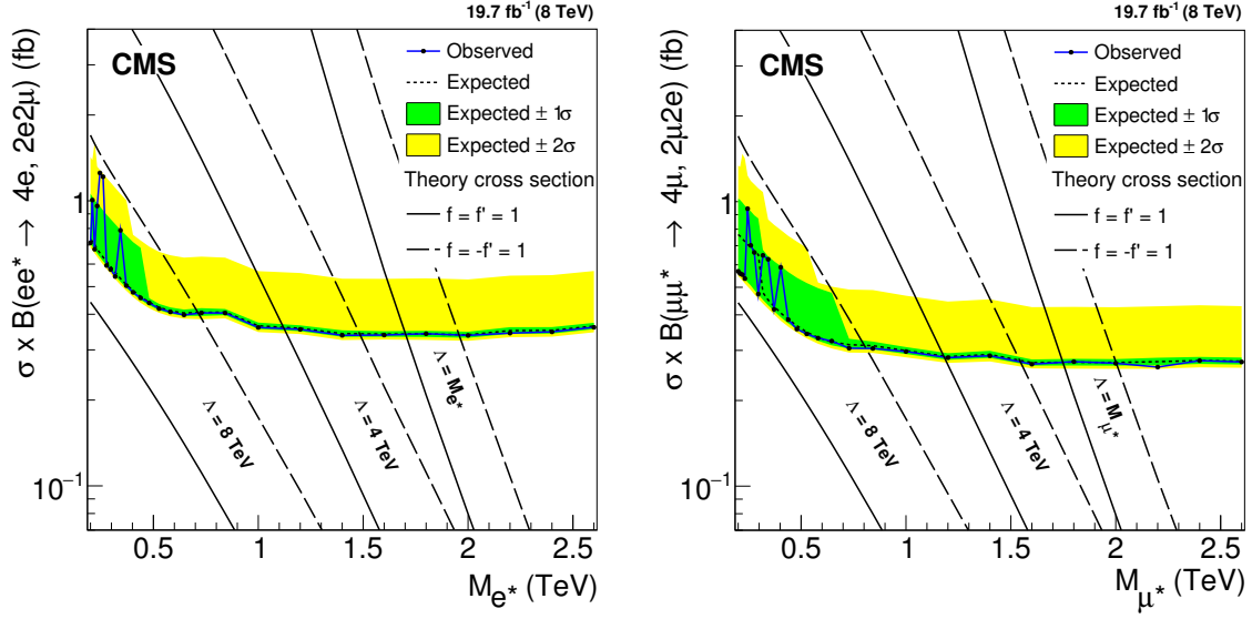
Figure 6.19: Cross section limit of the 2e2l - (left) and 2\mu2l - (right) channel. Previously published in [3].
