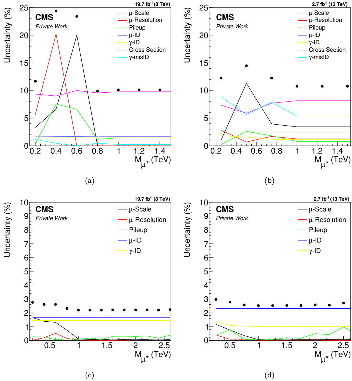
Figure 6.8: Impact of the systematic uncertainties on various search regions as determined for the background (upper two) and various signal samples (lower two) and for the Run I (left two) and Run II (right two) analysis. Black points represent the quadratic sum of all contributions.
