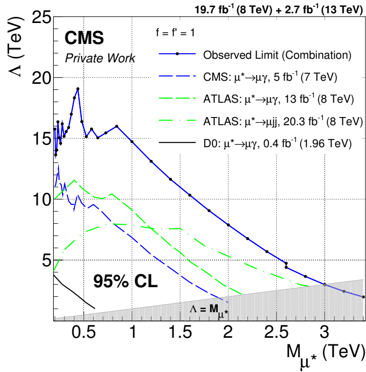
Figure 6.14: Comparison of the combined observed limit as obtained in this thesis (blue with black dots) with a selection of existing results. Blue lines indicate limits from CMS, green from the ATLAS Collaboration. Observed limits obtained from various final states, integrated luminosities, and center of mass energies are compared.
