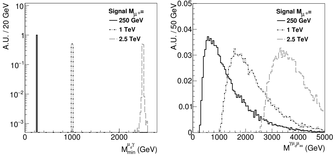
Figure 2.15: Invariant masses of the photon and \mu_d (left) and three-body invariant masses (right), as obtained from signal simulation on generator level.
