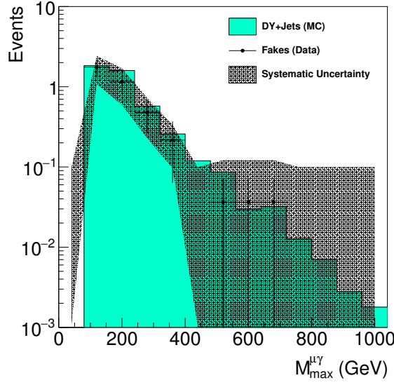
Figure 5.13: Comparison of the data driven description of backgrounds with a faked photon (black dots) with the simulated Drell-Yan background (colored area). The hatched area represents the systematic uncertainty on the fake prediction from data. Empty bins have an assigned systematic uncertainty of 0.1 events.
