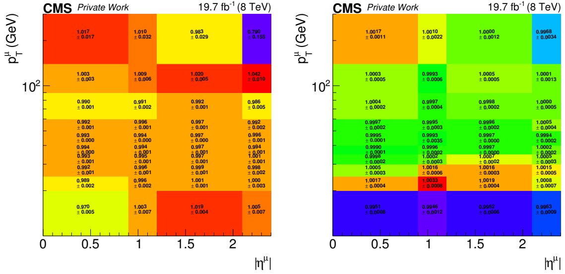
Figure B.1: Scalefactors for the High- p_T muon ID (left) and the relative tracker isolation for muons (right) as they are applied in Run I analyses [88].
