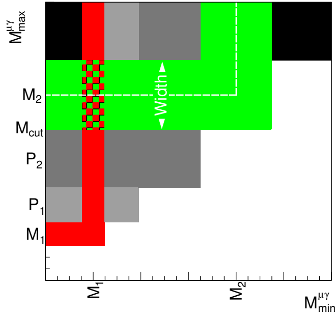
Figure 6.3: Scheme of the L-shape selection. Two windows that are optimized with signal MC at masses M_1 and M_2 are outlined in red and green. Additional interpolated windows at positions P_1 and P_2 are shown in gray.
