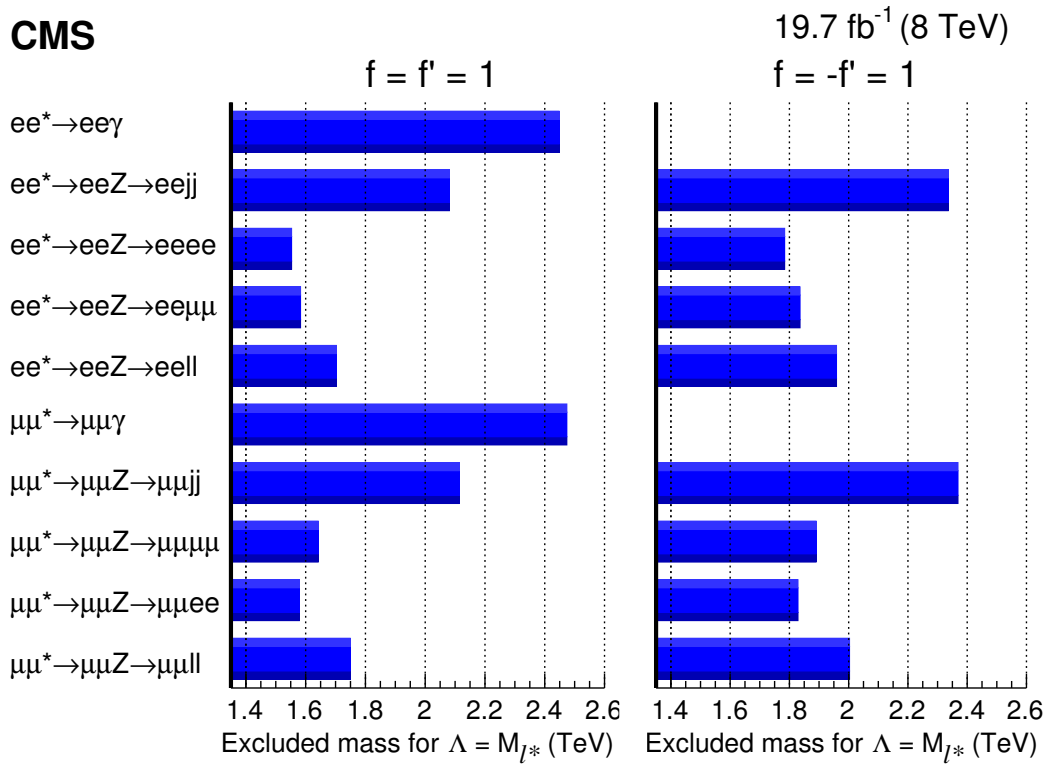
Figure 6.21: Summary of all limits on the compositeness scale \Lambda in the case \Lambda = M_{l^*} for f = f' = 1 and f = -f' = 1 . In the latter case, the photon channels are suppressed. Previously published in [3].
