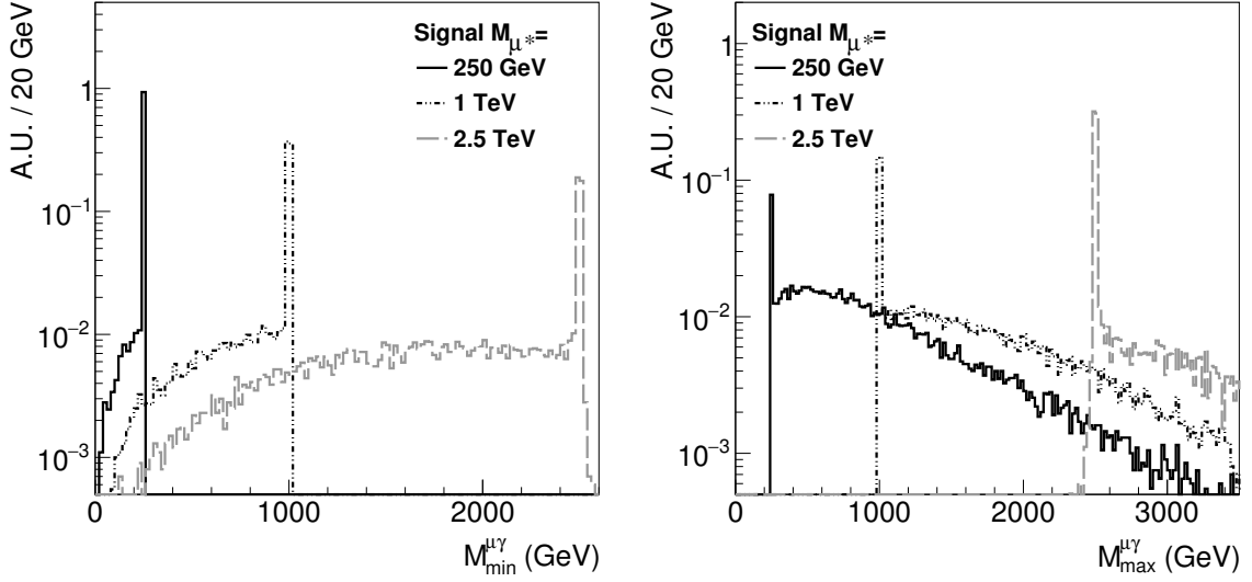
Figure 2.16: Minimum (left) and maximum (right) invariant muon-photon masses, denoted as M_{\min}^{\mu\gamma} & M_{\max}^{\mu\gamma} , as obtained from signal simulation on generator level.
