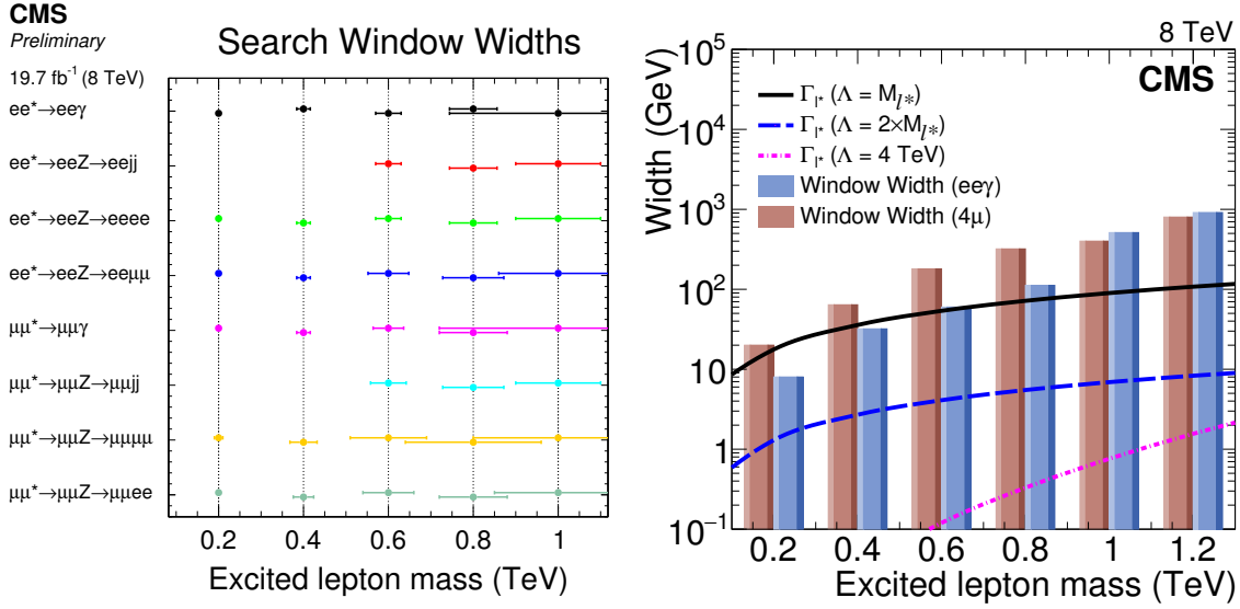
Figure 6.15: Left: Summary of the optimized search window widths of all considered channels. Previously published in [2]. Right: Comparison of the intrinsic excited lepton width at different values of \Lambda with the search window widths of two different channels. Previously published in [3].
