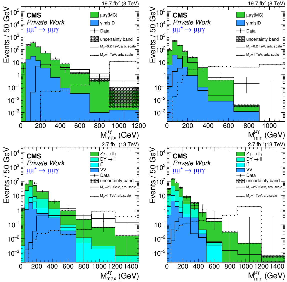
Figure 5.14: Distributions of the masses M_{\max}^{\mu\gamma} (left) and M_{\min}^{\mu\gamma} (right) of the Run I (top) and Run II (bottom) analyses after the selection of two muons and one photon.
