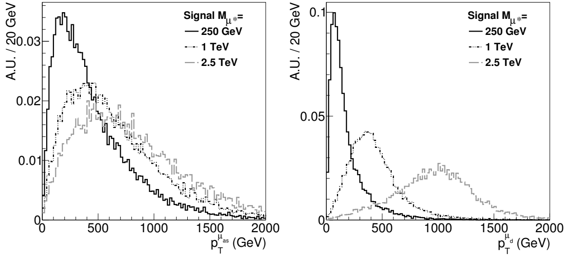
Figure 2.11: Transverse momenta of the muon from the associated production ( \mu_{as} , left) and the \mu^* -decay ( \mu_d , right), as obtained from signal simulation on generator level.
