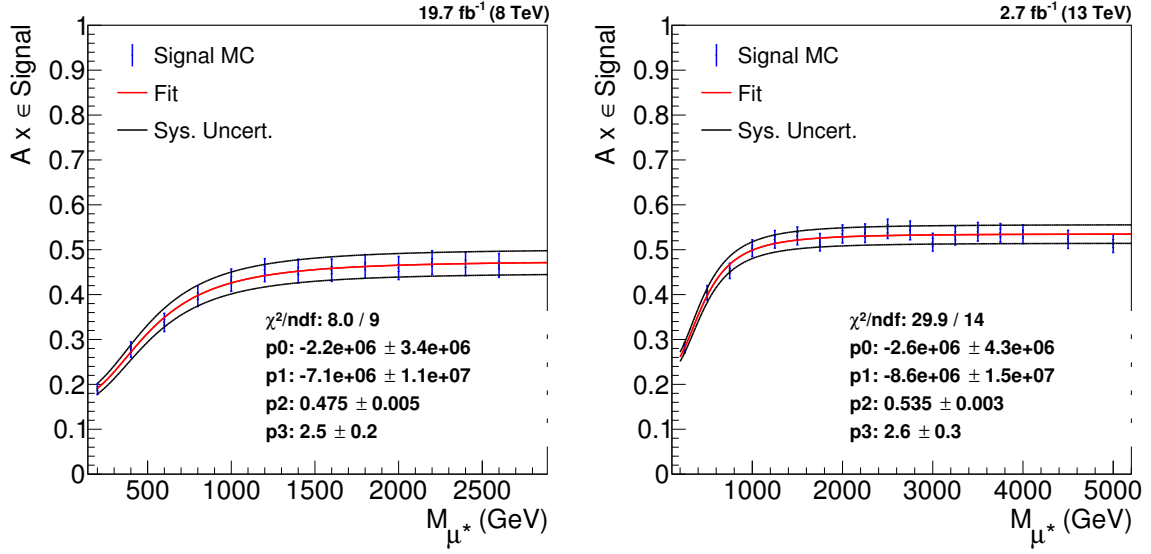
Figure 6.6: Fit to the signal efficiencies for both analyses: Signal efficiency after all cuts, including the final L-shape selection and with systematic uncertainties in blue. Fit to the efficiency as a red line, shifted fit to account for systematic uncertainties in black.
