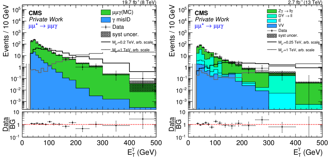
Figure 4.8: Distributions of E_T^\gamma for Run I (left) with the cut-based photon identification, and Run II (right) using the MVA-identification. Both plots show distributions after the selection of two muons and a photon. The Run I distribution on the left includes a data-derived background contribution, shown in blue.
