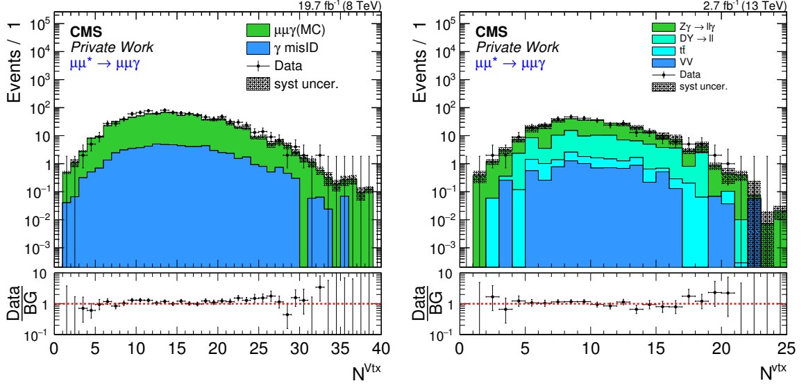
Figure 5.2: Number of reconstructed vertices per event for Run I (left) and Run II (right) with the corresponding systematic uncertainty.
