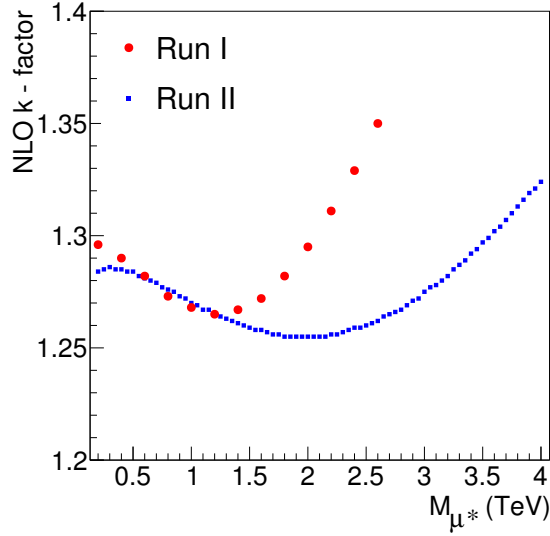
Figure 2.8: NLO k-factors as a function of M_{\mu^*} for \sqrt{s} = 8 TeV (red points) and \sqrt{s} = 13 TeV (blue squares). The exact numbers were provided by the author of [32].
