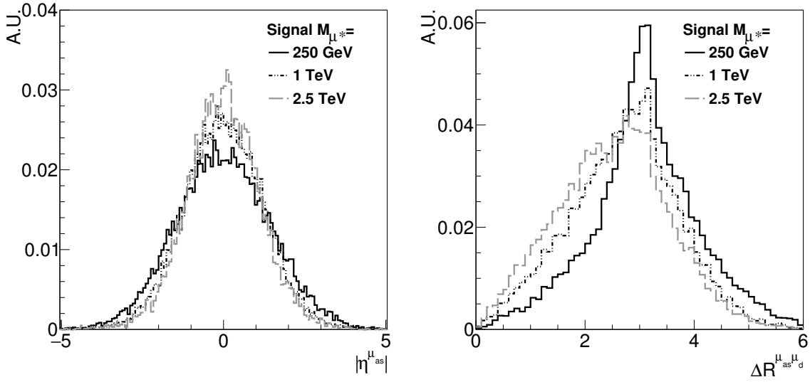
Figure 2.12: Left: \eta -distributions of the muon from the associated production, \mu_{as} . Right: Angle \Delta R between both muons. Both are obtained from signal simulation on generator level.
