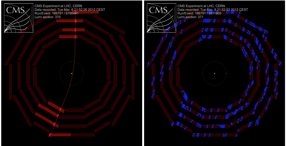
Figure 4.3: Events with cosmic muons in the r - \phi plane of the detector. Left: A single muon traversing the detector with visible bending from the magnetic field that can be used for momentum resolution studies. Right: A shower of cosmic muons. Fascinating, but rather useless for analysis purposes.
