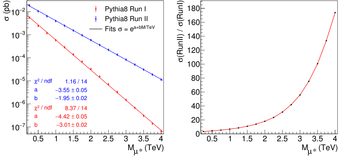
Figure 2.7: Left: Cross sections for the process q\bar{q} \rightarrow \mu\mu^* \rightarrow \mu\mu\gamma as a function of M_{\mu^*} for \sqrt{s} = 8 TeV (red) and \sqrt{s} = 13 TeV (blue), calculated with Pythia8.205. An exponential function is fitted to both in order to be able to evaluate the cross section at any given mass. An uncertainty of 10% is assigned to the cross sections. Right: Ratio between both. Both plots are for \Lambda = 10 TeV.
