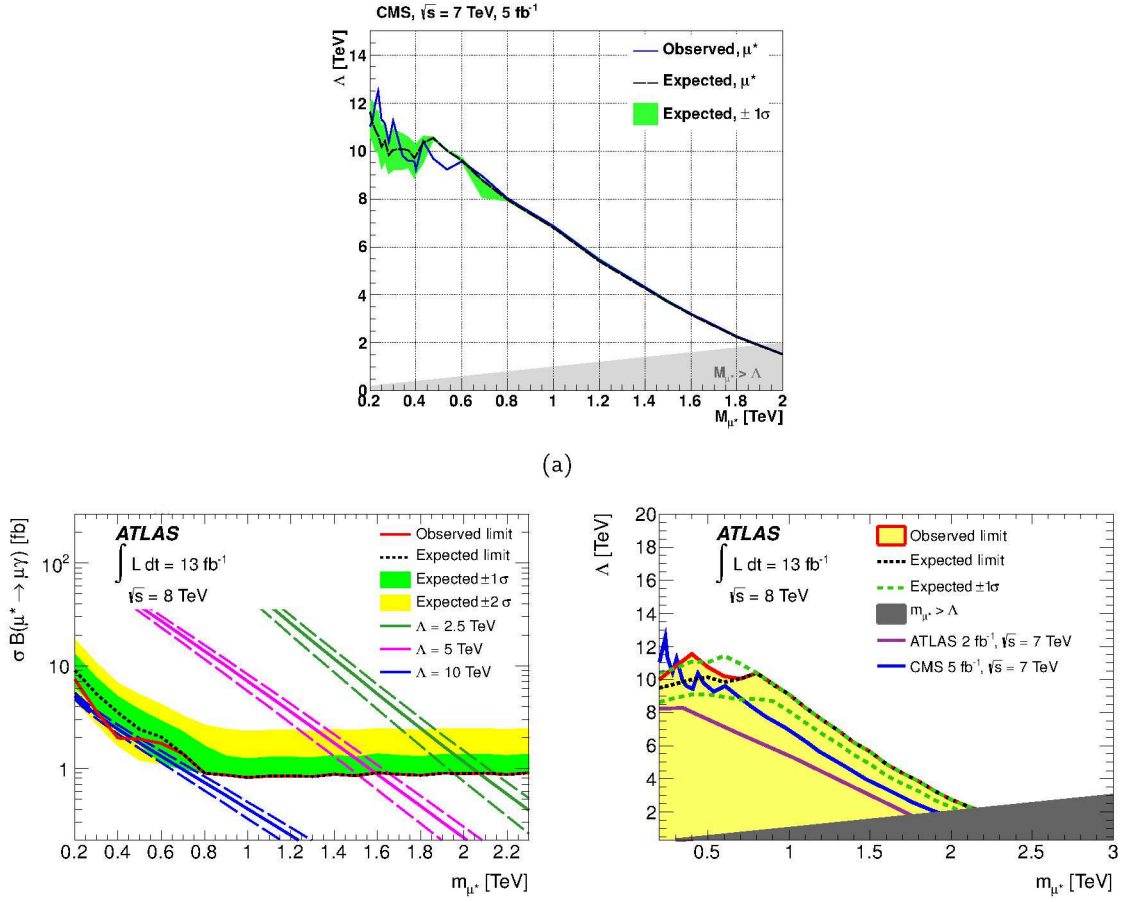
Figure 2.19: Limits on q\bar{q} \rightarrow \mu\mu^* \rightarrow \mu\mu\gamma : Upper figure: Excluded \Lambda - M_{\mu^*} values of the 7 TeV CMS analysis [43]. Lower plots: Cross section (left) and \Lambda (right) limit of the 8 TeV ATLAS \mu^* analysis [44].
