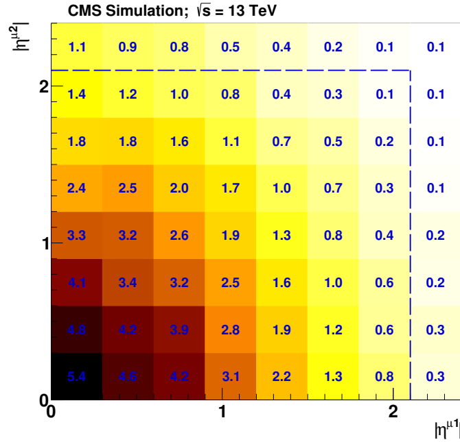
Figure 4.10: Two dimensional distribution of \eta of two muons at generator level shown for a signal sample with M_{\mu^*} = 1 TeV and \sqrt{s} = 13 TeV. Color coding and numbers refer to the relative number of events in a respective tile, given in percent. The area outside the dashed line yields 5.4%.
