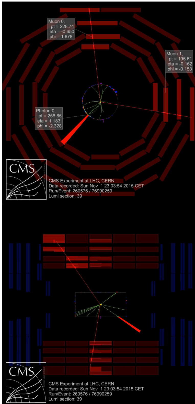
Figure 6.25: Event display of the \mu\mu\gamma -event with the highest maximum invariant mass ( M_{\max}^{\mu\gamma} = 672.8 \text{ GeV} ) as found in the Run II analysis, after applying all selections, including the Z-veto.
