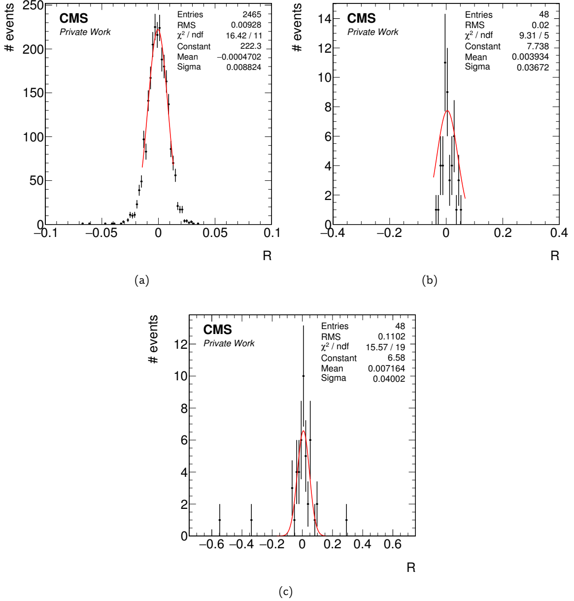
Figure 4.5: Distributions of the residual R (equation 4.3) in different bins of p_T with Gaussian fits. (a)&(b): TuneP reconstruction in the bins (0 < p_T < 10) GeV and (350 < p_T < 500) GeV. (c): Global muon reconstruction in the bin (350 < p_T < 500) GeV.
