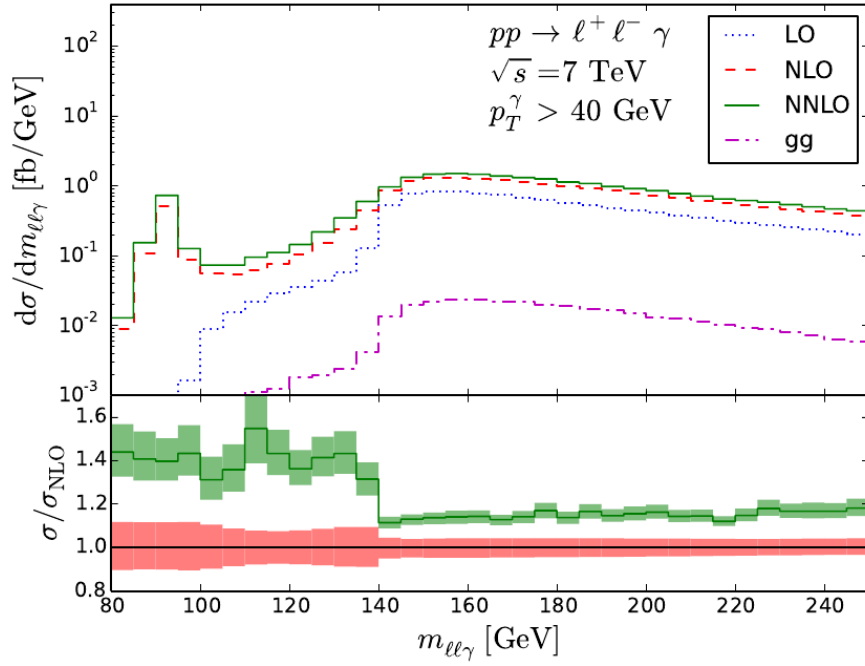
Figure 5.6: Distribution of the \ell\ell\gamma invariant mass with cross sections at LO (dotted blue), NLO (dashed red), NNLO (solid green), and loop processes from gg-fusion (purple) like in figure 5.5(d). The lower plot shows the ratio NNLO/NLO and the uncertainty of the NLO and NNLO predictions as colored bands. Taken from [123]. According to the reference, masses m_{\ell\ell\gamma} < 97 GeV are kinematically not accessible at LO. This changes when either the order in QCD is increased or the photon momentum is considerably lowered.
