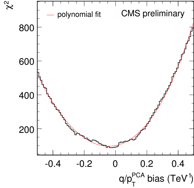
Figure 4.2: Example of a \chi^2 -distribution obtained from the cosmic endpoint method in [90]. The line is a polynomial function that was fitted to the data.
