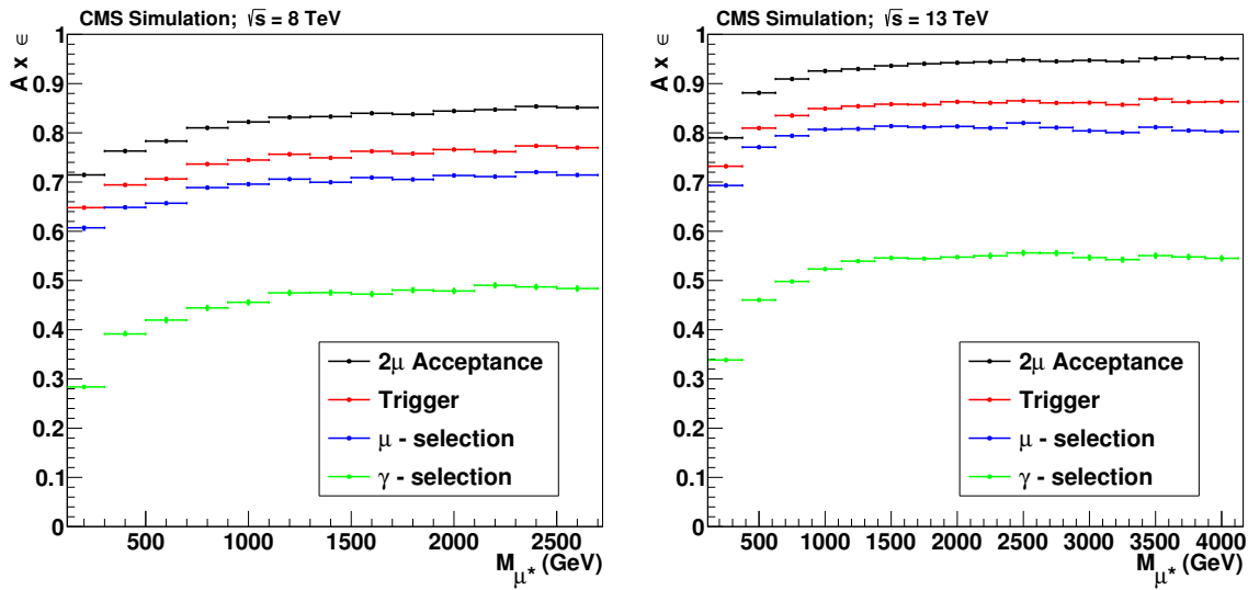
Figure 4.11: Overall selection efficiency as estimated from signal simulation after various requirements for both analyses (analysis level, after reconstruction): After selecting two reconstructed muons within the kinematic range (black), the requirement of the trigger (red), after applying the quality cuts on both muons (blue), and after selecting an additional photon with the respective ID (green).
