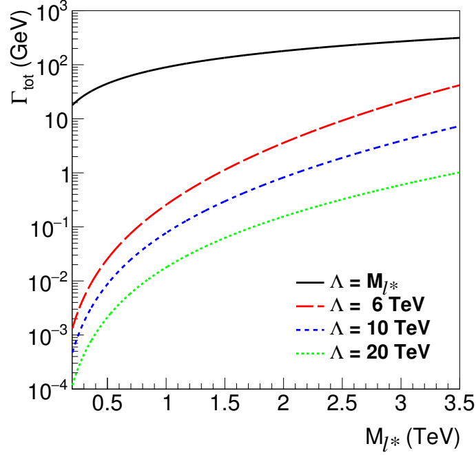
Figure 2.5: Total decay width of an excited lepton as a function of M_{l^*} and different values of \Lambda . The values are calculated as the sum of the partial widths from the photon, gauge-boson and CI-decays with f = f' = 1 .
