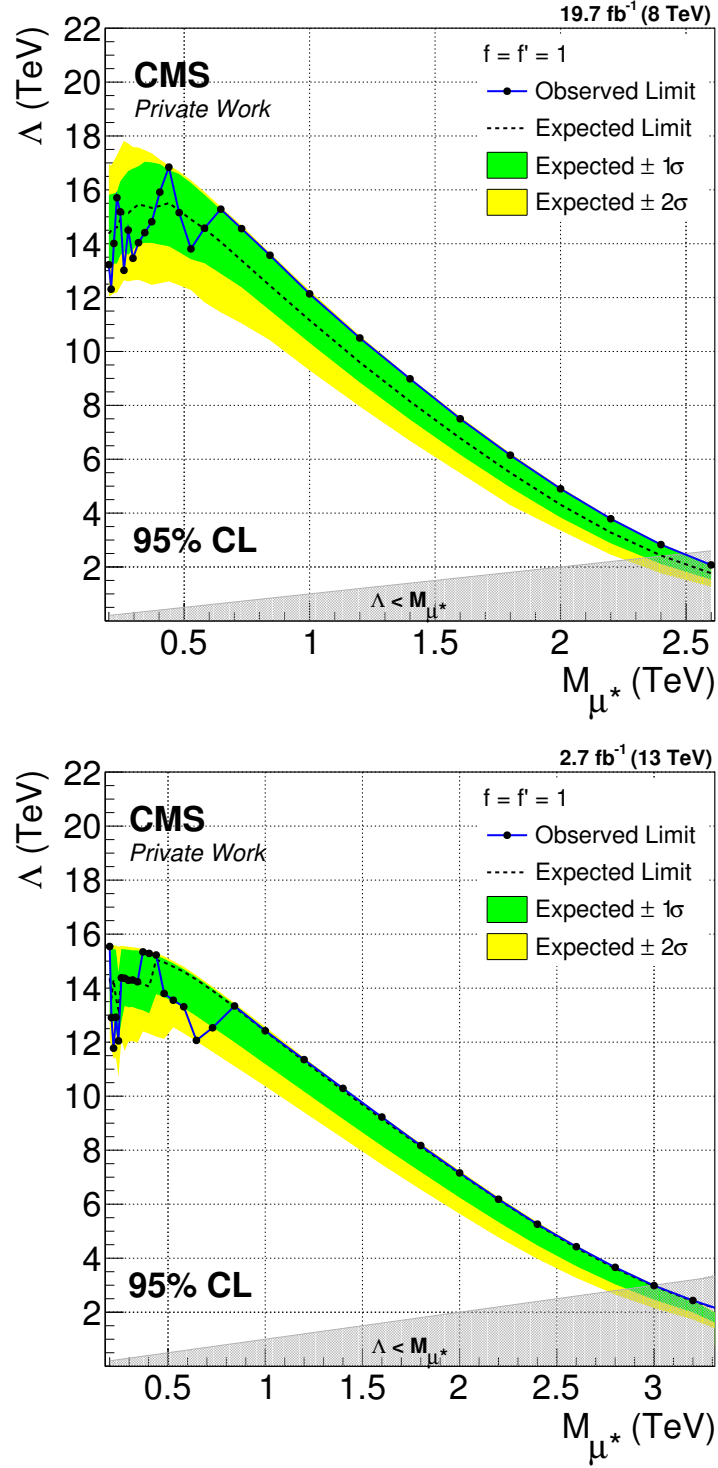
Figure 6.12: Limits on \Lambda , as a function of the excited lepton mass, M_{\mu^*} . Excluded values are below the curves. The gray regime indicates the theoretically forbidden area, where \Lambda < M_{\mu^*} .
