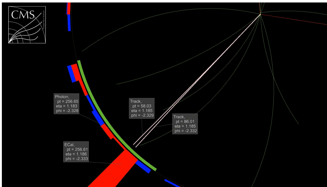
Figure 6.26: Detailed view into the transverse plane of the event from figure 6.25 with focus on the photon, its main ECal deposit, and the tracks pointing into the same direction.
