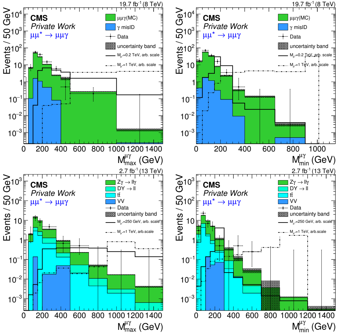
Figure 5.16: Distributions of the masses M_{\max}^{\mu\gamma} (left) and M_{\min}^{\mu\gamma} (right) of the Run I (top) and Run II (bottom) analyses after the selection of two muons and one photon, as well as the additional Z-veto.
