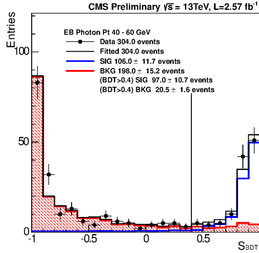
Figure 5.12: Output of the BDT score of preselected photons S_{\text{BDT}}^{\gamma} in the bin 40 \text{ GeV} < E_T^{\gamma} < 60 \text{ GeV} . Various contributions are shown. Black dots: Outcome from the data. Blue “Signal”: True photons estimated from a W\gamma -sample simulated with Pythia. Red “Background”: Contribution from faked photons, estimated from a W +Jets sample from data, where the lepton is used to tag the events. Black line: Fit of “SIG”+“BKG” to data. Adapted from [130].
