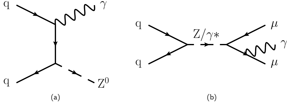
Figure 5.3: Feynman diagram of leading order Z\gamma production (a) and dimuon production by Drell-Yan with an additional photon from final state radiation (b).
