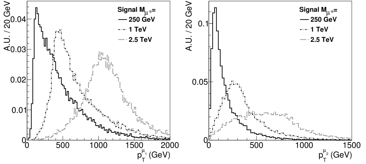
Figure 2.10: Distributions of the transverse momenta of the leading ( \mu_1 , left) and subleading ( \mu_2 , right) muon, as obtained from signal simulation on generator level.
