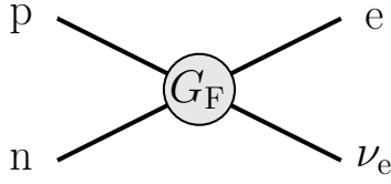
Figure 2.1: Fermi's interaction: Scheme of the \beta -decay, where all involved particles share one common vertex with the coupling strength G_F .
