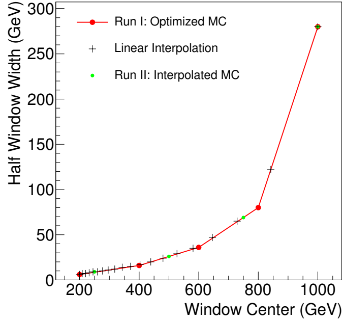
Figure 6.5: Interpolation of L-shaped search windows. Red dots: Widths optimized for the Run I MC samples. Black crosses: Linear interpolation of additional search windows. Green dots: Linear interpolation at the masses of the Run II MC samples.
