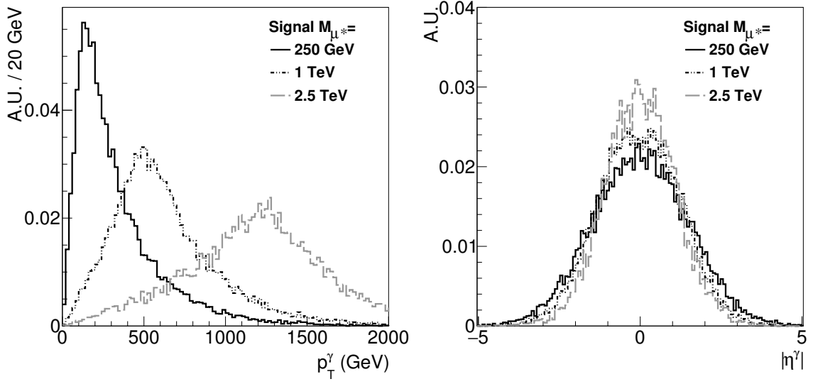
Figure 2.13: Left: Transverse momentum distributions from the photons originating from the \mu^* -decay. Right: The corresponding \eta -distributions. Both are obtained from signal simulation on generator level.
