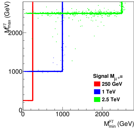
Figure 2.17: Two-dimensional M_{\min}^{\mu\gamma} - M_{\max}^{\mu\gamma} -distribution, as obtained from signal simulation on generator level.
