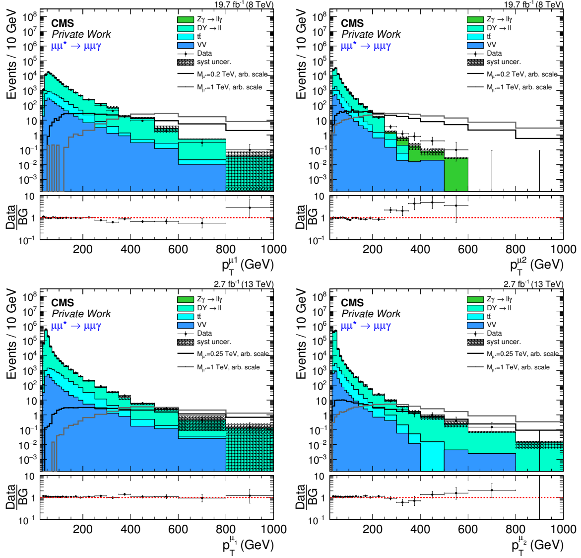
Figure 4.1: p_T -distributions of the leading (left) and subleading (right) muon as obtained in the Run I (top) and Run II (bottom) analyses. Backgrounds in all plots are determined from MC, exclusively. Due to low MC statistics, the backgrounds of the Run I plots stop at certain points in the spectra. As these backgrounds are replaced by a prediction from data later-on, this behavior is not further discussed here. Additionally, the expected signal behavior is given by two exemplary samples, outlined by solid lines. The Run II plots show the results after requiring M^{\mu\mu} > 60 GeV.
