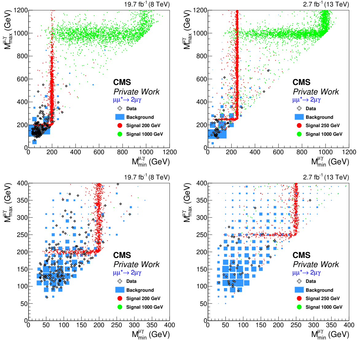
Figure 6.2: Two dimensional M_{\min}^{\mu\gamma} - M_{\max}^{\mu\gamma} -distributions after all cuts, including the Z-veto. Backgrounds are added up and shown in blue, various example signals are also presented. Their distributions show the typical “L-shapes”. For reasons of presentational style, the signal MC has not been weighted according to cross section or luminosity. The lower plots show a zoom into the low-mass region
