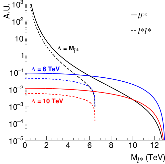
Figure 2.3: Partonic cross sections for the production of an excited lepton in association with an ordinary lepton (solid) and excited lepton pair-production (dashed), as a function of the excited lepton mass. The functional behavior for three different values of \Lambda is shown, assuming \sqrt{s} = 13 TeV.
