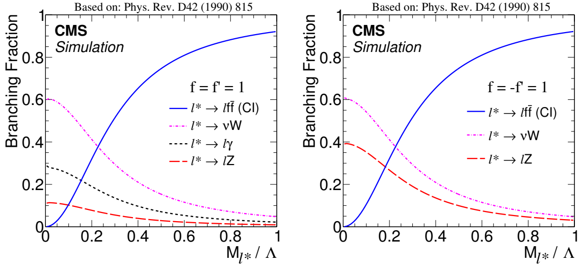
Figure 2.4: Branching ratios of the various \ell^* -decay modes as a function of M_{\ell^*}/\Lambda . Previously published in [3].
