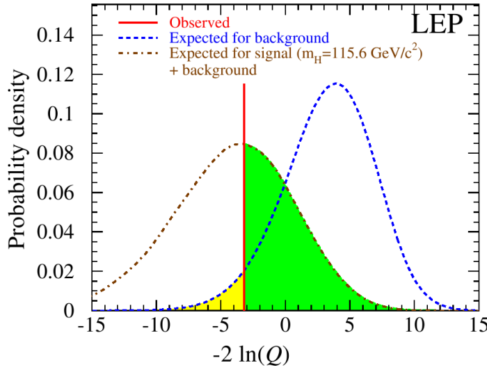
Figure 6.1: Distributions of the test statistic ( -2\ln(Q) ) for b (dashed blue), s+b (dashed-dotted), and the observation (solid red). Taken from [139].
