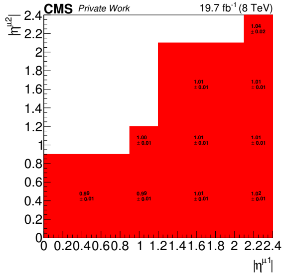
Figure B.2: Scalefactors for the di-muon trigger of the Run I analysis. An additional systematic uncertainty of 0.8% is applied [88].
