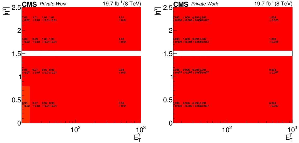
Figure B.3: For Run I, scalefactors are provided separately for the simple cut based photon ID, tight working point (left) and the conversion safe electron veto (right) [102].
