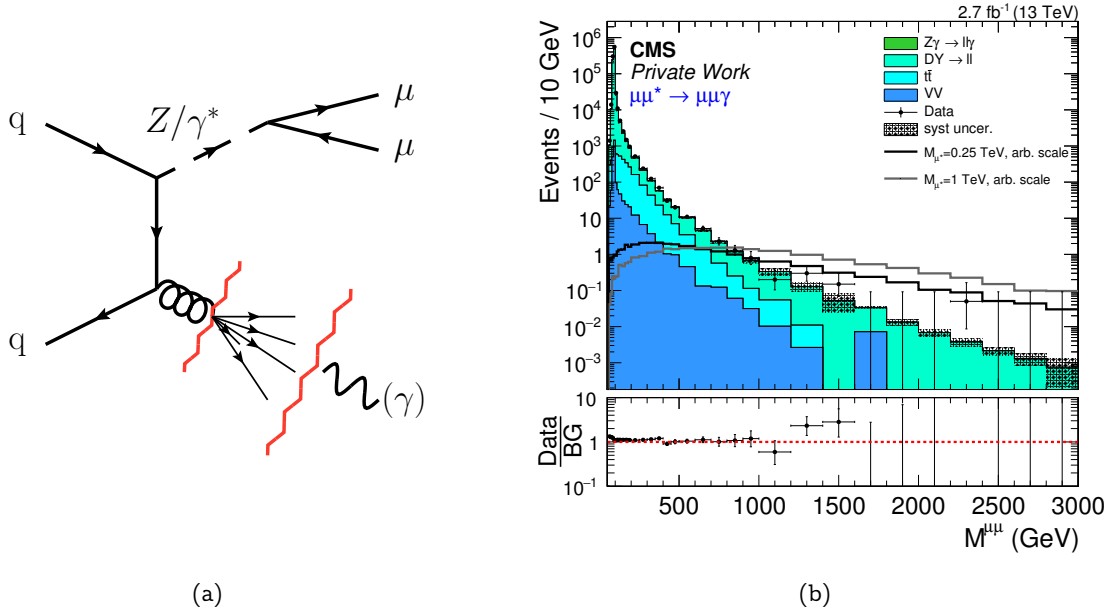
Figure 5.9: Left: Example Feynman diagram of the DY+Jets process where a jet is misidentified as a photon. Right: Dimuon invariant mass spectrum after selecting two muons. An additional photon is not required.
