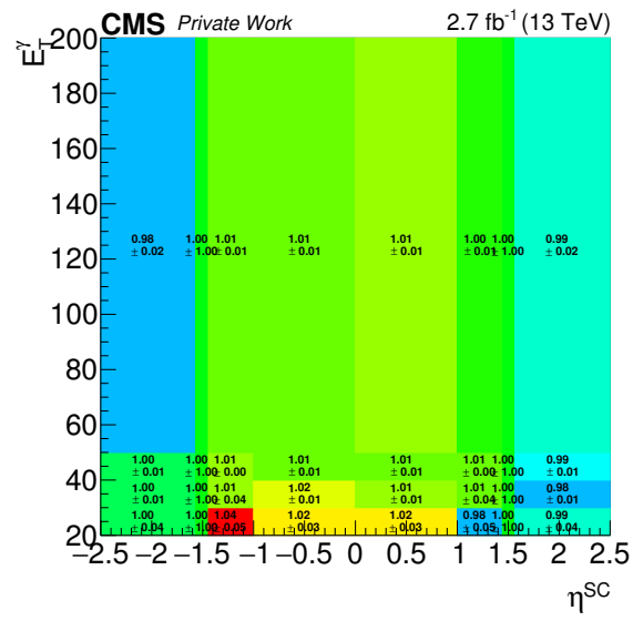
Figure B.5: Scalefactors for the MVA photon ID of Run II analyses [165].
