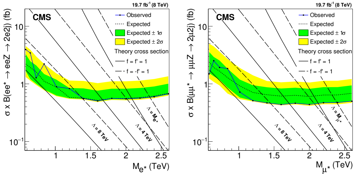
Figure 6.18: Cross section limit of the 2e2j - (left) and 2\mu2j - (right) channel. Previously published in [3].
