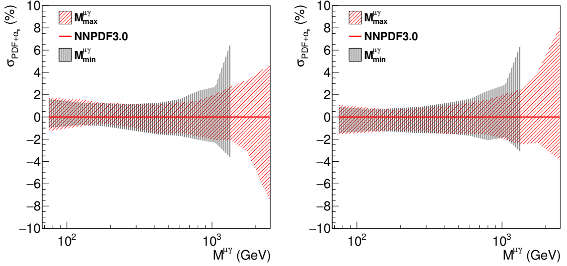
Figure 6.9: PDF+ \alpha_s -uncertainties evaluated for the M_{\min}^{\mu\gamma} (black) and M_{\max}^{\mu\gamma} (red) -distributions of the Z\gamma -background, after all selection without the final L-shape requirement. The plot on the left belongs to the reweighting of PDF-sets that are NLO in QCD, the right to NNLO.
