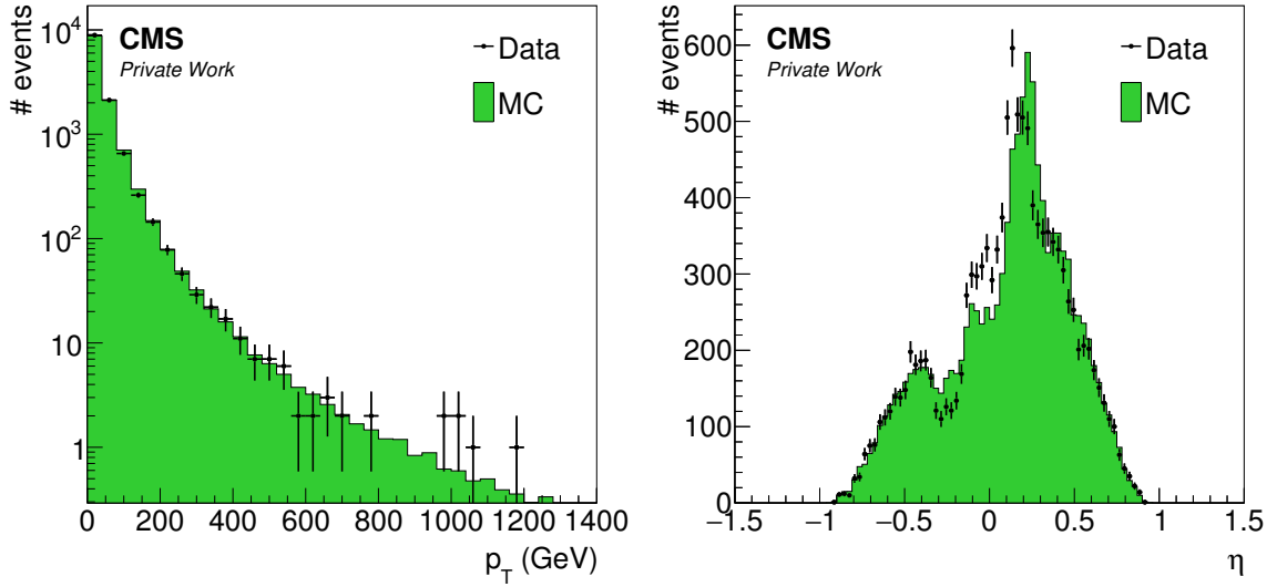
Figure 4.4: Example distributions of the comparison of measured and simulated cosmic muons with the global muon reconstruction. Both have a “high- p_T -ID”-like selection applied.
