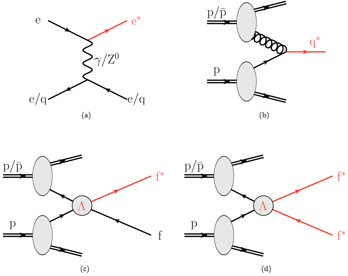
Figure 2.2: Examples for excited fermion ( f^* ) -production: (a) Direct electron excitation by boson exchange in e/p and e^+e^- -collisions; (b) Excited quark production by quark-gluon fusion in pp or p\bar{p} collisions; Associated production of an excited and an ordinary fermion (c) and pair-production (d) of excited fermions ( \ell^*/q^* ) in pp or p\bar{p} collisions. More production mechanisms exist, e.g. including (excited) neutrinos and W -bosons.
