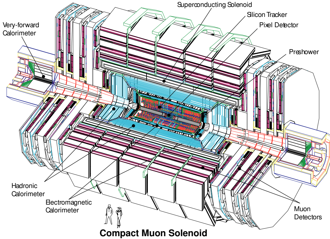
Figure 3.2: Scheme of the CMS detector [59].
