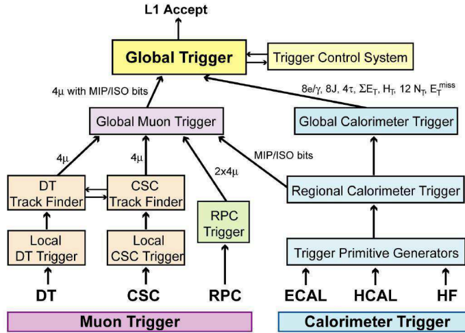
Figure 3.6: Scheme of the CMS L1 trigger (Run I setup) [52].
