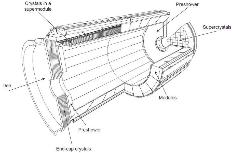
Figure 3.4: The CMS electromagnetic calorimeter [52].
