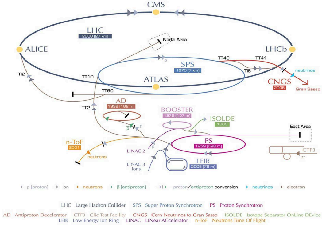
Figure 3.1: The CERN accelerator chain with the LHC and various pre-accelerators. The figure was adapted from [58].
