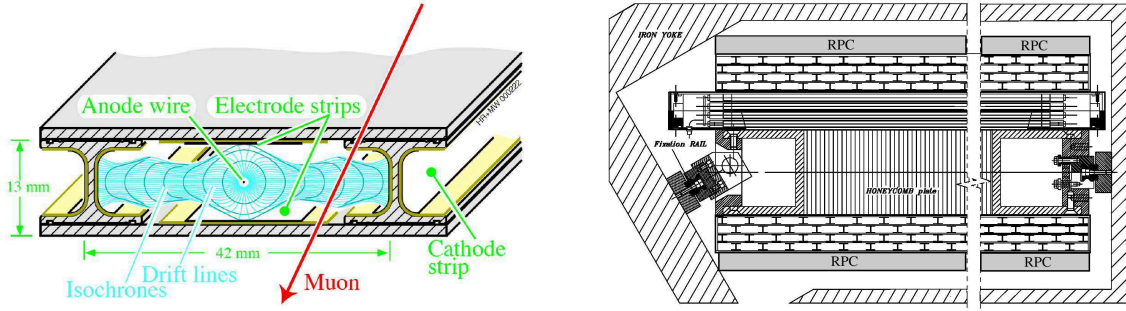
Figure 3.5: Schematic view of a drift tube (left) and a muon station (right) with its superlayers of DTs and RPCs [52]
