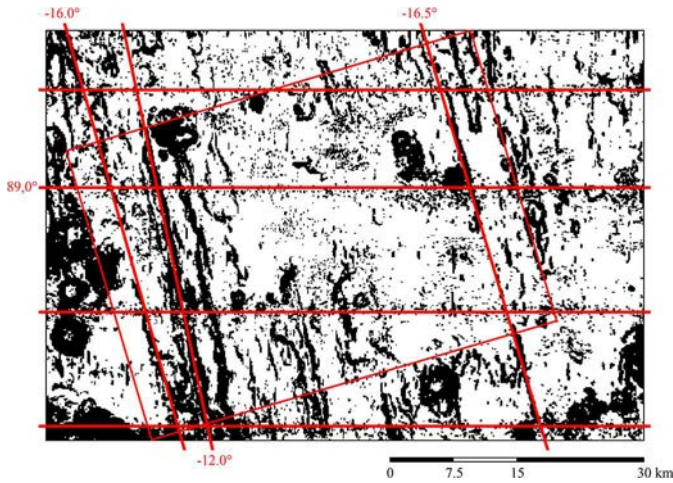
Figure 4. Binary image of the bathymetry of the seafloor in a part of E1 analyzed by Kuhn, Rühlemann, and Wiedicke-Hombach (2012). The inner rectangle indicates the analyzed area. Lines represent interpreted horizontal and vertical image structures.
