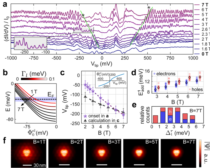
Figure 5. (a) dI/dV spectroscopy in the vicinity of an AA stacked area at varying B , marked on the right. Four spatially adjacent spectra are averaged and the ones for B > 0 T are offset by a value proportional to \sqrt{B} . V_{\text{stab}} = 1000 mV, I_{\text{stab}} = 700 pA, V_{\text{mod}} = 4.2 mV rms . Green lines are guides to the eye, marking the onset voltage of charging peaks V^* . At 7 T, an asterisk marks the first charging peak on either side. Inset shows zoom onto marked peaks. (b) Energy of first confined hole state as a function of induced potential amplitude \Phi_0^{\text{el}} for different B as marked. At larger B , states cross E_F at larger \Phi_0^{\text{el}} , shifting V^* to larger negative V_{\text{tip}} . Color codes imaginary part of the eigenenergy as in Figure 4a. (c) Comparison between measured and calculated V^* . Inset shows the required \Phi_0^{\text{el}}(V_{\text{tip}}) for conversion, taken from a Poisson-solver (Supporting Information) and including a reasonable work function difference of \Delta\Phi = 50 meV between graphene and tip. Error bars for measured V^* reflect typical variation of V^* on AA areas across a few superstructure unit cells. Error bars for calculation arise from the uncertainty in E_F . (d) Plot of the B dependence of E_{\text{add}}^1 \approx E_C^1 of 20 spectra (semitransparent dots) in the vicinity of an AA area. Data points are recorded at integer valued B fields (in Tesla) but displayed slightly shifted to the left (electrons, blue) and to the right (holes, red) for clarity. Median values are encircled in black. (e) Histogram of \Delta_1^1 \approx E_{\text{add}}^2 - E_{\text{add}}^1 (experimental error below 0.2 meV) at B = 7 T for the same AA area used in panel d. Electron (blue bars) and hole (red bars) contributions are colored. (f) Calculated |\Psi| of the first confined hole state (see panel b) crossing E_F at different B as marked. The state originates from LL_{-1} , i.e., V_{\text{tip}} < 0 V when crossing. All scale bars identical.
