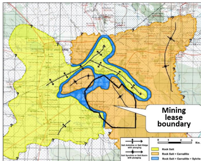
Figure 5.7: Geological structure of Bamnet Narong deposit (ASEAN Potash Mining PLC, 2014a; Suwanich, 2007)
