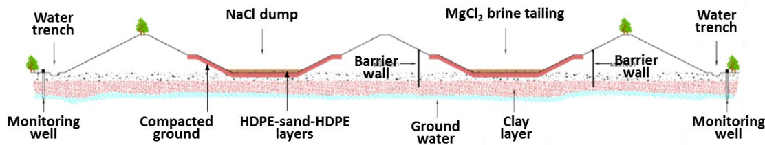
Figure 5.8: Seepage prevention measures in the waste storage facility (Adapted from ASEAN Potash Mining PLC, 2014a, pp. 7–10)
