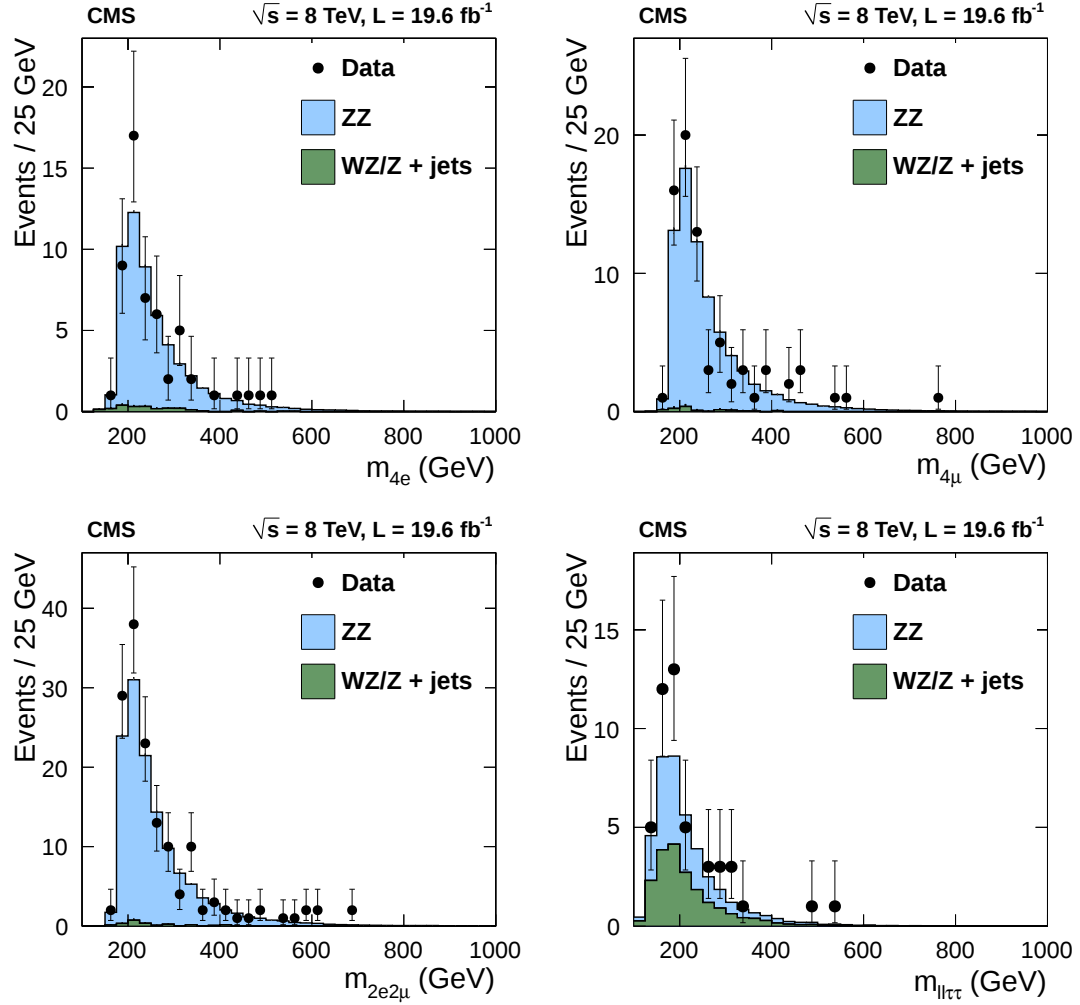
Figure 1: Distribution of the reconstructed four-lepton mass for the (upper left) 4e, (upper right) 4μ, (lower left) 2e2μ, and (lower right) combined \ell\ell\tau\tau decay channels. The data sample corresponds to an integrated luminosity of 19.6 fb⁻¹. Points represent the data, the shaded histograms labeled ZZ represent the POWHEG +GG2ZZ+PYTHIA predictions for ZZ signal, the histograms labeled WZ/Z+jets show the background, which is estimated from data, as described in the text.
