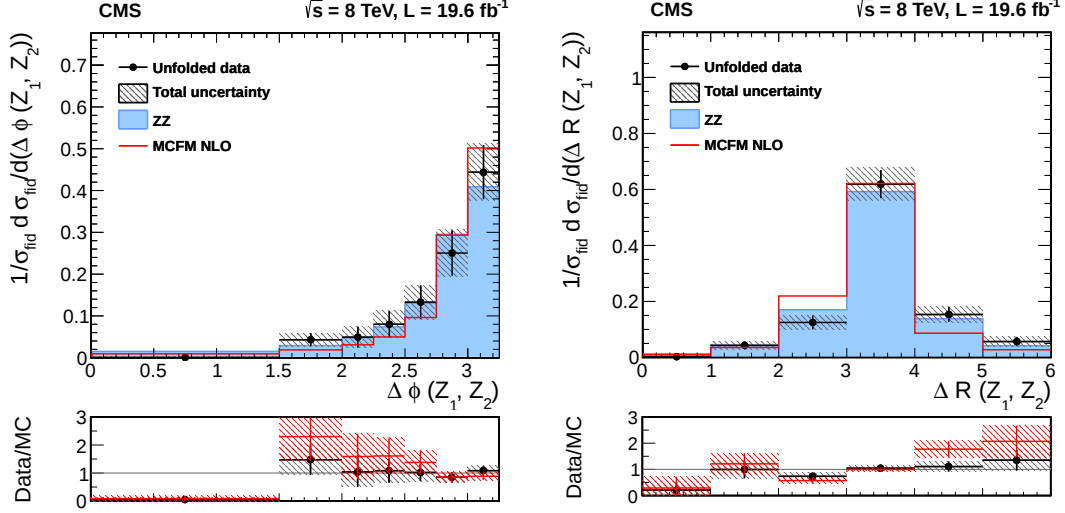
Figure 4: Differential cross section normalized to the fiducial cross section for the combined 4e , 4\mu , and 2e2\mu decay channels as a function of (left) azimuthal separation of the two Z bosons and (right) \Delta R between the Z -bosons. Points represent the data, and the shaded histograms labeled ZZ represent the POWHEG +GG2ZZ+PYTHIA predictions for ZZ signal, while the solid curves correspond to results of the MCFM calculations. The bottom part of each subfigure represents the ratio of the measured cross section to the expected one from POWHEG +GG2ZZ+PYTHIA (black crosses with solid symbols) and MCFM (red crosses). The shaded areas on all the plots represent the full uncertainties calculated as the quadrature sum of the statistical and systematic uncertainties, whereas the crosses represent the statistical uncertainties only.
