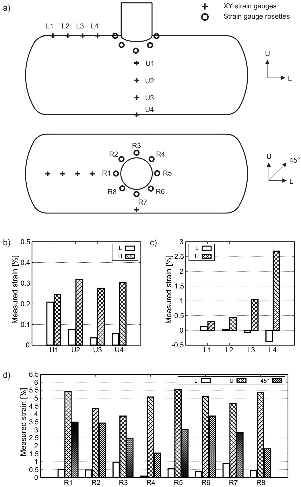
Figure 7.31.: a) Nomenclature of the strain gauges. Results of the measured strain immediately before bursting for strain gauges b) U1 - U4, c) L1 - L4, d) R1 - R8.
