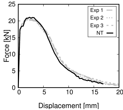
Figure 7.16.: Result of simulation and experiments for Charpy tests at room temperature of dvII.
