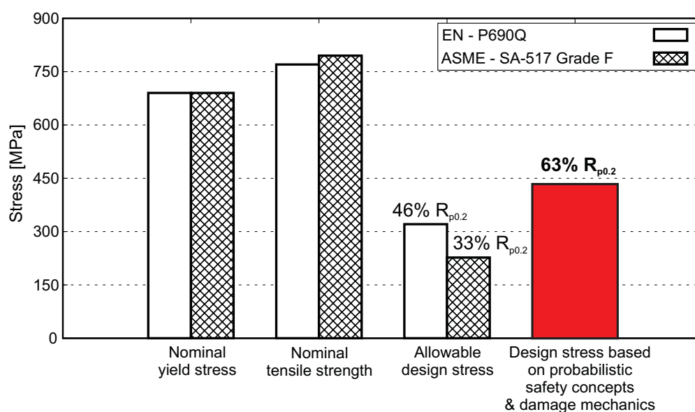
Figure 9.5.: Schematic illustration of the result of the design stress computed by using probabilistic safety concepts in combination with damage mechanics in relation to the currently defined design stresses.
