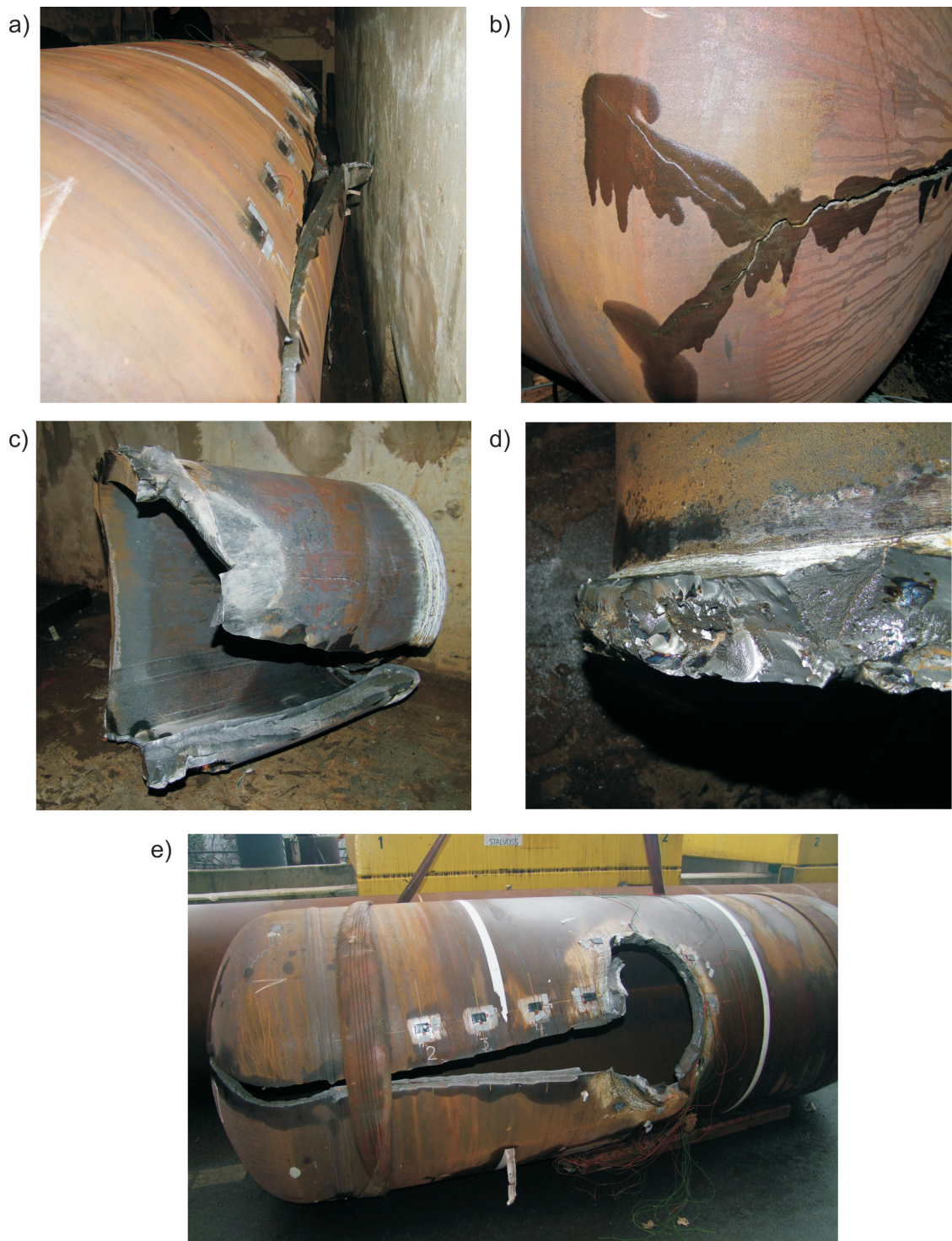
Figure 7.29.: Details of the crack path: a) Crack in the vessel body, b) split end of crack in the front heading, c) split nozzle d) heat tinted material at the nozzle crack surface, e) crack path in the vessel body, visible after relocation from the burst cavern.
