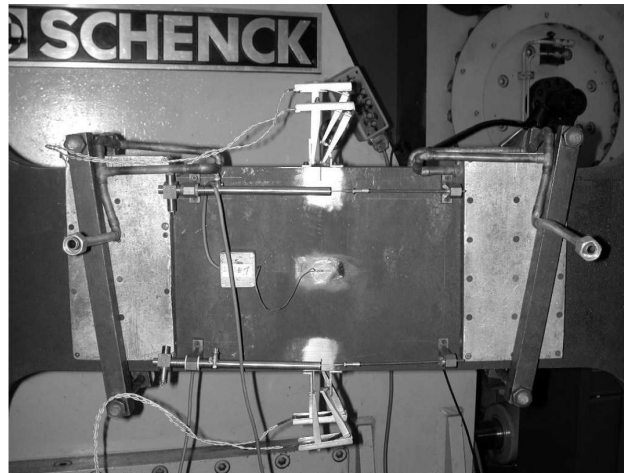
Figure 2.16.: Large-scale pre-cracked tensile sample with a height of 200 mm. The sample is cooled by copper plates at the limits of the test section. The fatigue pre-cracks are located at the end of the two outer notches. Crack mouth opening displacement is measured by clip gauges. Figure from [94].
