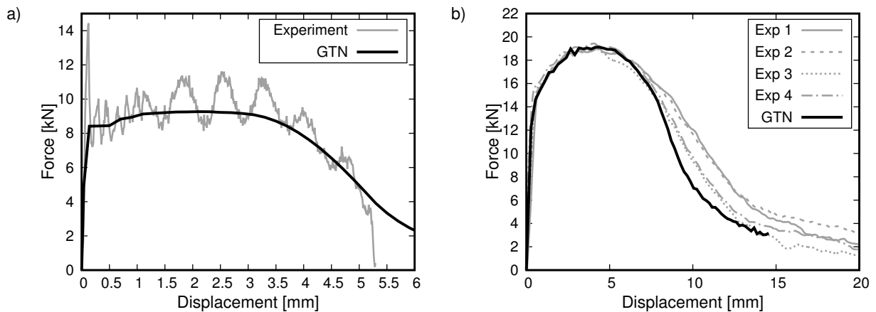
Figure 6.22.: Force-displacement curves of experiments and simulations performed with the re-calibrated parameter set for a) a highspeed tensile test at a strain rate of 250/s b) Charpy tests at room temperature.
