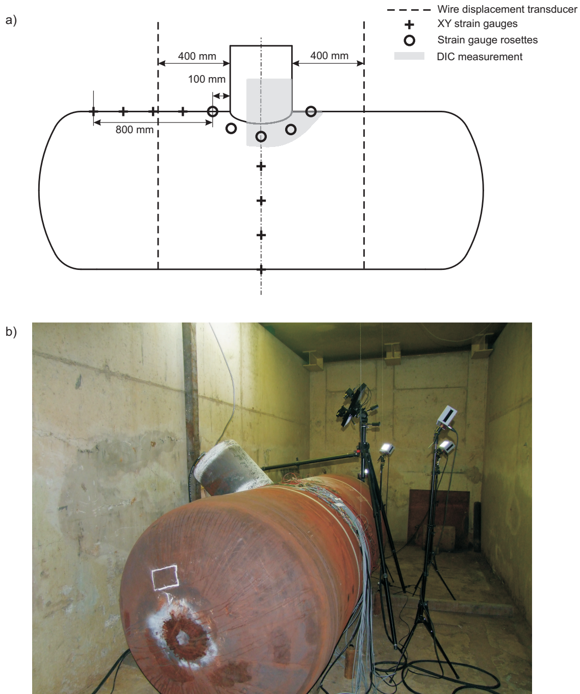
Figure 7.7.: a) Schematic illustration of the vessel instrumentation. b) The instrumented vessel in the burst cavern.
