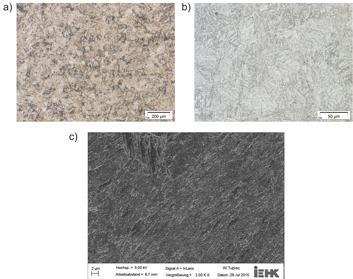
Figure A.9.: Metallographic characterisation of dvI.
