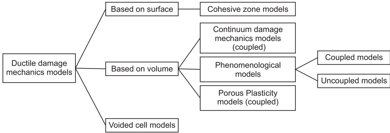
Figure 2.11.: Overview on ductile damage mechanics models, partly adapted from [47]
