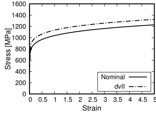
Figure 8.2.: Derived nominal flow curve for P690Q and the original flow curve of dvII in comparison.
