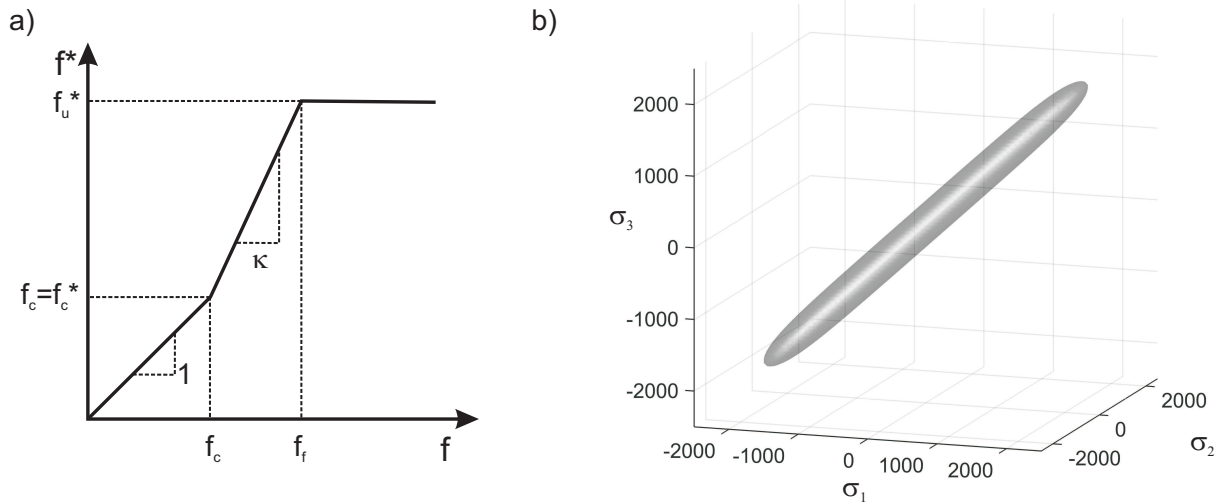
Figure 2.13.: a) Schematic illustration of the evolution of f^* in dependence of f . Figure adapted from [66]. b) Yield potential of the GTN model in principal stress space.
