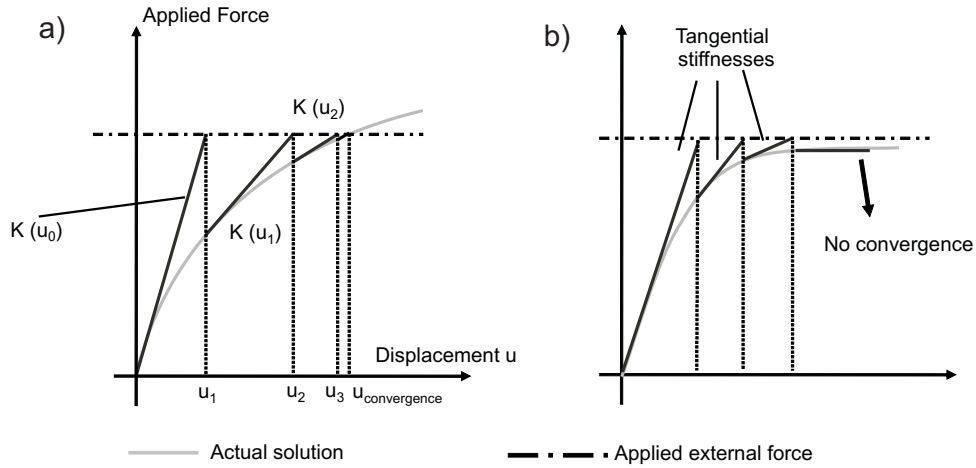
Figure 2.15.: a) Schematic illustration of the Newton-Raphson-Algorithm in FEM and b) the corresponding convergence difficulties for horizontal tangent stiffness matrices. Figure adapted from [20].
