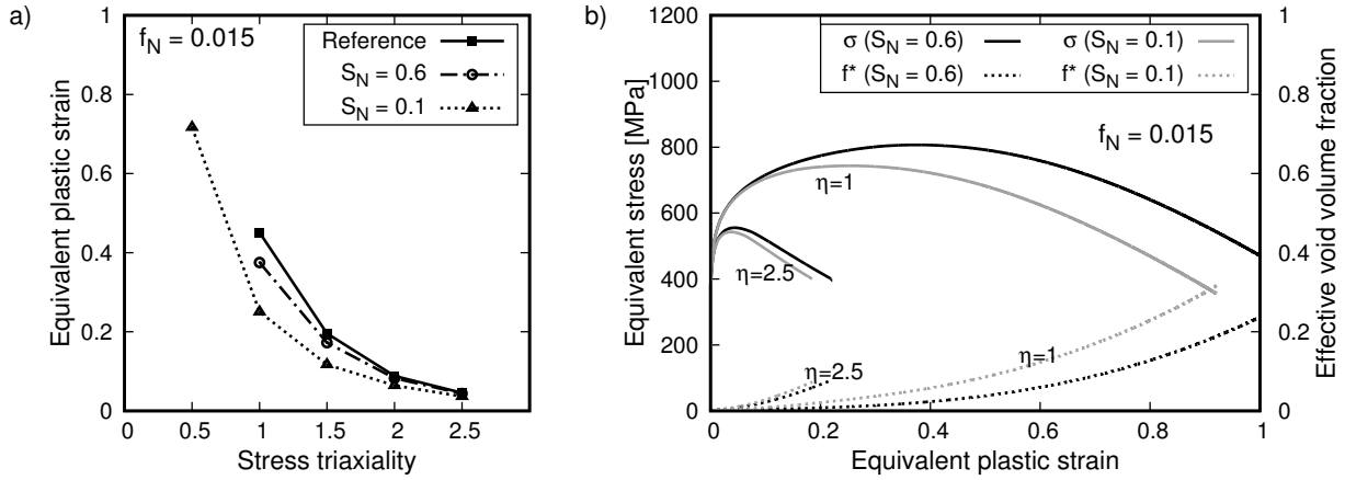
Figure 6.10.: Influence of S_N (with f_N = 0.015 ) on a) derived limit strains from and b) \sigma_e and f^* within cell element simulations for \eta=1.0 and \eta = 2.5 .
