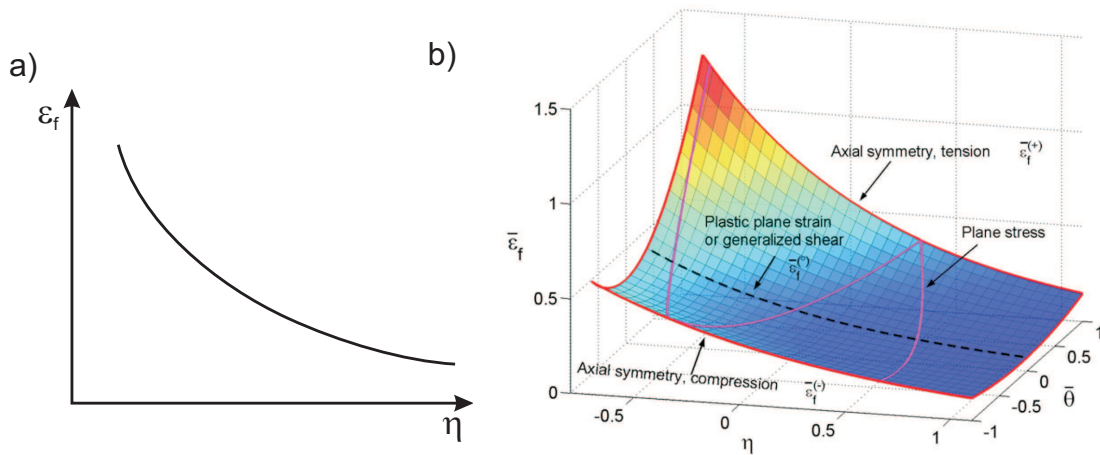
Figure 2.12.: Schematic illustration of a) the JC failure strain definition and b) the BW failure strain definition (taken from [26]).
