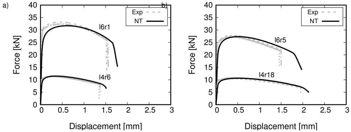
Figure A.21.: Result of NRB simulation and experiments (dashed lines) a) L6R1 and L4R6 b) L6R5 and L4R18 of dvV.
