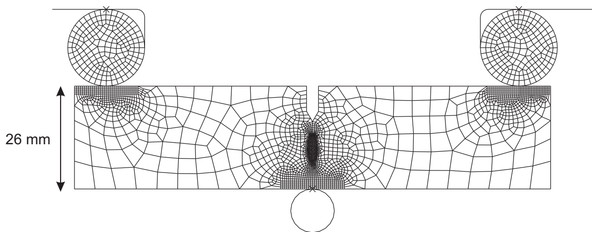
Figure 7.6.: Meshed SENB sample with explicitly modelled bearings.
