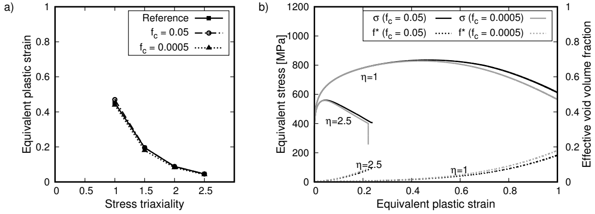
Figure 6.12.: Influence of f_c on a) derived limit strains from and b) \sigma_e and f^* within cell element simulations for \eta=1.0 and \eta = 2.5 .
