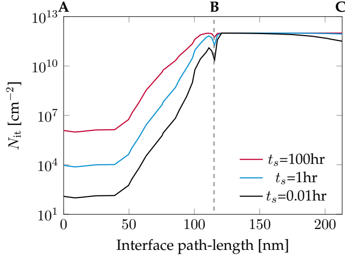
Figure 4.18: Trap densities generated at different stress time steps along the EB spacer oxide interface from node A to C denoted in Fig. 4.15 at V_{EB} = 3 V and V_{CB} = 3 V.
