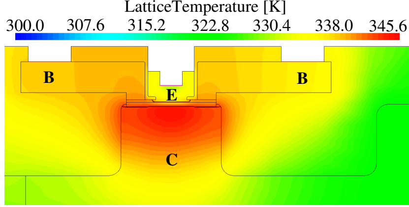
Figure 3.7: Self-consistent lattice temperature at V_{BE} = 0.9 V and V_{CE} = 1 V.
