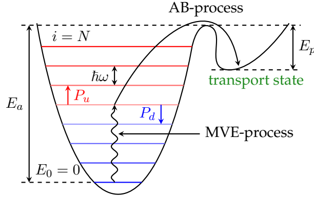
Figure 4.3: The energy configuration of the Si-H bond modeled as a truncated harmonic oscillator.
