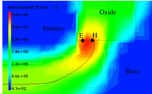
Figure 4.20: Electric field in the SiGe HBT at V_{EB} = 3\text{ V} and V_{CB} = 3\text{ V} . The possible locations of the generated electron (E) and hole (H) due to non-local BTBT have been marked.
