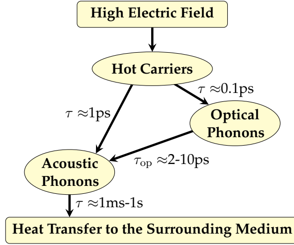
Figure 3.1: Diagram of thermal energy transport in semiconductors.
