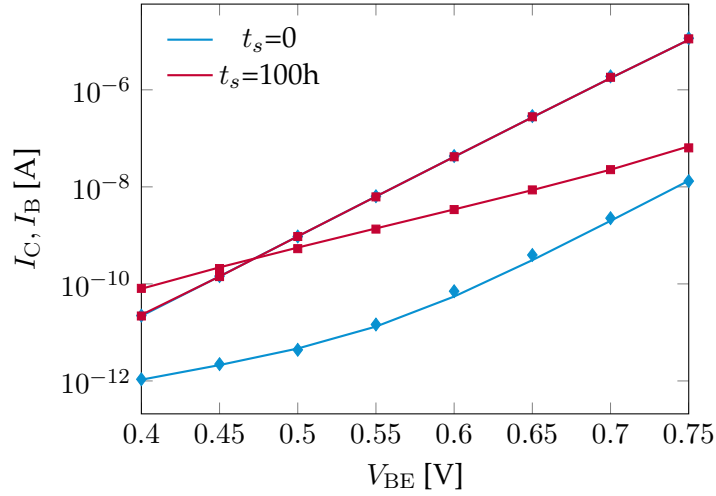
Figure 4.19: Gummel characteristics of the fresh and degraded SiGe HBT after 100 h at V_{EB} = 3 V and V_{CB} = 3 V obtained from simulation (lines) and measurement (symbols).
