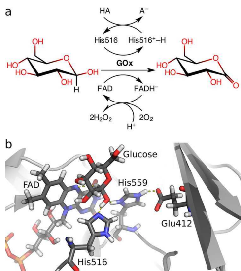
Figure 1. (a) In the reductive half-reaction, glucose binding is followed by concerted proton and hydride transfer from the C1 carbon of glucose to His516 and FAD, respectively. Electrons are then transferred, in the oxidative half-reaction, from reduced FAD to oxygen in two single-electron-transfer steps. (b) The active site of glucose oxidase from A. niger is buried in a pocket, and it is defined by Glu412, His516, His559, and FAD, which are shown as sticks, together with glucose, and colored by atom type (gray, C; blue, N; red, O; white, H; orange, P). The rest of the protein is shown in gray cartoon, and hydrogen bonds are indicated by dashed yellow lines.
