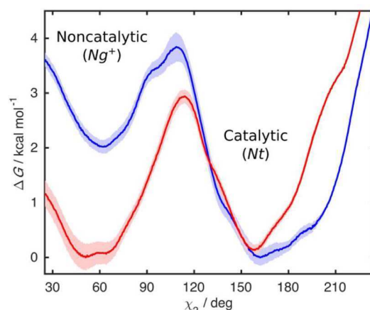
Figure 7. Free energy for the rotation around the \chi_2 dihedral angle of His516: (red) WT GOx; (blue) A2 mutant. The shaded areas around the free energy profiles represent the errors estimated using the blocking procedure.
