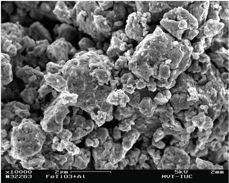
Figure 10. SEM image of formed FeTiO 3 /Al agglomerates.
