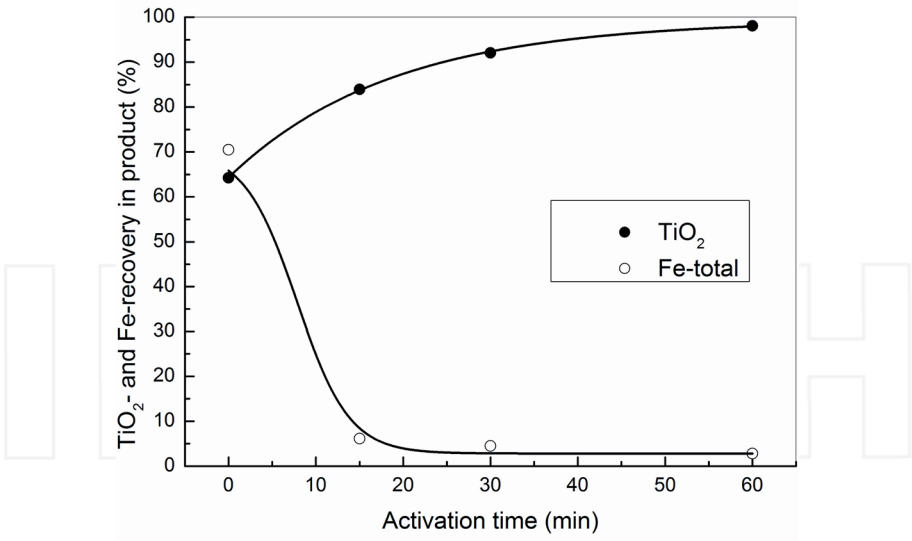
Figure 6. Influence of the mechanical activation time of FeTiO 3 on the precipitation of TiO 2 ; leaching temperature: 150°C, s/l ratio: 50 g.l -1 , leaching time: 60 min, H 2 SO 4 : 30%, and Fe powder: 12%.
