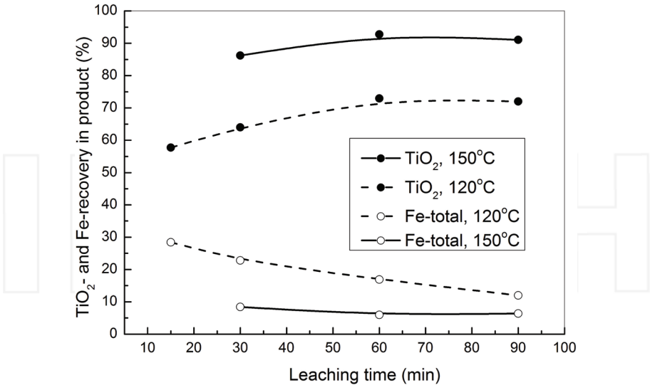
Figure 7. Influence of the leaching time and the temperature on the precipitation of TiO 2 ; s/l ratio: 50 g.l -1 , mechanical activation time: 15 min, H 2 SO 4 : 30%, and Fe powder: 6%.
