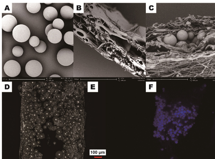
Fig. 4. Morphology of drug-loaded microspheres and PU constructs. (A): SEM pictures of gefitinib-loaded PLGA microspheres (with size range of 50–100 μm); (B): blank PU construct; (C): PU construct (sample GMSP4a) with gefitinib-loaded PLGA microspheres sandwiched between support and top PU layer; (D): laser scanning picture of sample GMSP4a (D); fluorescence microscopy pictures of blank PU construct (E) and sample GMSP4a (F).
