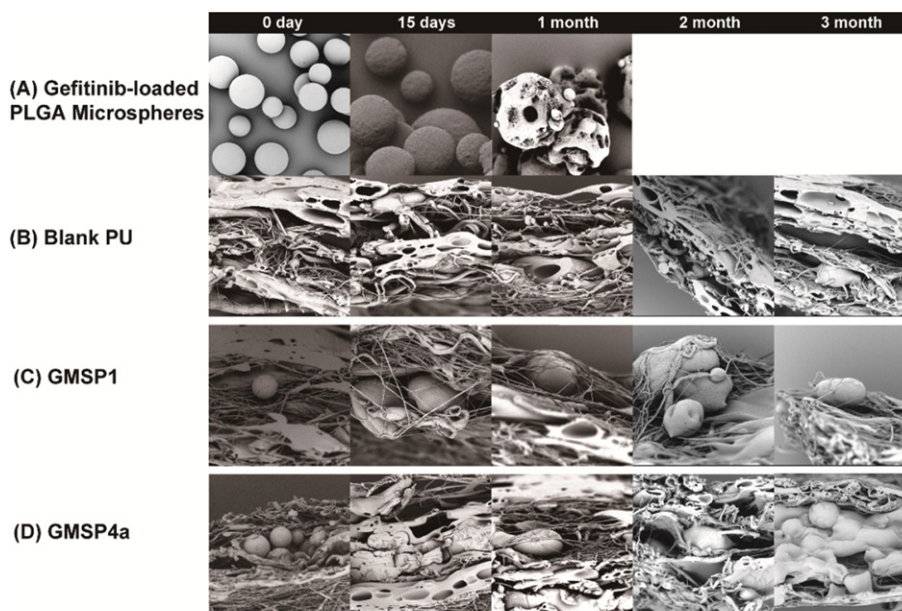
Fig. 8. In vitro degradation of gefitinib-PLGA microspheres embedded in PU constructs. SEM pictures of materials incubated at 37^\circ\text{C} in incubation buffer for indicated time periods. (A): gefitinib-loaded PLGA microspheres; (B): blank PU constructs; (C): GMSP1 construct, i.e. gefitinib-loaded PLGA microspheres deposited on PU support layer without PU top layer; (D): GMSP4a construct in which gefitinib-PLGA microspheres are embedded between support and top PU layer. Magnification is the same for all images ( \times 600 ).
