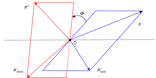
Figure 3 | Definition of the \Phi angle. The decay planes formed by the p\pi_{\text{fast}}^- (blue) and the \pi_{\text{slow}}^-\pi^+ (red) systems in the \Lambda_b^0 rest frame. The momenta of the particles, represented by vectors, determine the two decay planes and the angle \Phi \in [-\pi, \pi] (ref. 19) measures their relative orientation.
