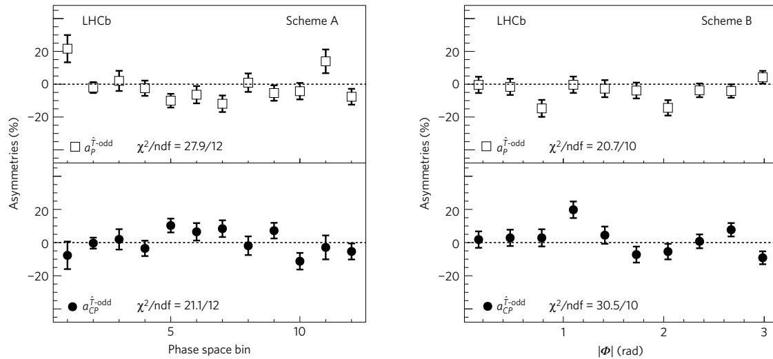
Figure 4 | Distributions of the asymmetries. The results of the fit in each region of binning schemes A and B are shown. The asymmetries a_P^{\bar{T}\text{-odd}} and a_{CP}^{\bar{T}\text{-odd}} for \Lambda_b^0 \rightarrow p\pi^-\pi^+\pi^- decays are represented by open boxes and filled circles, respectively. The error bars represent one standard deviation, calculated as the sum in quadrature of the statistical uncertainty resulting from the fit to the invariant mass distribution and the systematic uncertainties estimated as described in the main text. The values of the \chi^2/\text{ndf} are quoted for the P - and CP -conserving hypotheses for each binning scheme, where ndf indicates the number of degrees of freedom.
