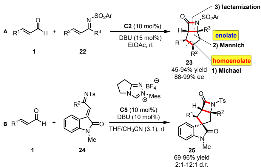
Scheme 13. Domino \alpha^3 - d^3 Umpolung/Michael/Mannich/Lactamization Reaction
