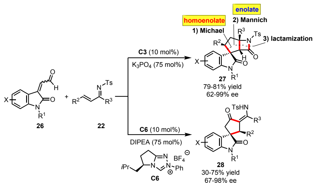
Scheme 14. Domino \alpha^3 - d^3 Umpolung/Michael/Mannich/Lactamization Reaction of Isatin-Derived Enals
