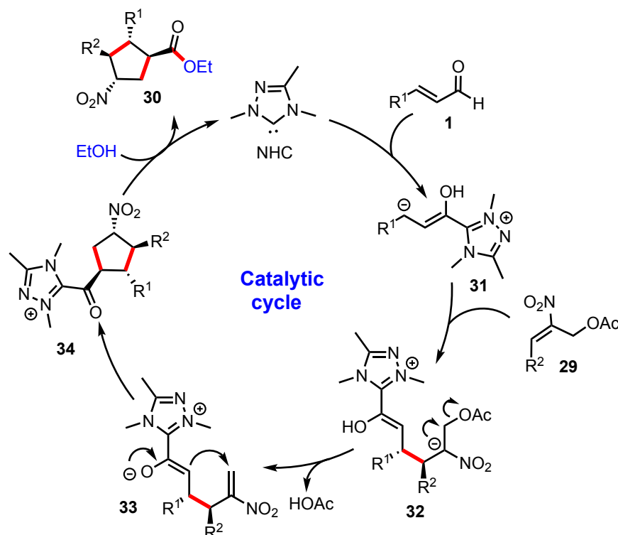
Scheme 16. Proposed Mechanism for Domino a^3 - d^3 Umpolung/Michael/Michael/Esterification Reaction
