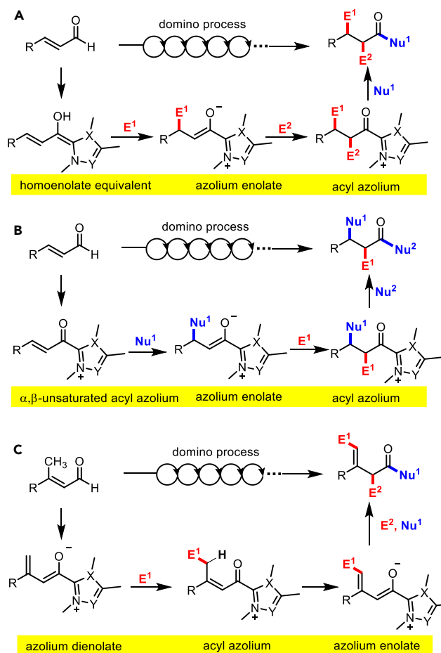
Scheme 3. Classification of NHC-Catalyzed Domino Reactions via Two or More Activation Modes
