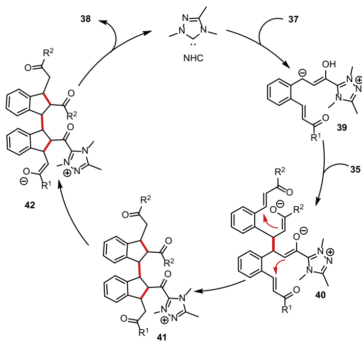
Scheme 18. Domino \alpha^3 - d^3 Umpolung/Michael/Michael/Michael/Lactonization Reaction
