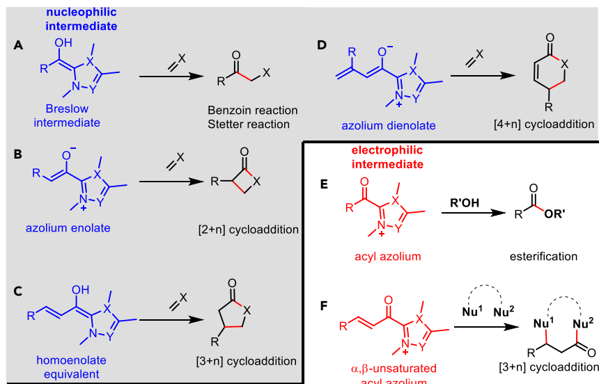
Scheme 1. Summary of Classic Reactions via NHC Catalysis
