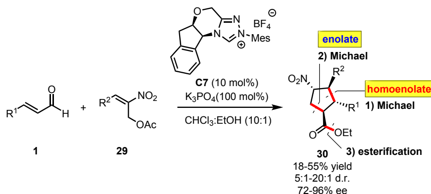
Scheme 15. Domino a^3 - d^3 Umpolung/Michael/Michael/Esterification Reaction
