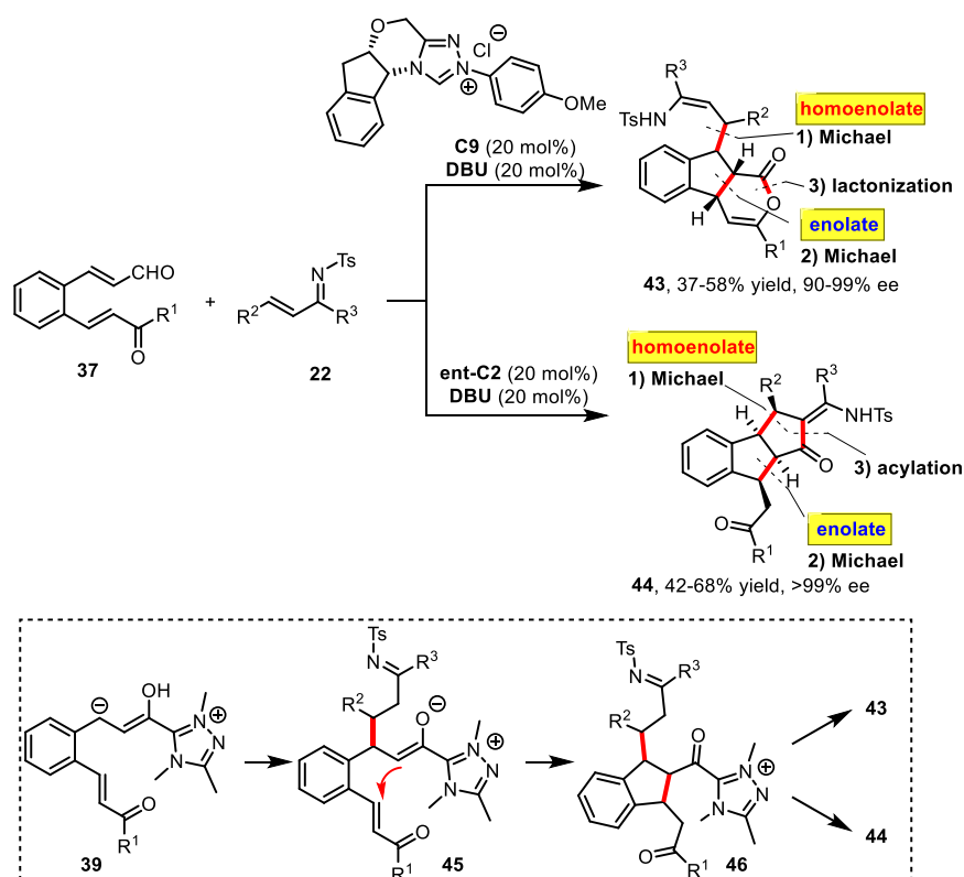
Scheme 19. Domino a^3 - d^3 Umpolung/Michael/Michael/Lactonization Reaction of 2-Aroylvinylcinnamaldehydes
