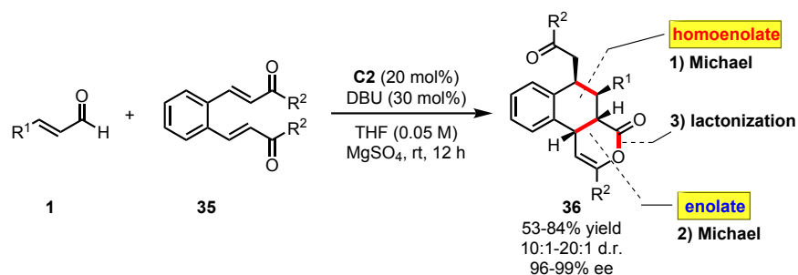
Scheme 17. Domino \alpha^3 - d^3 Umpolung/Michael/Michael/Esterification Between Benzodienones and \alpha,\beta -Unsaturated Aldehydes
