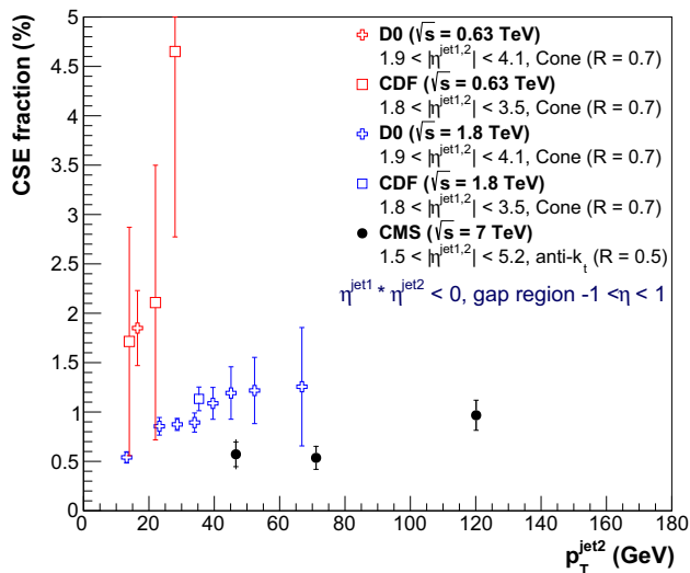
Fig. 8 Fraction of dijet events with a central gap ( f_{\text{CSE}} ) as a function of p_{\text{T}}^{\text{jet}2} at \sqrt{s} = 7 TeV, compared to the D0 [27] and CDF [29,30] results at \sqrt{s} = 0.63 and 1.8 TeV. The details of the jet selections are given in the legend. The results are plotted at the mean value of p_{\text{T}}^{\text{jet}2} in the bin. The inner and outer error bars represent the statistical, and the statistical and systematic uncertainties added in quadrature, respectively
