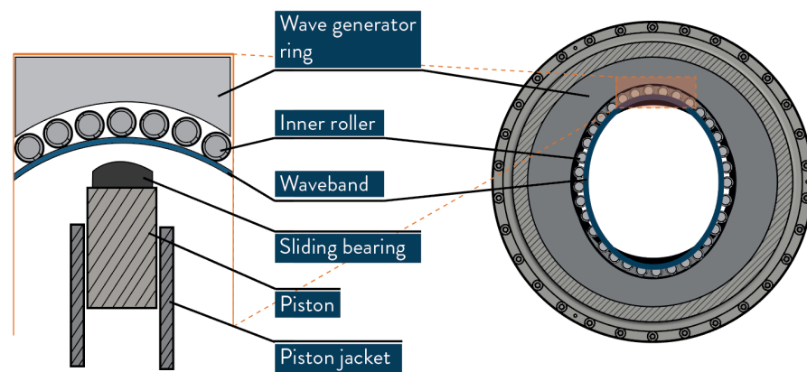
Figure 3: Sliding surface bearing approach. By adding additional rollers and a so-called waveband, the piston is actuated through almost pure translation.
