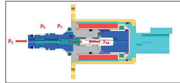
Figure 1: Force balance of a direct operating pressure reducing valve
