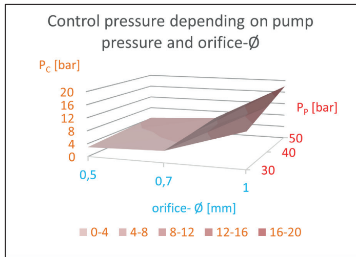
Figure 9: Residual control pressure of a PPCD04 Fail Safe valve with respect to the pump pressure and an additional orifice.
