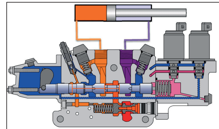
Figure 2: Sectional valve with two pilot valves. One energized and acting on a hydraulic cylinder.
