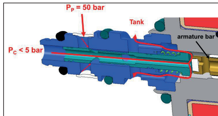
Figure 3: Functional principle of a fail safe valve. Basic type PPCD04 with nominal flow 4 l/min.
