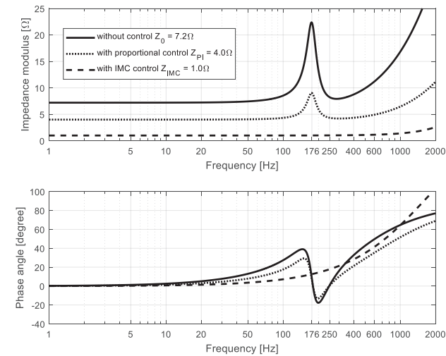
Figure 7: Comparison between impedance curves using different control strategies
