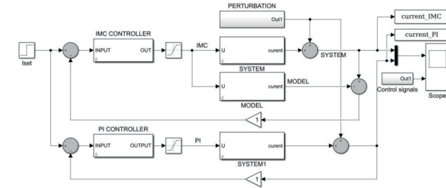
Figure 9: The simulation model - Simulink
