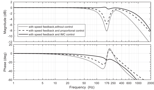
Figure 8: Current dynamics - Bode plot
