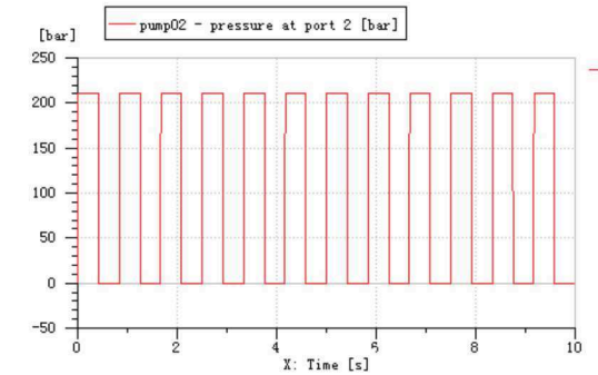
Figure 6: The pressure of the pump's right port.
