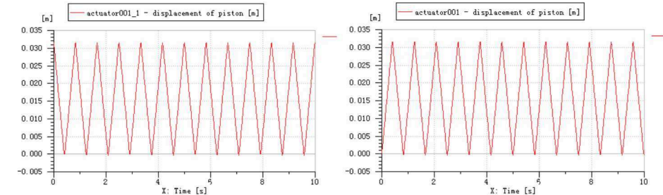
Figure 7: The displacement of the two actuators.
