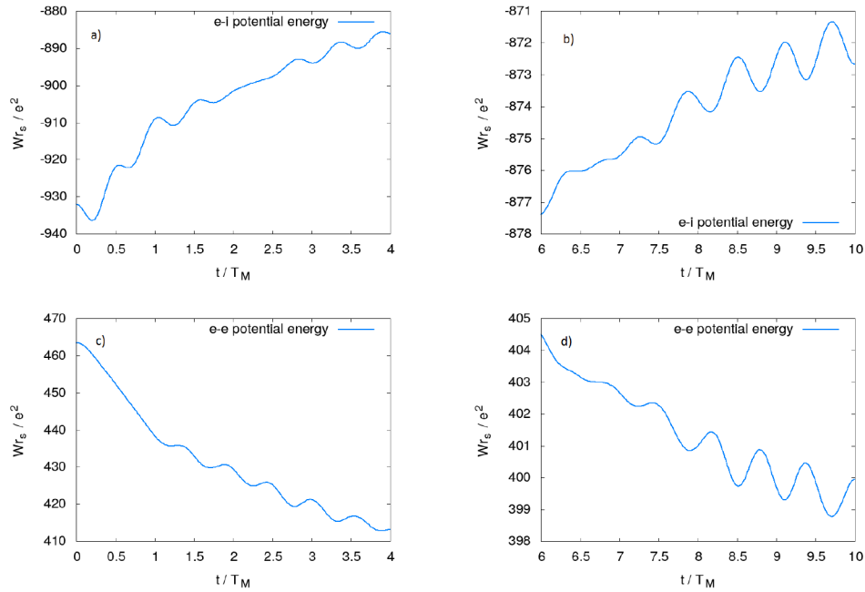
Figure 4. Evolution of potential energies. The magnitude of the potentials decreases due to the increase of the extension of the electron cloud. Furthermore, a decrease of the oscillation frequency indicates a conversion from surface modes with frequency 2\omega_M to volume modes with frequencies in the range of \omega_p . a) Initial and b) final stage of the electron-ion potential energy. c) Initial and d) final stage of the electron-electron potential energy. ( R = 28 , \Gamma = 0.1 , \Delta x = 0.15R )
