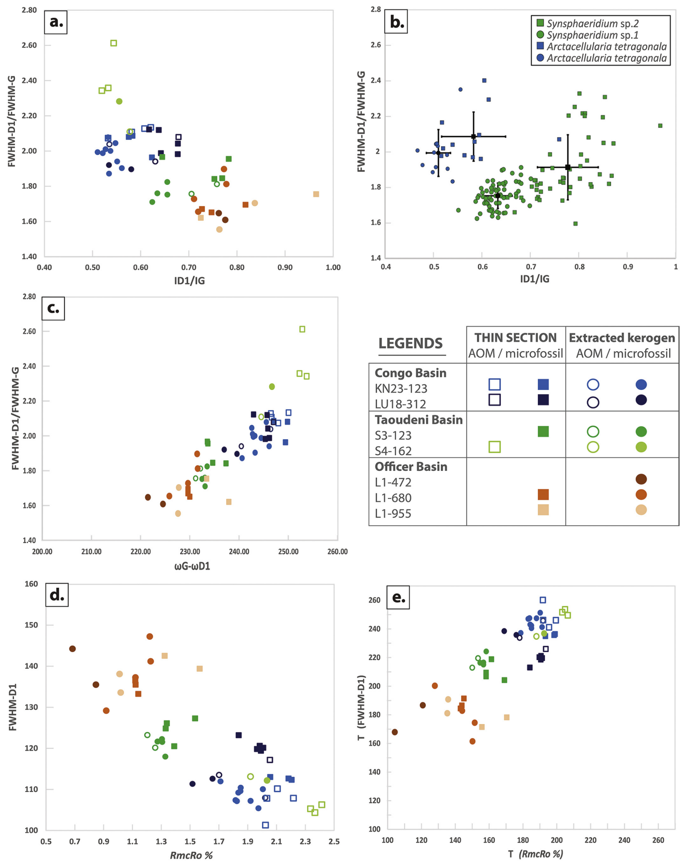
Fig. 3. (a) Average values of FWHM-D1/FWHM-G ratio vs ID1/IG ratio. (b) Analyses for the specimens Synsphaeridium in S3 drill core and Arctacellularia tetragonal a in Kanshi drill core (extracted kerogen and thin section). Means and standard deviations are in black. (c) FWHM-D1/FWHM-G ratio vs \omega G-\omega D1 . (d) FWHM-D1 vs RmcRo\% and (e) T FWHM-D1 (Eq. 5) and T RmcRo\% .
