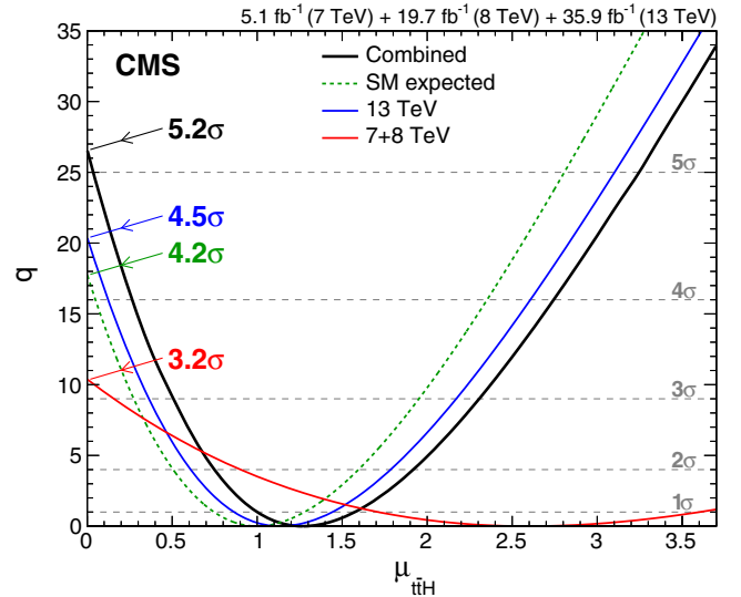
FIG. 4. Test statistic q , described in the text, as a function of \mu_{t\bar{t}H} for all decay modes at 7 + 8 TeV and at 13 TeV, separately, and for all decay modes at all c.m. energies. The expected SM result for the overall combination is also shown. The horizontal dashed lines indicate the p values for the background-only hypothesis obtained from the asymptotic distribution of q , expressed in units of the number of standard deviations.
