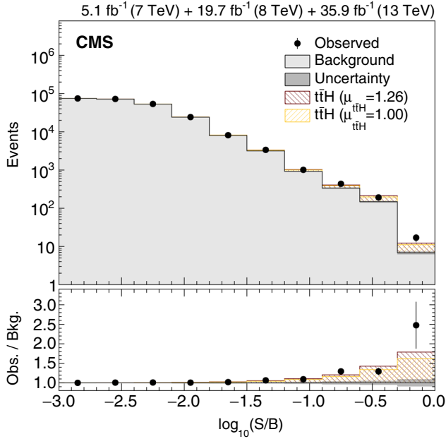
FIG. 3. Distribution of events as a function of the decimal logarithm of S/B , where S and B are the expected postfit signal (with \mu_{t\bar{t}H} = 1 ) and background yields, respectively, in each bin of the distributions considered in this combination. The shaded histogram shows the expected background distribution. The two hatched histograms, each stacked on top of the background histogram, show the signal expectation for the SM ( \mu_{t\bar{t}H} = 1 ) and the observed ( \mu_{t\bar{t}H} = 1.26 ) signal strengths. The lower panel shows the ratios of the expected signal and observed results relative to the expected background.
