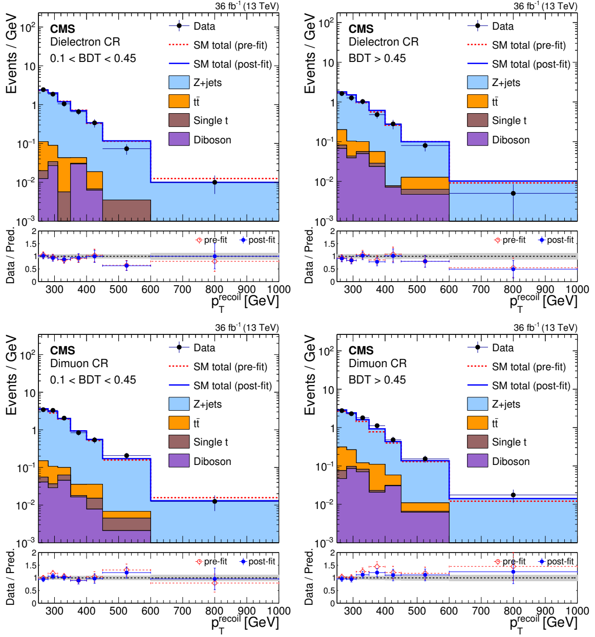
Figure 4. Comparison between data and SM predictions in the dilepton control regions before and after performing the simultaneous fit to the different control regions and signal region. Each bin shows the event yields divided by the width of the bin. The upper row of figures corresponds to the dielectron control region, and the lower row to the dimuon control region. The left (right) column of figures corresponds to the loose (tight) category of the control regions. The blue solid line represents the sum of the SM contributions normalized to their fitted yields. The red dashed line represents the sum of the SM contributions normalized to the prediction. The stacked histograms show the individual fitted SM contributions. The lower panel of each figure shows the ratio of data to fitted prediction. The gray band on the ratio indicates the one standard deviation uncertainty on the prediction after propagating all the systematic uncertainties and their correlations in the fit.
