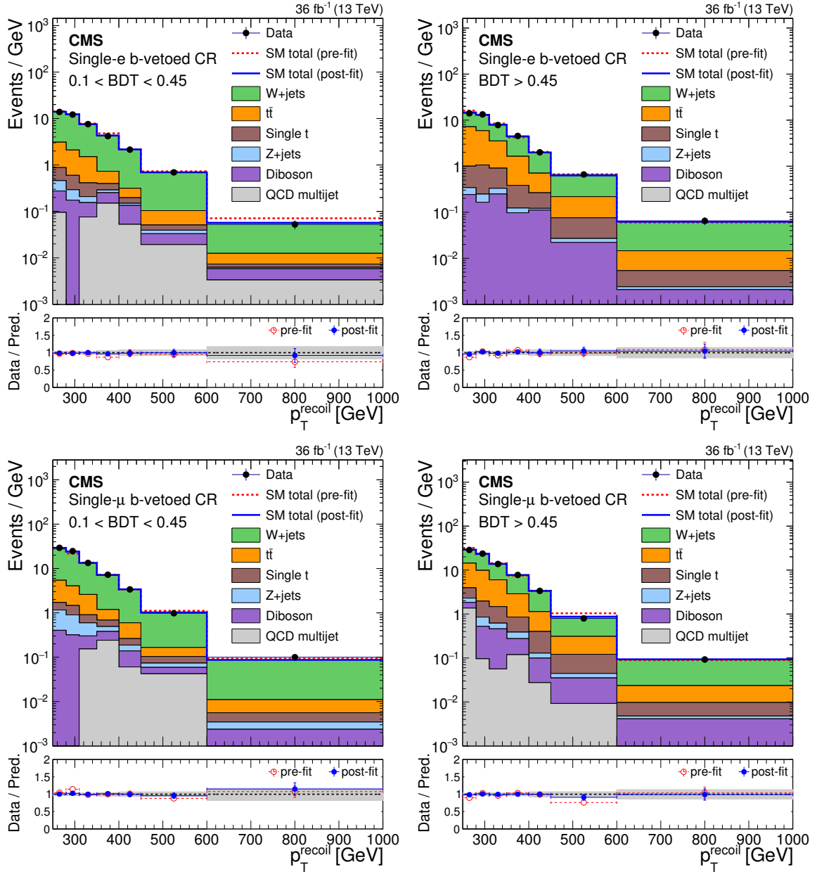
Figure 6. Comparison between data and SM predictions in the b-vetoed single lepton control regions before and after performing the simultaneous fit to the different bin control regions and signal region. Each bin shows the event yields divided by the width of the bin. The upper row of figures corresponds to the single electron b-vetoed control region, and lower row to the single muon b-vetoed control region. The left (right) column of figures corresponds to the loose (tight) category of the control regions. The blue solid line represents the sum of the SM contributions normalized to their fitted yields. The red dashed line represents the sum of the SM contributions normalized to the prediction. The stacked histograms show the individual fitted SM contributions. The lower panel of each figure shows the ratio of data to fitted prediction. The gray band on the ratio indicates the one standard deviation uncertainty on the prediction after propagating all the systematic uncertainties and their correlations in the fit.
