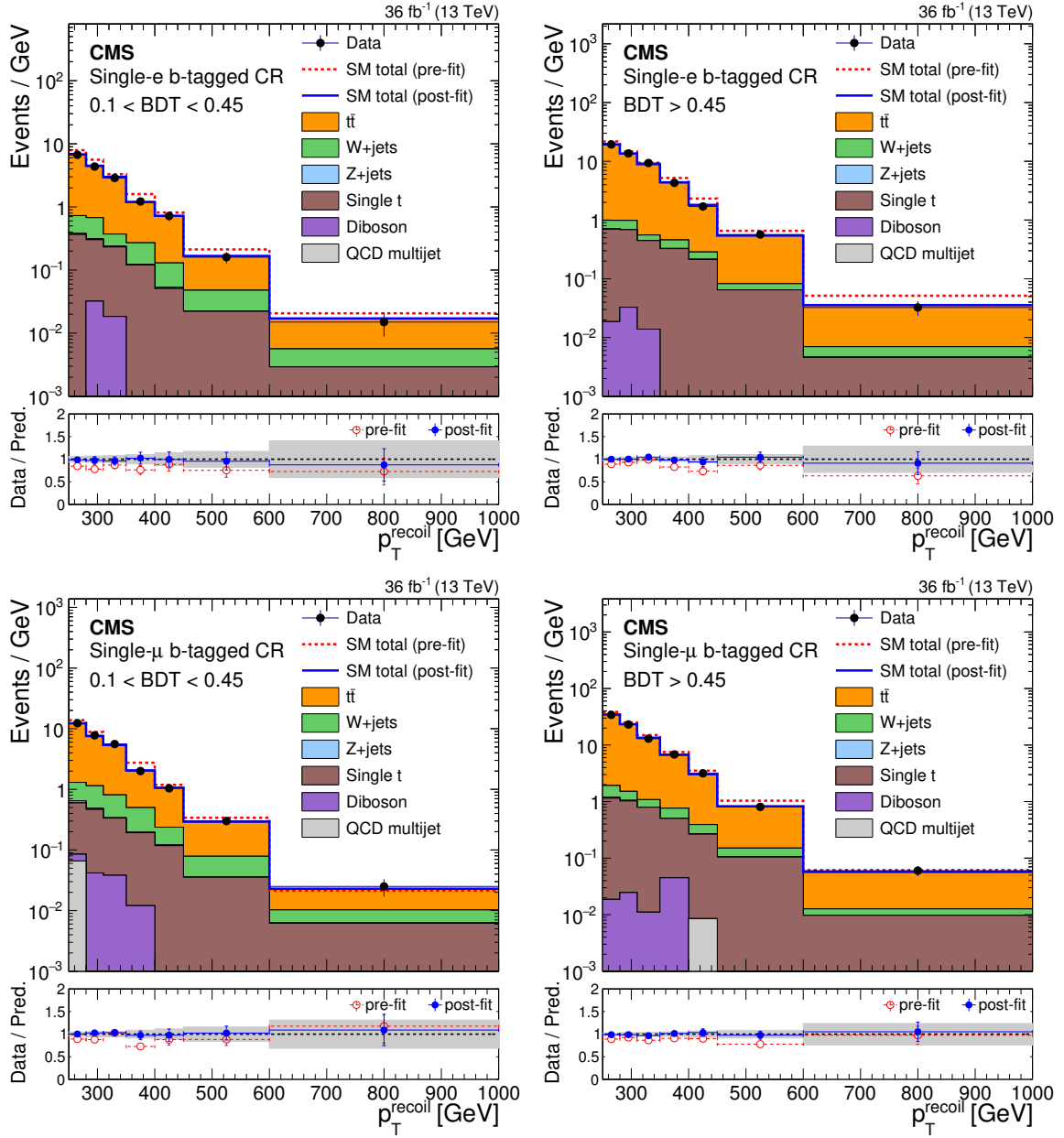
Figure 7. Comparison between data and SM predictions in the b-tagged single lepton control regions before and after performing the simultaneous fit to the different bin control regions and signal region. Each bin shows the event yields divided by the width of the bin. The upper row of figures corresponds to the single electron b-tagged control region, and lower row to the single muon b-tagged control region. The left (right) column of figures corresponds to the loose (tight) category of the control regions. The blue solid line represents the sum of the SM contributions normalized to their fitted yields. The red dashed line represents the sum of the SM contributions normalized to the prediction. The stacked histograms show the individual fitted SM contributions. The lower panel of each figure shows the ratio of data to fitted prediction. The gray band on the ratio indicates the one standard deviation uncertainty on the prediction after propagating all the systematic uncertainties and their correlations in the fit.
