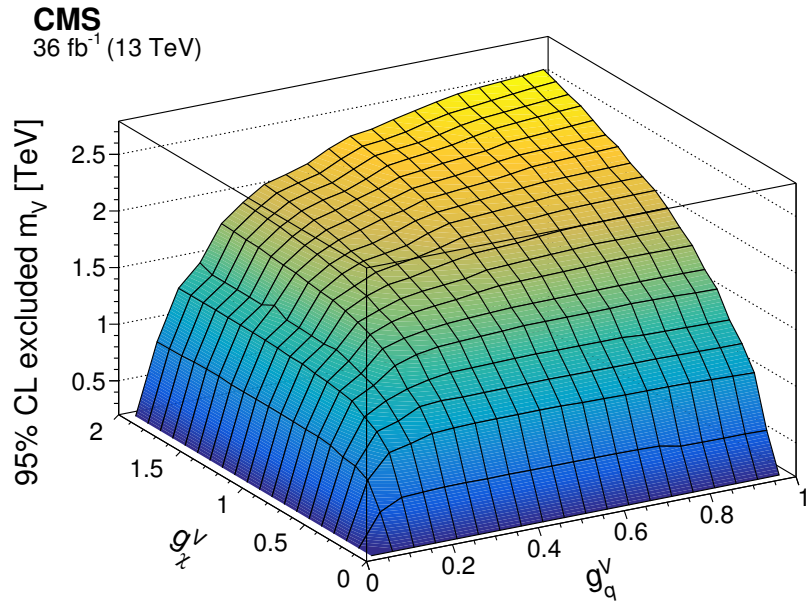
Figure 20. The maximum excluded mediator mass at 95% CL as a function of vector couplings to DM and quarks. This plot fixes m_\chi = 1 GeV and g_\chi^A = g_q^A = 0 . Masses up to 2.5 TeV are excluded given sufficiently large coupling choices.
