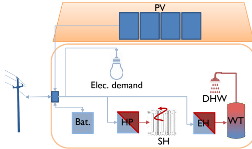
Figure 4.4: Thermal (red) and electrical (blue) representation of the considered house set up with a heat pump (HP) supplying the space heating (SH), an electrical heater (EH) supplying a water tank (WT) for domestic hot water demand (DHW), photovoltaic panels (PV) and domestic battery.
