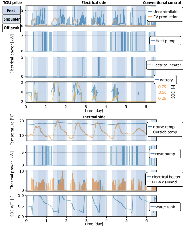
Figure 4.8: Illustration of conventional control with TOU tariff.
