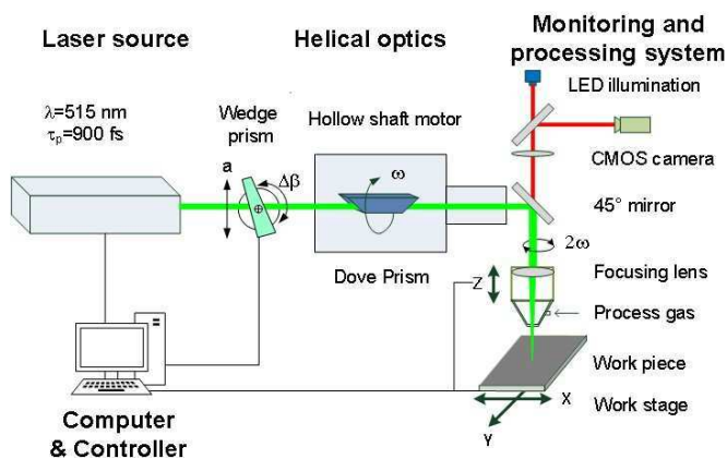
Fig. 1. Schematic of the helical drilling systems
