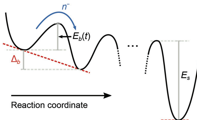
Figure 2. Sketch of the collective relaxation model. The amorphous state created via the melt-quench process is in an unstable state and proceeds through a sequence of transitions toward the energetically more favorable “ideal glass” state. The activation energy E_b(t) for collective reconfigurations grows as they involve the movement of atoms that have been increasingly stabilized in their positions through previous relaxation steps.
