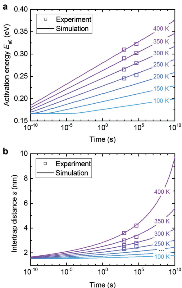
Figure 5. Illustration of the drift model. Both E_{a0} and 1/s are assumed to vary linearly with the order parameter \Sigma to constitute the drift model. Those relationships are plotted in (a) and (b) for different ambient temperatures along with the experimental data points of Figure 4.
