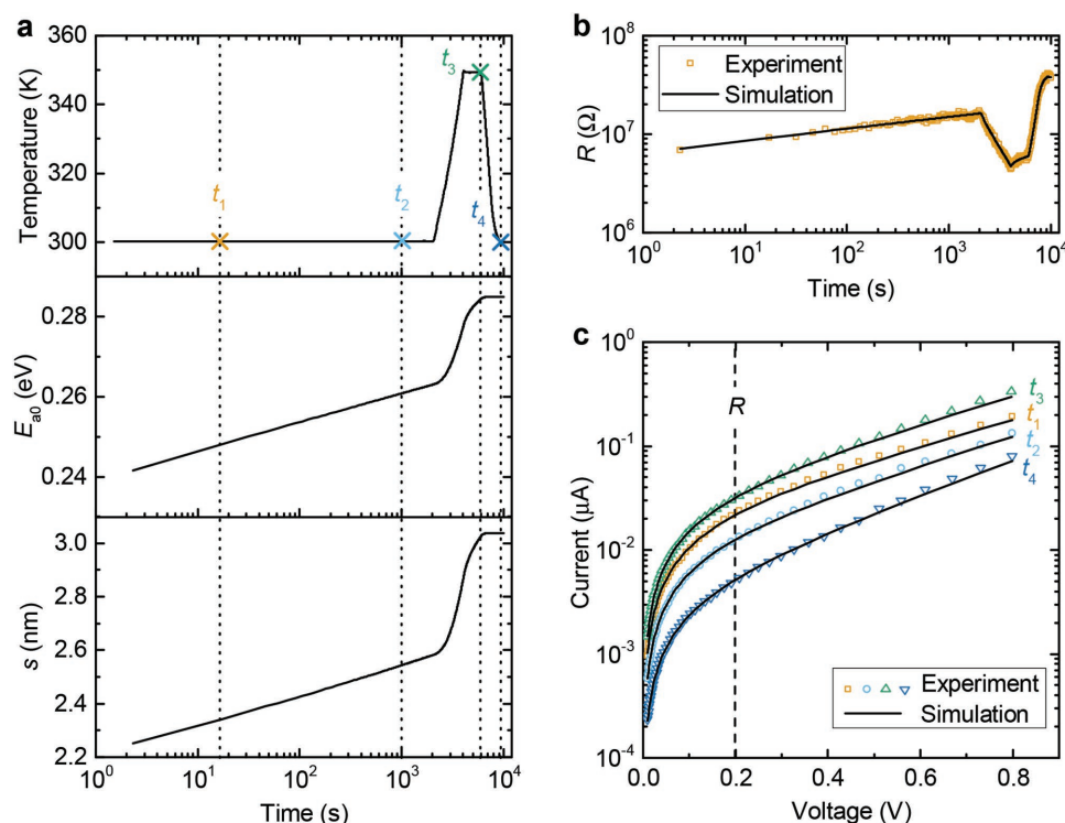
Figure 7. Variable temperature I – V drift experiment. a) Temperature profile applied to the PCM device and corresponding evolutions of E_{a0} and s obtained from the drift model. b) Experimental and simulated evolution of the low-field resistance R . c) Experimental and simulated I – V characteristics at four instances in time.
