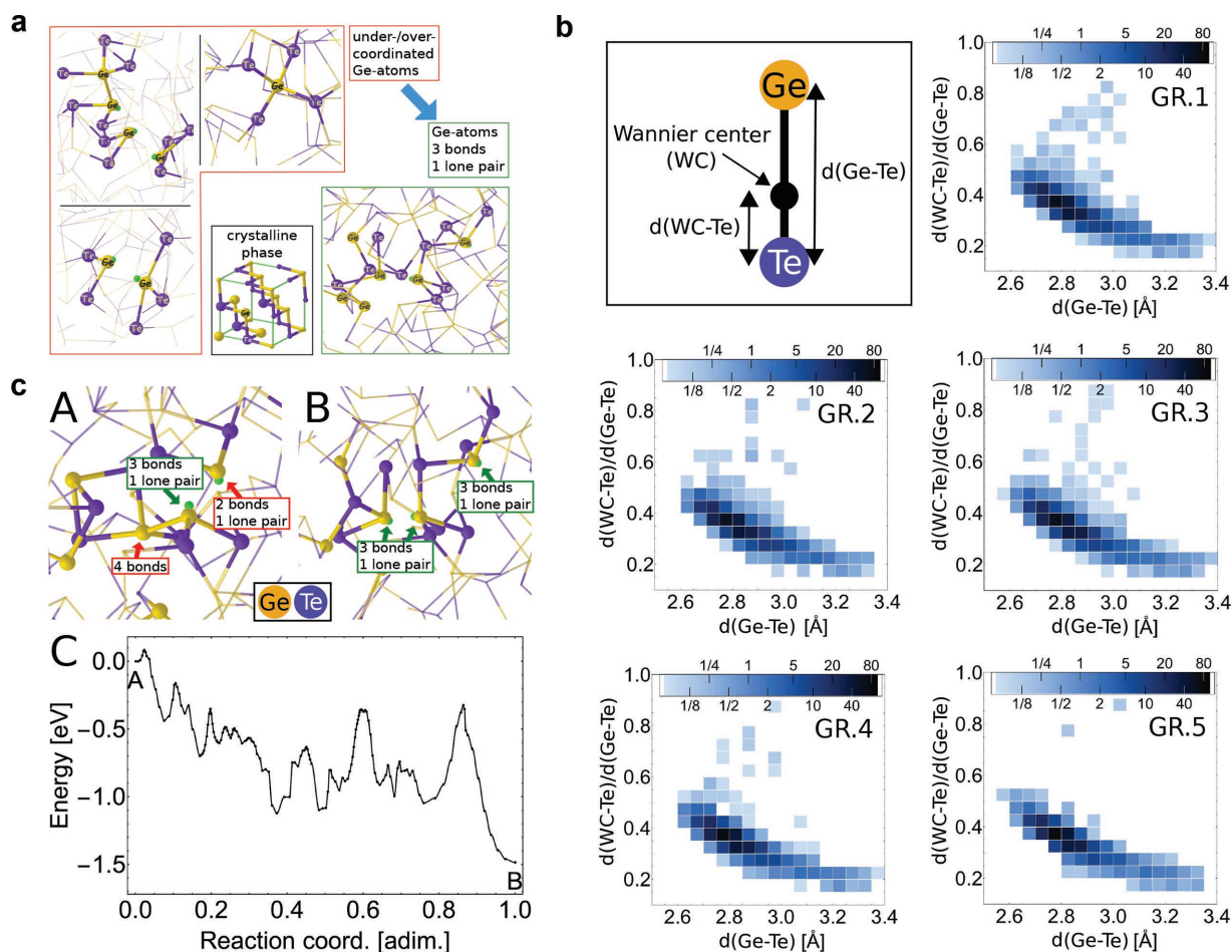
Figure 1. Structural relaxation in amorphous GeTe. a) Examples of structures with Ge atoms having a bond configuration different from the ideal chemically ordered threefold one are illustrated within the red contour. Such structures are responsible for localized electronic states in the bandgap. Recent studies show that resistance drift is mostly caused by a gradual transition of these structures formed during the melt-quench process toward lower energy structures having more ideal configurations. The green box shows an example of an amorphous region consisting of Ge atoms with threefold bond configurations. Ge and Te atoms are depicted as dark yellow and violet spheres, respectively. Bonds between these atoms, determined using Wannier analysis [22,24] are indicated by cylinders and the surrounding bond network via thin lines. b) The link between distribution of bond configurations and conductivity is shown here. Each histogram shows the distribution of bond configurations of all the Ge–Te bonds characterized by bond polarization and bond distance. Sixty-five structures obtained via classical MD simulations and analyzed via first-principles calculations are grouped into five sets ranging from high conductivity (GR.1) to low conductivity (GR.5), see ref. [22] for more details. The number of bonds in each bin normalized by the number of configurations of the group is indicated by the color scale. Amorphous states with a higher conductivity show a broader distribution. Upon relaxation, i.e., with decreasing conductivity, the distribution of Ge–Te bonds becomes sharper and outliers disappear. c) The energy profile associated with the annealing of a defective Ge–Te structure is shown. The starting condition (Panel A) produces an electronic state in the bandgap. In the final state (Panel B), i.e., after the annealing, the defective configurations causing the localized electronic state are removed. Red arrows indicate the Ge atoms with defective configurations. Green arrows indicate Ge atoms with an ideal threefold bond configuration. The minimum energy pathway at T = 0 K (Panel C) shows that the process occurs via a complex sequence of activated processes characterized by a changing collective activation energy. Adapted from ref. [22].
