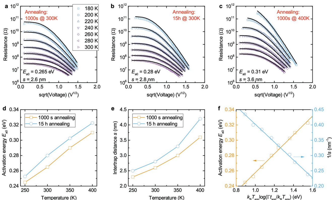
Figure 4. Link between electrical transport and structural relaxation. a–c) Experimental resistance versus voltage curves of RESET state measured from 300 K down to 180 K after annealing. Three annealing conditions are shown, exhibiting higher low-field resistance and stronger voltage dependence for both increasing annealing time and temperature. Fits of the temperature dependent I – V characteristics underlying the data in (a)–(c) using the electrical transport model described in Section 5 (black lines) result in activation energy E_{a0} d) and intertrap distance s e) for different annealing times and temperatures. f) E_{a0} and 1/s plotted as function of k_B T_{\text{ann}} \log(\Gamma t_{\text{ann}}/k_B T_{\text{ann}}) , where T_{\text{ann}} is the annealing temperature and t_{\text{ann}} the annealing time.
