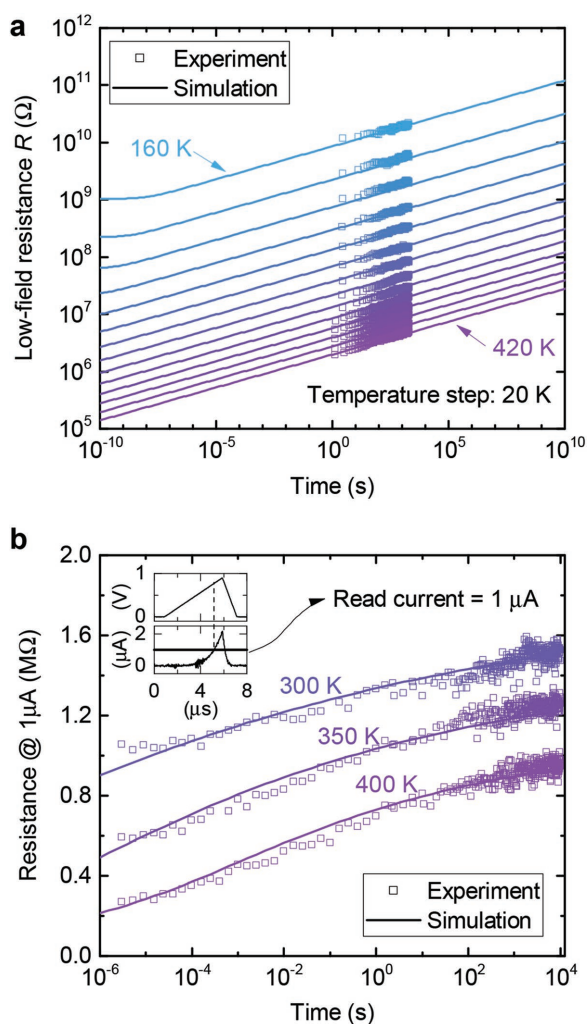
Figure 6. Constant temperature drift experiments. a) Low-field resistance drift measured at various temperatures from 160 to 420 K in steps of 20 K after the PCM cell has been programmed to a constant amorphous size. b) High-field resistance drift measured at 300, 350, and 400 K over 10 decades of elapsed time after RESET. The high-field resistance was defined as the resistance of the PCM cell at a fixed current of 1 \mu A. The inset shows a typical trace of the pulse used to measure the high-field resistance.
