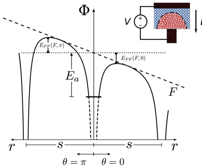
Figure 3. Electrical transport model The field dependence of the free carrier density is described by 3D Poole–Frenkel emission from a two-center Coulomb potential \Phi . The applied field F reduces the potential barrier in the direction \theta = 0 and increases it along \theta = \pi .
