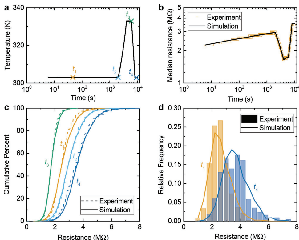
Figure 8. Array-level drift experiment High-field resistance measurements (0.62 V read voltage) were conducted on 4000 devices in the RESET state undergoing changes in the ambient temperature. The drift model was used to simulate the evolution of the high-field resistance on 1000 devices. In the simulation, normal distribution of drift variability and programmed state variability with 5% standard deviation were assumed. a) Temperature profile applied to the PCM chip. b) Experimental and simulated evolution of the median resistance. c) Experimental (dashed lines) and simulated (plain lines) cumulative resistance distributions at four instances in time. d), Experimental (bars) and simulated (plain lines) resistance histograms before and after annealing.
