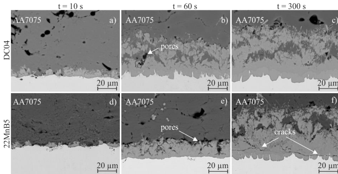
Figure 3. SEM images of the interface between AA7075 coating and steel DC04 after heat treatment at T = 550\text{ °C} for a) t = 10\text{ s} , b) t = 60\text{ s} , c) t = 300\text{ s} and between AA7075 coating and steel 22MnB5 after heat treatment at T = 550\text{ °C} for d) t = 10\text{ s} , e) t = 60\text{ s} , f) t = 300\text{ s}
