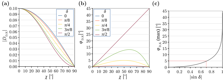
Fig. A.4: Diattenuation caused by anisotropic absorption (dichroism) of two in-plane crossing fiber bundles (see Fig. A.3) with dichroism D_K = 5\% , retardance \delta , and crossing angle \chi . The amplitude |D_{D,K}| and the phase \varphi_{D,K} of the transmitted light intensity profile I_D(\rho, \chi) (see Eq. (A.60)) were computed analytically using Eqs. (4.36) and (4.37): (a) |D_{D,K}| plotted against \chi for different \delta , (b) \varphi_{D,K} plotted against \chi for different \delta , (c) maximum \varphi_{D,K} plotted against the retardation |\sin \delta| . When the order of the fiber bundles in Fig. A.3 is reversed, the graphs for \varphi_{D,K} are mirrored about the x-axis.
