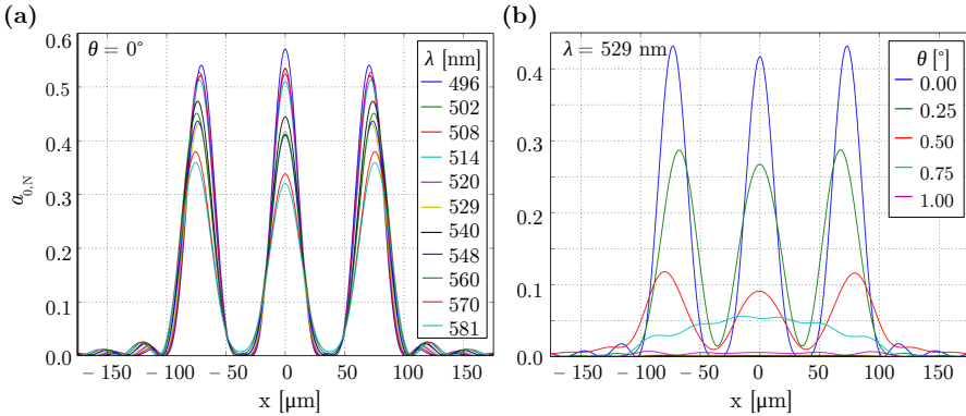
Fig. 10.11: Transmittance profiles obtained from 2D simulations of the USAF resolution target for the LAP (with line width l = 35.08\mu\text{m} ): (a) normally incident light ( \theta = 0^\circ ) with different wavelengths \lambda , (b) light with fixed wavelength ( \lambda = 529\text{ nm} ) and different angles of incidence \theta
