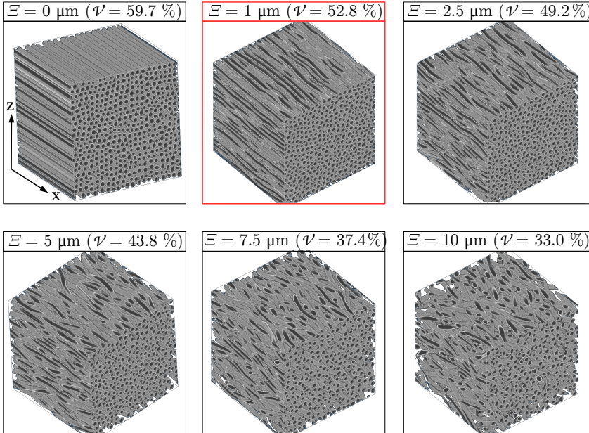
Fig. 10.20: Horizontal fiber bundle ( 30 \times 30 \times 30 \mu\text{m}^3 ) with fiber radii r \in [0.5, 0.8] \mu\text{m} and different fiber orientation distributions (i.e. different maximum displacements \Xi of fiber midpoints) generated by the VCS. The volume fraction \mathcal{V} of the fibers decreases with increasing \Xi . The red frame highlights the reference fiber bundle (cf. Fig. 10.18b).
