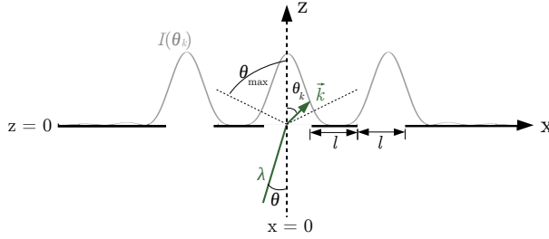
Fig. 10.12: 1D grating consisting of three slits with width and spacing l , representing the USAF resolution target for the LAP. The Fraunhofer diffraction pattern was computed for light with different angles of incidence \theta and different wavelengths \lambda . The numerical aperture of the imaging system (NA) was taken into account by computing the transmitted light intensity I(\theta_k) only from k -vectors with angles \theta_k \leq \theta_{\max} = \arcsin(\text{NA}) .
