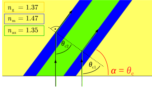
Fig. A.5: Schematic drawing of total internal reflection: Light under normal incidence is “guided” within the myelin layer (blue) when the inclination angle \alpha of the straight fiber becomes larger than the critical angle \theta_c of total internal reflection, which is defined by the refractive indices of myelin ( n_m ), axon ( n_{ax} ), and the surrounding glycerin solution ( n_g ).
