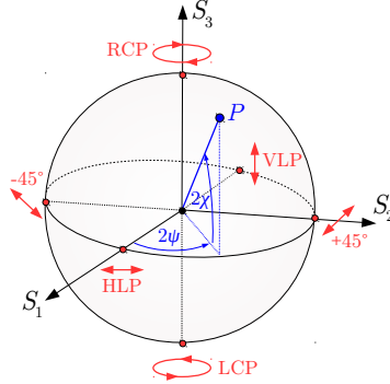
Fig. 2.4: Poincaré sphere used to represent polarized light (inspired by [87]): Every polarization state P is represented by a vector in Cartesian coordinates (S_1, S_2, S_3) or spherical coordinates (2\psi, 2\chi) . The length of the vector represents the degree of polarization p \leq 1 ( p = 0 corresponds to the origin and p = 1 to the surface of the sphere). Linear polarization states lie on the equator, circular polarization states at the poles, elliptical polarization states everywhere else on the surface (see Fig. 2.1 for the definition of polarization states).
