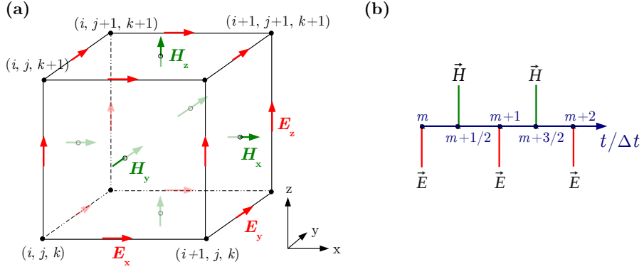
Fig. 6.1: (a) Unit cell of the cubic Yee grid: Each component of the magnetic field \vec{H} is surrounded by four components of the electric field \vec{E} and vice versa. (After: YEE [176] Fig. 1) (b) Illustration of the leapfrog time-stepping scheme. (After: WILTS [175] Fig. 1) (The figures have been published in MENZEL et al. (2016) [66] Fig. 3b.)
