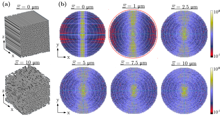
Fig. 11.6: (a) 3D views and (b) scattering patterns ( I_k ) for horizontal fiber bundles with different fiber orientation distributions (i. e. bundles generated with different maximum displacements \Xi in the VCS, cf. Fig. 10.20). The red frame highlights the scattering pattern of the reference fiber bundle (see Fig. 10.18b).
