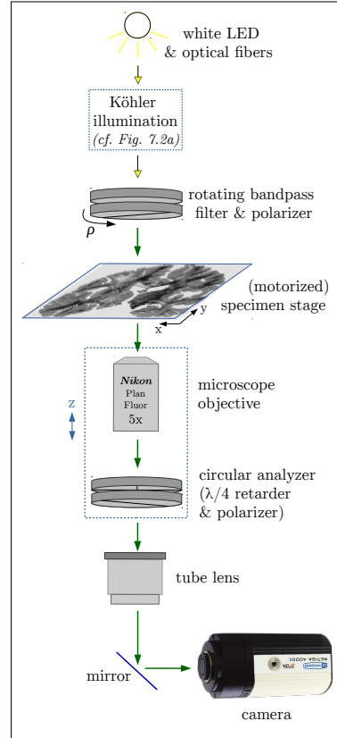
Fig. B.1: Schematic figure (not to scale) of the optical components incorporated in the PM
