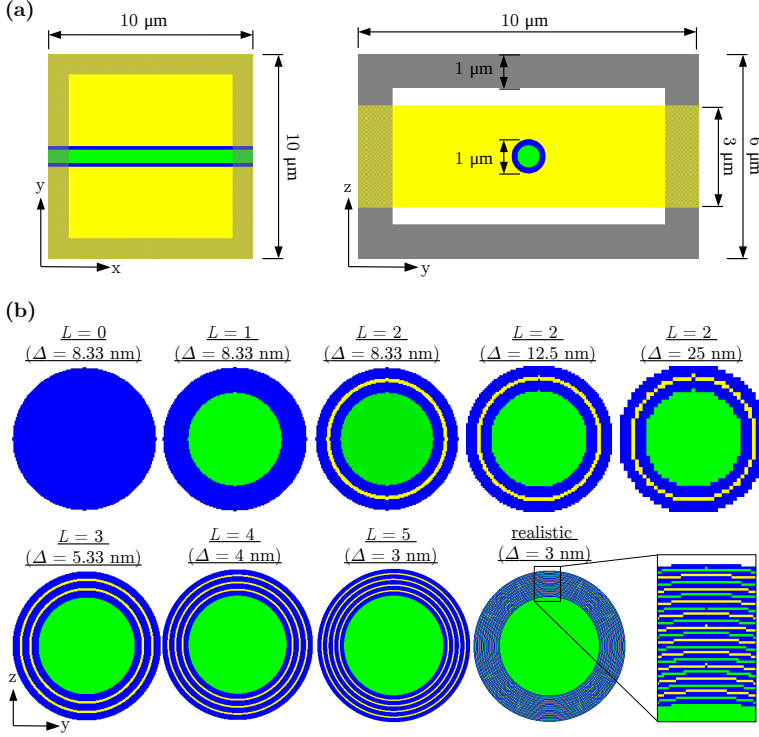
Fig. 10.30: Model of the myelin sheath for different numbers of myelin layers: (a) Dimensions of the simulation volume used to simulate a straight single fiber. (b) Cross-section through fibers with different numbers L of myelin layers and different Yee mesh sizes \Delta . All fibers were modeled with a diameter of 1\ \mu\text{m} , consisting of an inner axon (green) with a diameter of 0.65\ \mu\text{m} and a surrounding myelin sheath with a thickness of 0.175\ \mu\text{m} . The myelin sheath is composed of alternating layers of myelin (blue) and glycerin (yellow), the myelin layers are three times thicker than the glycerin layers (the glycerin layer thickness is defined by the number of myelin layers, see Eq. (10.46)). The realistic model of the myelin sheath contains 22 layers of 5\ \text{nm} thick cell membranes (blue), interrupted by 3\ \text{nm} thick alternating layers of cytoplasm (green) and glycerin solution (yellow), yielding a myelin sheath composed of 43 thin layers. The refractive indices are 1.35 for the axon/ cytoplasm (green), 1.37 for the glycerin solution (yellow), and 1.47 for the myelin layers (blue). A motivation of the myelin sheath model and the refractive indices can be found in Fig. 10.26. A similar figure has been published in MENZEL et al. (2018a) [67] Fig. 18a-b.
