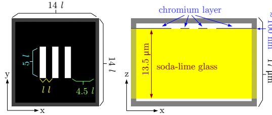
Fig. 10.4: Dimensions for the simulation model of the USAF target. The x- and y-dimensions of the simulation model scale according to the line width l , the dimensions in the z-direction remain unchanged. The simulation volume is surrounded by 1\text{ }\mu\text{m} thick UPML boundaries (gray).
