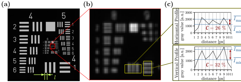
Fig. 7.5: USAF resolution target measured with the PM: (a,b) transmittance image, (c) horizontal and vertical line profiles evaluated for a line width l = 1.95 \mu\text{m} (group 8, element 1). The contrast \mathcal{C} of the lines was computed by averaging the local minima ( \overline{I_{\min}} ) and the local maxima ( \overline{I_{\max}} ) of the intensity profile, and using Eq. (7.4).
