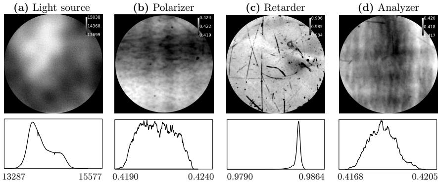
Fig. 7.7: Images and histograms of light source, polarizer, retarder, and analyzer. Note that the contrasts between images differ (the maximum measurable intensity values are depicted in white, the minimum values in black, respectively). The figure has been published in MENZEL et al. (2017) [3] Fig. 12.
