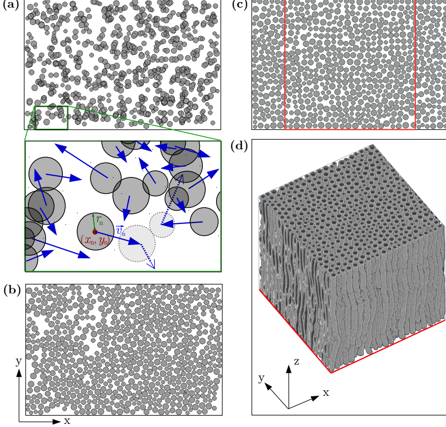
Fig. 6.2: Illustration of the Fiber Growing Algorithm: (a) A number of circles ( N = 700 ) with a user-defined distribution of radii (uniform distribution with r_n \in [0.5, 0.8] \mu\text{m} ) are randomly uniformly distributed in the xy-plane (in an area of 45 \times 30 \mu\text{m}^2 ). Every circle is initialized with a random speed \vec{v}_n ; the circles collide assuming elastic collision (see circles with dashed lines). (b) The circles move around until a solution is reached without overlapping circles in the xy-plane. (c) The previous step is repeated 250 times until the position of the circles is stored. (d) To generate a 3D fiber volume ( 30 \times 30 \times 30 \mu\text{m}^3 ), the position of the circles in the xy-plane (red square) is stored while incrementing the z-position by 1 \mu\text{m} per step.
