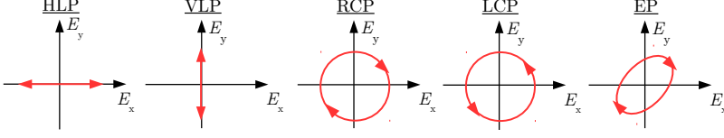
Fig. 2.1: Polarization states of light: horizontal/vertical linear polarization (HLP/VLP), right-/left-handed circular polarization (RCP/LCP), and elliptical polarization (EP). The figure shows the shape (in red) that \vec{E}(\vec{r} = 0, t) describes in the plane perpendicular to \vec{k} ( \vec{k} points out of the image plane, towards the observer).
