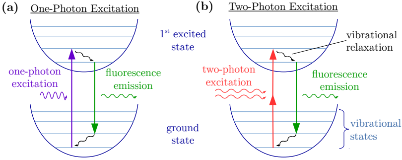
Fig. 5.3: Jablonski diagram of one-photon excitation (a) and two-photon excitation (b) (adapted from [166] Fig. 1)
