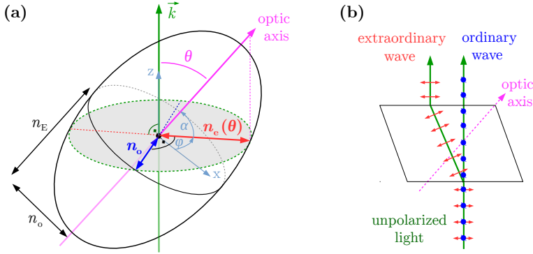
Fig. 2.3: (a) Rotational index ellipsoid of a positive uniaxial birefringent medium with n_E > n_o (inspired by [70] Fig. 8.31a). The intersection curve (green dotted line) between the ellipsoid and the plane of constant phase (gray) defines the refractive index that a light wave with wave vector \vec{k} experiences when it passes through the medium. The refractive index depends on the polarization, i.e. the direction of \vec{D} in the plane of constant phase: In case of the extraordinary wave (with refractive index n_e(\theta) ), \vec{D} lies parallel to the projection of the optic axis onto the plane of constant phase (red arrow). In case of the ordinary wave (with refractive index n_o ), \vec{D} lies perpendicularly to the optic axis and its projection (dark blue arrow). (b) Unpolarized light that passes through a birefringent medium is split into an ordinary wave (blue) and an extraordinary wave (red) with orthogonal linear polarization states. The ordinary wave obeys Snell's law, while the extraordinary wave is refracted even at normal incidence (adapted from [71] Fig. 8.19). The image plane shows the principal plane (spanned by the wave vector \vec{k} and the optic axis).
