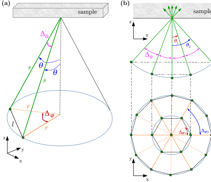
Fig. D.1: Uniform illumination of the light source: (a) 3D representation of two neighboring light rays (in green) with polar and azimuthal angular distances \Delta\theta and \Delta\varphi . (b) 2D representation of several neighboring light rays (top: xz -plane, bottom: xy -plane)
