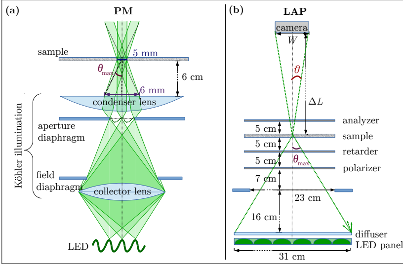
Fig. 7.2: Schematic figures (not to scale) illustrating the homogeneous illumination of the sample: (a) In the PM, a Köhler illumination is used to generate a homogeneous illumination of the sample. For reasons of simplification, the rotating bandpass filter and the polarizer in front of the sample (cf. Fig. B.1) are not included in the figure. (b) In the LAP, a diffuser plate is placed behind the LED panel to generate a homogeneous illumination of the sample. The homogeneous illumination in the PM and the LAP implies that the sample is illuminated under different angles. The maximum angle of incidence (with respect to the center of the sample) is denoted by \theta_{\max} , respectively. The refraction of light on plane surfaces (e.g. polarizing filters) has been neglected in the figures.
