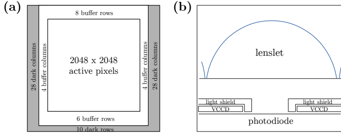
Fig. 7.4: CCD image sensor of the PM (Kodak KAI-04022-ABA): (a) device architecture (2048 × 2048 active pixels), (b) pixel architecture (square pixels with spherical microlens). The figures were drawn according to the data sheet from August 2015, Rev. 2, provided by Semiconductor Components Industries, LLC. 1
