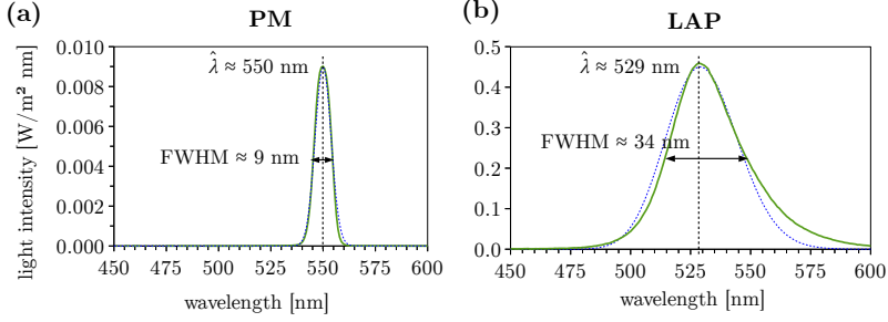
Fig. 7.1: The green curves show the wavelength spectra of the light sources (a) in the PM and (b) in the LAP (Adapted from RECKFORT [53]). The blue dotted curves show the wavelength spectra resulting from a Gaussian fit to the corresponding frequency spectrum, using [74] Eq. (6) with \lambda_0 \equiv \hat{\lambda} and \Delta\lambda \equiv \text{FWHM} .
