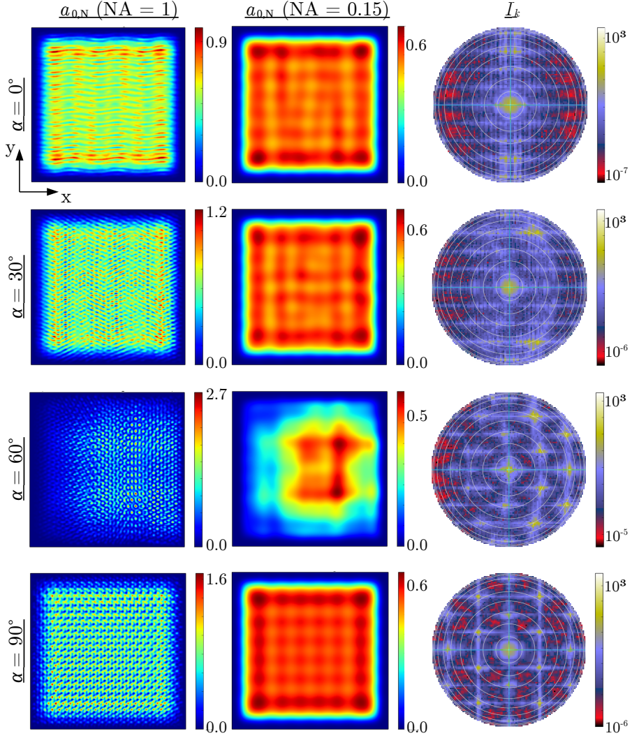
Fig. D.5: Transmittance images ( a_{0,N} ) and scattering patterns ( I_k ) computed from a simulated 3D-PLI measurement of a hexagonal grid of aligned helical fibers (see Sec. 10.2.1) for different fiber inclination angles \alpha . The transmittance images were computed for the microscope objective of the PM (numerical aperture: NA = 0.15, microlenses: r_0 = 0.665 \mu\text{m} ) and for the case without objective lens (NA = 1, r_0 = 0 \mu\text{m} ).
