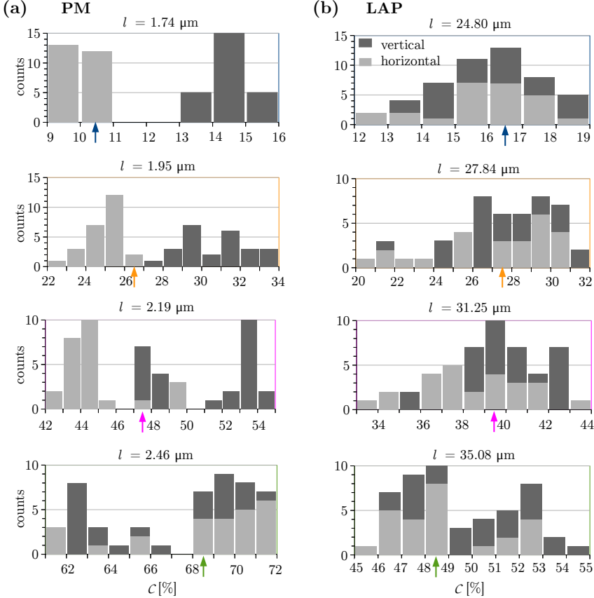
Fig. B.2: Histograms of the contrasts \mathcal{C} obtained from 25 measurements of the USAF resolution target with the PM and the LAP (see Sec. 7.1.4). The contrasts were computed for different line widths l from the horizontal and vertical line profiles of the transmittance images (cf. Fig. 7.5). The arrows mark the columns that contain the median contrast values \bar{\mathcal{C}} (cf. Fig. 7.6b).
