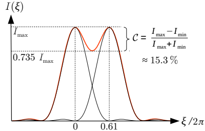
Fig. 2.2: Rayleigh criterion for two incoherent point sources with circular aperture
