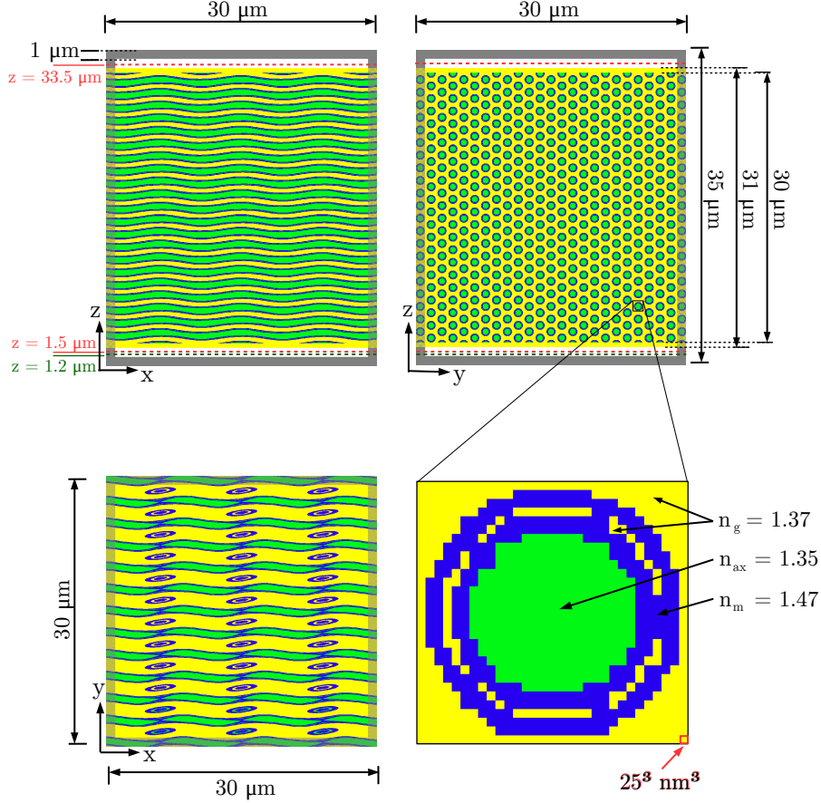
Fig. 10.27: Dimensions of the simulation box used for simulating the fiber configurations by TDME3D in Chaps. 11 and 12, shown exemplary for the hexagonal grid of aligned helical horizontal fibers (see Sec. 10.2.1). All fiber configurations were simulated in a volume of 30 \times 30 \times 30 \mu\text{m}^3 , surrounded by a medium with dimensions 30 \times 30 \times 31 \mu\text{m}^3 and a refractive index n_g = 1.37 (yellow). The sample was placed in a simulation box of 30 \times 30 \times 35 \mu\text{m}^3 , surrounded by 1 \mu\text{m} thick UPML boundaries (gray). The fibers were modeled with double myelin layers (see Fig. 10.26d), i.e. two myelin layers (blue, n_m = 1.47 ) with separating glycerin layer (yellow, n_g = 1.37 ) surrounding the inner axon (green, n_{ax} = 1.35 ). The Yee mesh size was chosen to be \Delta = 25 \text{ nm} for all simulations. The light source (green dashed line) was placed in front of the sample at position z = 1.2 \mu\text{m} . The detection planes which record the reflected and transmitted light waves (red dashed lines) were placed between light source and sample at position z = 1.5 \mu\text{m} , and behind the sample at position z = 33.5 \mu\text{m} .
