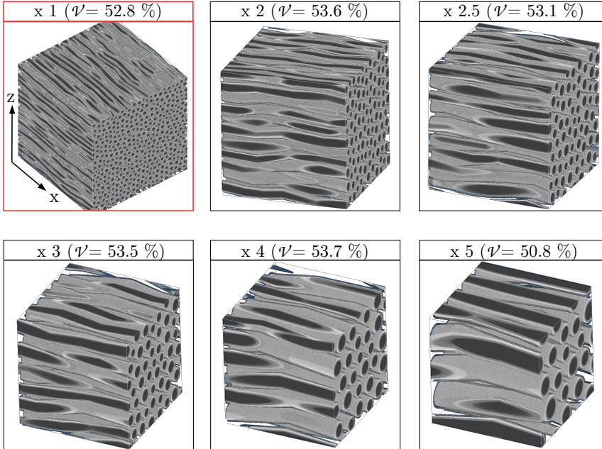
Fig. 10.24: Horizontal fiber bundle generated by the VCS with different scaling factors in a volume of 30 \times 30 \times 30 \mu\text{m}^3 . The volume fraction \mathcal{V} of the fibers is similar for scaling factors 1 to 4. For a scaling factor of 5, it is slightly smaller. The red frame highlights the reference fiber bundle without scaling (cf. Fig. 10.18b).
