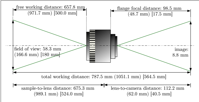
Fig. 7.3: Camera objective of the LAP (schematic system drawing, not to scale). The numbers have been computed with MachVis 5.0.6 (lens calculator for Qioptiq Machine Vision lenses) by specifying the field of view and selecting a 2/3 inch sensor, a C-mount adapter, and modular focus. The numbers without brackets refer to the camera objective with higher resolution ( Apo-Rodagon-N90 ), the numbers in brackets refer to the camera objectives with lower resolution (round brackets: Apo-Rodagon-N50 ; square brackets: Lametar 2.8/25 ). The flange focal distance refers to the distance from the mounting flange of the camera to the sensor plane.
