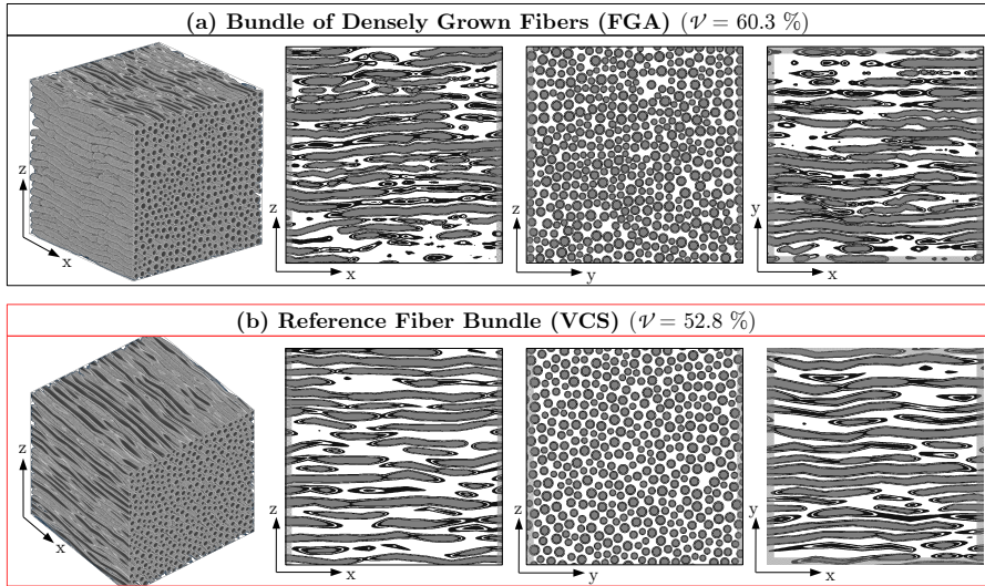
Fig. 10.18: 3D view and cross-sections through mid-planes for a horizontal fiber bundle: (a) bundle of densely grown fibers generated by the FGA, (b) reference fiber bundle generated by the VCS (see Sec. 10.2.3.1, with maximum displacement of fiber midpoints \Xi = 1 \mu\text{m} ). For both fiber bundles, 700 fibers with radii r \in [0.5, 0.8] \mu\text{m} were generated in a volume of 45 \times 30 \times 45 \mu\text{m}^3 and cropped to a volume of 30 \times 30 \times 30 \mu\text{m}^3 . Note that all fiber radii were reduced by 5% to prevent fibers from touching each other. In addition to the geometry, the volume fraction \mathcal{V} is given (i. e. the volume filled by fibers divided by the total volume).
