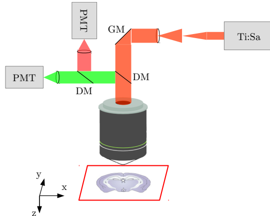
Fig. 5.4: Schematic drawing visualizing the TPFM measurement setup. The setup consists of a titanium-sapphire (Ti:Sa) laser, a pair of galvanometric mirrors (GM), dichroic mirrors (DM), photomultiplier tubes (PMT), a microscope objective, and a motorized specimen stage. (Courtesy of Irene Costantini)
