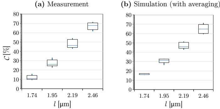
Fig. 10.9: Box-and-whisker diagrams for the contrast values of the USAF resolution target measured with the PM for different line widths l . The blue lines indicate the median contrast values, the boxes contain 25–75 % of the contrast values, the ends of the whiskers represent the minimum and maximum contrast values: (a) measured contrast values (see Tab. 10.2 in italics), (b) simulated contrast values (the downsampling was performed by applying a moving average over an area of 2.66 \times 2.66 \mu\text{m}^2 on the transmittance images and rasterizing with spacing \Delta x = 1.33 \mu\text{m} along the x- and y-axes, see Tab. 10.2 in bold).
