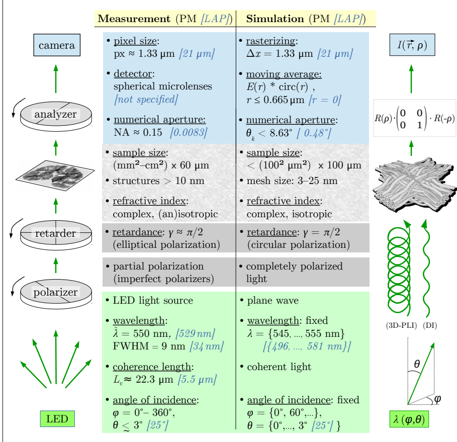
Fig. 10.1: Model of the optical systems (PM/LAP): On the left-hand side, the optical components of the polarimeters are characterized (cf. Tab. 7.3): light source (green), polarizer/retarder (dark gray), sample (light gray), objective lens/detector (blue). The figure shows the setup for the 3D-PLI measurement (for the DI measurement, retarder and analyzer are removed). The table and figure on the right-hand side show how the optical elements were modeled in the FDTD simulations: The incoherent and diffuse light source (LED) was modeled by performing several simulation runs with plane waves that have different wavelengths ( \lambda ) and angles of incidence ( \varphi, \theta ). The modeled light source emits coherent light that is circularly or linearly polarized depending on the type of measurement (3D-PLI or DI). The tissue sample was represented by an artificial fiber architecture, the rotating analyzer by a rotated Jones matrix. A similar figure has been published in MENZEL et al. (2018a) [67] Fig. 11.
