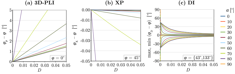
Fig. 9.1: Predicted impact of the non-ideal polarization properties of the LAP (Eqs. (7.5) and (7.6)) on the fiber direction angles \{\varphi_P, \varphi_X, \varphi_D\} obtained from 3D-PLI, XP, and DI measurements (see Secs. 4.4.1 to 4.4.3). The maximum difference between \{\varphi_P, \varphi_X, \varphi_D\} and the actual fiber direction angle \varphi is plotted against the tissue diattenuation D \geq 0 for different fiber inclinations \alpha : (a) As the curves for different \varphi look identical, the curves are only shown for an assumed fiber direction \varphi = 0^\circ . (b) The curves are shown for \varphi = 45^\circ for which |\varphi_X - \varphi| becomes maximal. (c) The curves are shown for \varphi = 43^\circ ( 133^\circ ) for which the difference between \varphi_D and \varphi becomes maximal (minimal). For D < 0 , the curves are rotated 180^\circ around the origin, the curves in Fig. c obtain an additional shift by +90^\circ along the y-axis. The figures are adapted from MENZEL et al. (2017) [3] Figs. 3 to 5.
