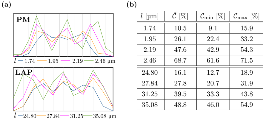
Fig. 7.6: Horizontal and vertical line profiles evaluated from 25 measurements of a USAF resolution target with the PM and the LAP (with Apo-Rodagon-N90 objective) for different line widths l : (a) Line profiles belonging to the median contrast values \bar{C} . (b) Median, minimum and maximum contrast values of all evaluated line profiles (horizontal and vertical).
