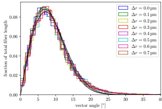
Fig. 10.23: Fiber orientation dispersion for bundles with an average fiber radius of 0.65 \mu\text{m} and different fiber radius distributions ( \Delta r = r_{\text{max}} - r_{\text{min}} , cf. Fig. 10.22). The dashed lines show the fitted Rayleigh distributions with mode \sigma = 6.7\text{--}7.1^\circ . The relative error of all fitted mode values is mostly below 0.6%.
