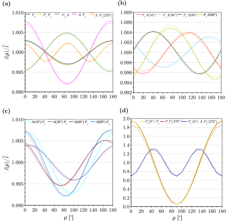
Fig. B.3: Normalized light intensity profiles: The solid curves show the profiles obtained from the filter measurements described in Tab. B.1. The dashed curves show the modeled profiles computed from the polarization parameters defined in Tab. B.2, first row. The angle \rho is the rotation angle of the rotating filters in the measurement. The figure has been published in MENZEL et al. (2017) [3] Fig. 13.
