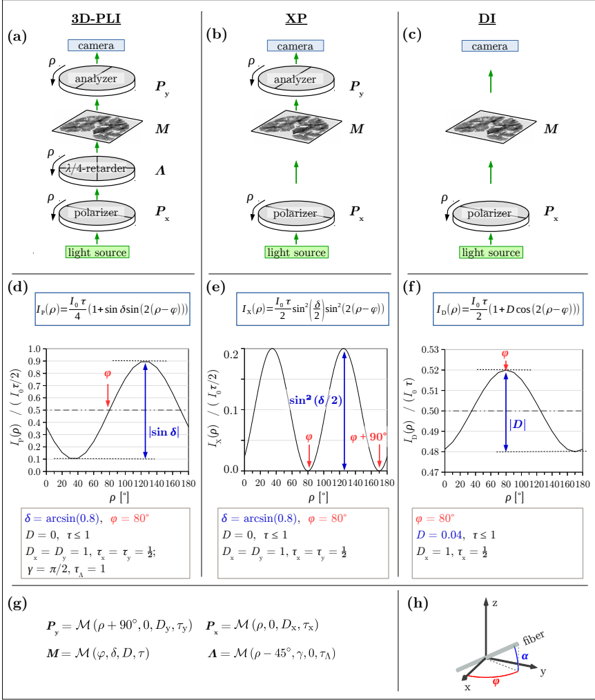
Fig. 4.4: (a-c) Schematic of the setups for the 3D-PLI, XP, and DI measurements for the LAP: For the 3D-PLI measurement (a), the brain section is placed between a pair of crossed linear polarizers (polarizer/analyzer) and a quarter-wave retarder. For the XP measurement (b), only the crossed linear polarizers are used while for the DI measurement (c) only the polarizer is used. For all measurement setups, the employed filters are rotated simultaneously by discrete rotation angles \rho around the stationary specimen. (d-f) Analytically computed normalized light intensity profiles for the different measurement setups, assuming a retardance \delta = \arcsin(0.8) , a fiber direction \varphi = 80^\circ , and ideal filter properties ( D_x = D_y = 1 , \tau_x = \tau_y = 1/2 ; \gamma = \pi/2 , \tau_A = 1 ): For the 3D-PLI and XP measurements, the diattenuation of the brain tissue was neglected ( D = 0 ). For the DI measurement, the tissue diattenuation was assumed to be D = 4\% . The phase \varphi of the intensity profiles (in red) is a measure for the in-plane fiber direction, while the amplitude (in blue) is correlated to the out-of-plane fiber inclination. (g) The transmitted light intensities are calculated using the Müller-Stokes calculus, in which each optical element is represented by a Müller matrix \mathcal{M}(\xi, \delta, D, \tau) as defined in Eqs. (2.56) to (2.58). (h) The three-dimensional fiber orientation is defined in spherical coordinates by the in-plane direction angle \varphi and the out-of-plane inclination angle \alpha . A similar figure has been published in MENZEL et al. (2017) [3] Fig. 2.
