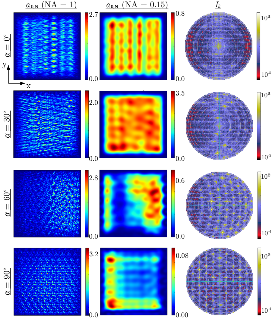
Fig. D.7: Transmittance images ( a_{0,N} ) and scattering patterns ( I_k ) computed from a simulated 3D-PLI measurement of a hexagonal grid of unaligned helical fibers with different strides (see Sec. 10.2.1) for different fiber inclination angles \alpha . The transmittance images were computed for the microscope objective of the PM (numerical aperture: NA = 0.15, microlenses: r_0 = 0.665 \mu\text{m} ) and for the case without objective lens (NA = 1, r_0 = 0 \mu\text{m} ).
