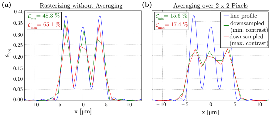
Fig. 10.8: Downsampled line profiles of the USAF resolution target (with line width l = 1.74 \mu\text{m} ) simulated for the optics of the PM. The blue curves show the line profiles of the original transmittance images without downsampling (cf. Fig. 10.7b). The green (red) curves show the downsampled line profiles with minimum (maximum) contrast, according to Eq. (7.4). (a) The downsampling was performed by rasterizing the transmittance image with spacing \Delta x = 1.33 \mu\text{m} along the x - and y -axes. (b) The downsampling was performed by applying a moving average over 2.66 \times 2.66 \mu\text{m}^2 before rasterizing the resulting image with spacing 1.33 \mu\text{m} .
