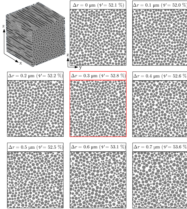
Fig. 10.22: Horizontal fiber bundle ( 30 \times 30 \times 30 \mu\text{m}^3 ) with an average fiber radius of 0.65 \mu\text{m} and different fiber radius distributions ( \Delta r = r_{\text{max}} - r_{\text{min}} ) generated by the VCS. The maximum displacement of fiber midpoints is \Xi = 1 \mu\text{m} . The figure shows cross-sections through the yz -mid-plane for different fiber radius distributions. The red frame highlights the reference fiber bundle (cf. Fig. 10.18b), which is also shown as 3D image. The volume fraction \mathcal{V} of the fibers is similar for different \Delta r .
