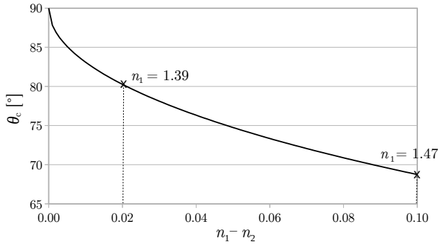
Fig. A.6: Critical angle of total internal reflection \theta_c plotted against the difference in refractive indices ( n_1 - n_2 ), where n_2 = n_g = 1.37 belongs to the medium with lower refractive index (surrounding glycerin solution) and n_1 to the medium with higher refractive index (myelin)
