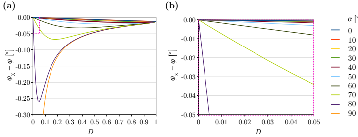
Fig. C.2: Predicted impact of the non-ideal polarization properties of the LAP (specified in Eqs. (7.5) and (7.6)) on the direction angle \varphi_X derived from an XP measurement (see Sec. 4.4.2). The plots show the difference between \varphi_X and the actual fiber direction \varphi plotted against the tissue diattenuation D \geq 0 for different fiber inclination angles \alpha . The actual fiber direction was set to \varphi = 45^\circ such that |\varphi_X - \varphi| becomes maximal. (a) Difference between \varphi_X and \varphi . (b) Enlarged view of (a) for D \leq 5\% . For D < 0 , the curves are rotated 180^\circ around the origin. The figure has been published in MENZEL et al. (2017) [3] Fig. 4.
