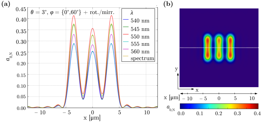
Fig. 10.7: USAF resolution target with line width l = 1.74 \mu\text{m} (cf. Fig. 10.4) simulated for the optics of the PM and diffuse light. The transmittance images were computed from three simulation runs with different angles of incidence ( \{\theta = 0^\circ\} , \{\theta = 3^\circ, \varphi = 0^\circ\} , \{\theta = 3^\circ, 60^\circ\} ), and by 180^\circ -rotation or flipping of the simulated transmittance images: (a) line profiles of the resulting transmittance images for different wavelengths \lambda , (b) transmittance image obtained from the weighted sum over all wavelengths (according to Fig. 10.5b). The corresponding line profile (white dashed line) is shown as yellow curve in subfigure (a).
