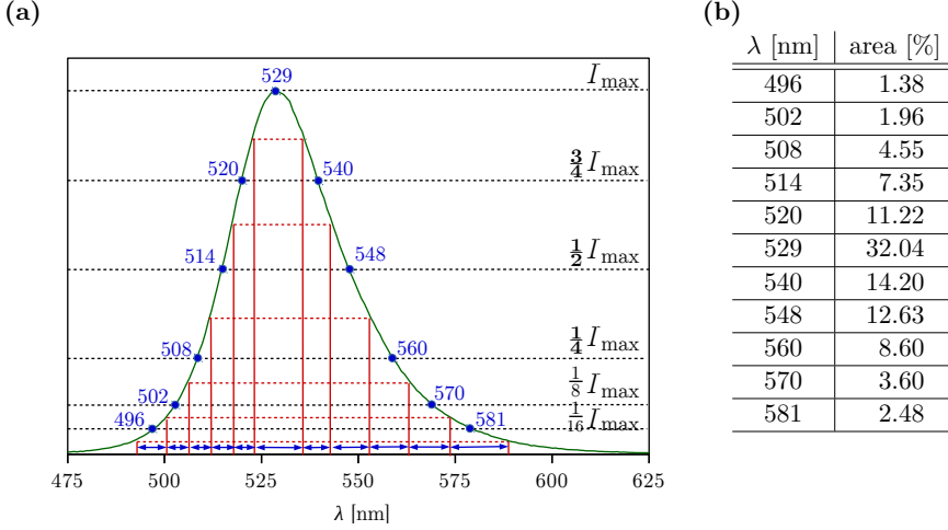
Fig. 10.10: (a) The wavelength spectrum of the LAP light source (see Fig. 7.1b) is less symmetric than the wavelength spectrum of the PM. Therefore, the spectrum was not sampled in equidistant steps, but with respect to the maximum intensity I_{\max} of the peak wavelength. For this purpose, the wavelengths with intensities \{1, 3/4, 1/2, 1/4, 1/8, 1/16\} I_{\max} were determined (blue numbers) and the wavelengths belonging to half of the intensity steps (red lines) were used to define borders around these wavelengths (blue arrows). The intensity steps were chosen such that the resulting wavelengths differ by 6–12 nm. The corresponding areas under the curve were used to compute the contribution of these wavelengths to the spectrum. (b) The table lists the fractions of the total intensity for these wavelengths, which were used to compute the weighted sum of transmittance images to model the wavelength spectrum of the LAP light source.
