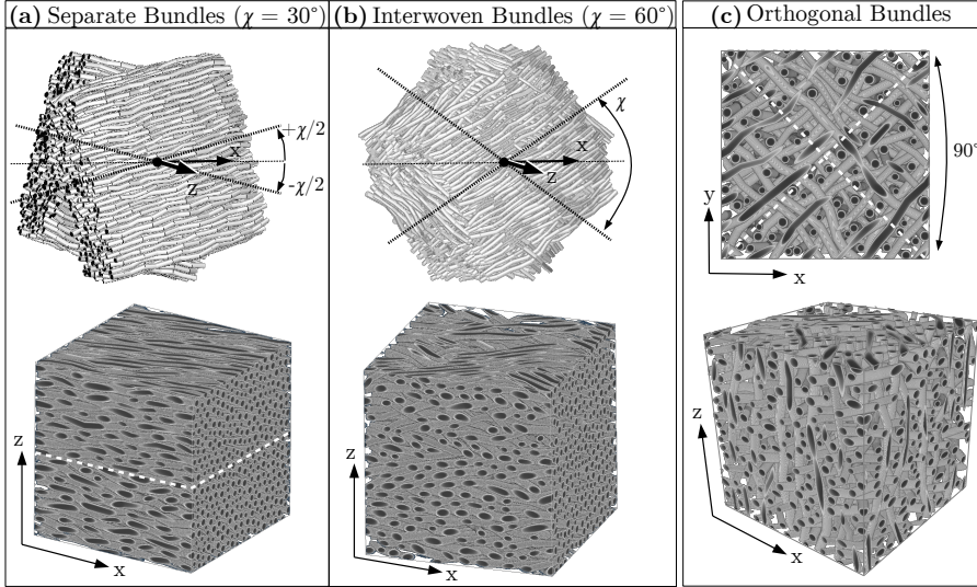
Fig. 10.25: (a-b) Separate and interwoven fiber bundles with crossing angle \chi : The upper figures show the bundles generated by the VCS. The lower figures show the bundles after being cropped to a volume of 30 \times 30 \times 30 \mu\text{m}^3 . The white dotted line indicates the border between the upper and lower bundle of the separate crossing fibers. For \chi = 0^\circ , the bundles correspond to the reference fiber bundle (cf. Fig. 10.18b). (c) Three mutually orthogonal, interwoven fiber bundles generated by the VCS and cropped to a volume of 30 \times 30 \times 30 \mu\text{m}^3 . The white dotted lines indicate the main directions of the two horizontal fiber bundles in the xy-plane, the third fiber bundle is oriented in the z-direction. All fibers were generated with radii r \in [0.5, 0.8] \mu\text{m} and a maximum displacement of fiber midpoints \Xi = 1 \mu\text{m} . The figure has been published in MENZEL et al. (2018a) [67] Fig. 15.
