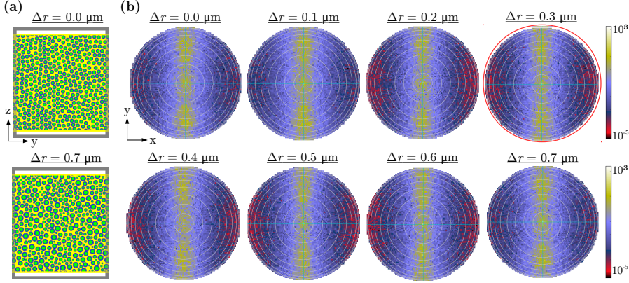
Fig. 11.8: (a) Cross-sections through yz-mid-plane and (b) scattering patterns ( I_k ) for horizontal fiber bundles with equal average fiber radius ( r_{\text{avg}} = 0.65 \mu\text{m} ) and different fiber radius distributions \Delta r = r_{\text{max}} - r_{\text{min}} (see Fig. 10.22). The red frame highlights the scattering pattern of the reference fiber bundle (see Fig. 10.18b).
