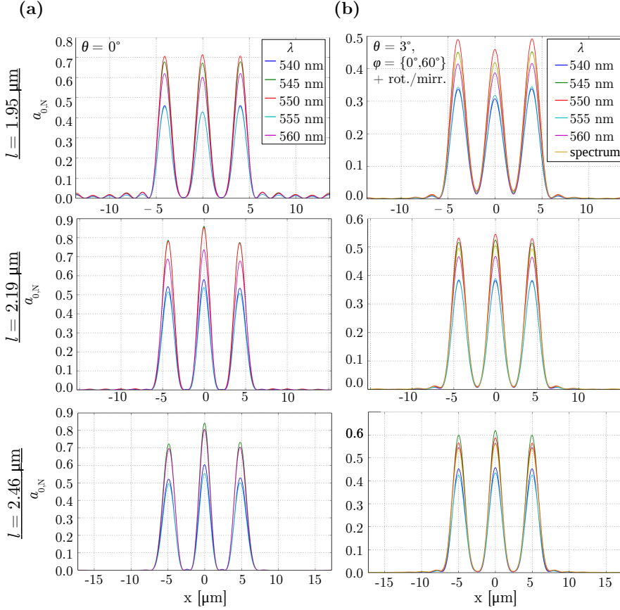
Fig. D.3: Line profiles of the USAF resolution target obtained from 3D-PLI simulations with line widths l = \{1.95, 2.19, 2.46\} \mu\text{m} (cf. Fig. 10.4) for the optics of the PM. The line profiles show the middle pixel in the y-direction evaluated along the x-direction of the resulting transmittance images: (a) normally incident light with different wavelengths \lambda , (b) diffuse light with different wavelengths. The transmittance images for diffuse light were computed from three simulation runs with different angles of incidence ( \{\theta = 0^\circ\} , \{\theta = 3^\circ, \varphi = 0^\circ\} , \{\theta = 3^\circ, \varphi = 60^\circ\} ), and by 180°-rotation or flipping of the simulated transmittance images. The yellow line profile was obtained from the weighted sum over the wavelength spectrum of the PM light source, according to Fig. 10.5b.
