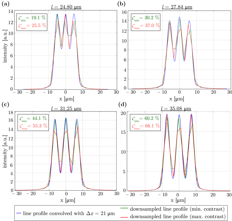
Fig. 10.14: Downsampled transmittance profiles of the USAF resolution target for different line widths l computed analytically from the Fraunhofer diffraction pattern of a 1D grating considering the optics of the LAP: The blue lines show the profiles after convolution with a rectangle function of width \Delta x = 21 \mu\text{m} , the green (red) lines show the downsampled profiles with minimum (maximum) contrast values. The contrasts \mathcal{C} were computed by averaging the local minima and maxima of the downsampled profiles and using Eq. (7.4).
