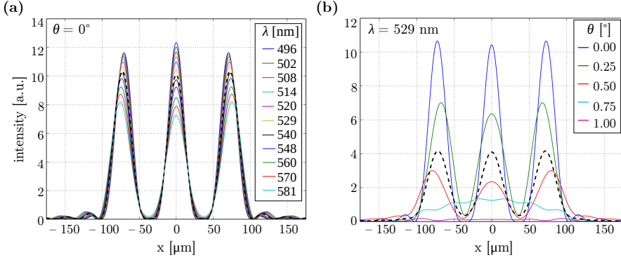
Fig. 10.13: Analytically computed transmittance profiles for the USAF resolution target of the LAP with line width l = 35.08 \mu\text{m} (Fraunhofer diffraction pattern of a 1D grating, see Appx. D.7): (a) normally incident light ( \theta = 0^\circ ) with different wavelengths \lambda , (b) light with fixed wavelength ( \lambda = 529 \text{ nm} ) and different angles of incidence \theta . The black dashed lines show the transmittance profiles obtained from the weighted sum over different wavelengths (according to Fig. 10.10b) and the weighted sum over different angles of incidence (same weighting for equidistant angles), respectively.
