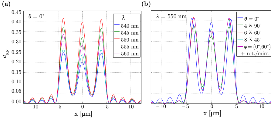
Fig. 10.6: Line profiles of the USAF target with line width l = 1.74 \mu\text{m} (cf. Fig. 10.4) simulated for the optics of the PM. The line profiles show the middle pixel in the y-direction evaluated along the x-direction of the resulting transmittance images: (a) normally incident light with different wavelengths, (b) diffuse light with different angles of incidence and fixed wavelength ( \lambda = 550 nm). The line profiles for diffuse light were generated by computing the weighted sum of the transmittance images obtained from several simulation runs with different angles of incidence, according to Eqs. (10.1) to (10.3). The notation \eta \times \Delta\varphi indicates that the transmittance image was computed from the simulation runs: \{\theta = 0^\circ\} , \{\theta = 3^\circ, \varphi = \eta \times \Delta\varphi\} . While the first line profiles were generated from a complete range of azimuthal angles ( \varphi \in [0^\circ, 360^\circ) ), the line profile in magenta was generated from only three simulation runs: \{\theta = 0^\circ\} , \{\theta = 3^\circ, \varphi = 0^\circ\} , and \{\theta = 3^\circ, \varphi = 60^\circ\} . The missing \varphi -angles were taken into account by rotating the resulting transmittance images by 180^\circ or by flipping the images with respect to the x- or y-axes.
