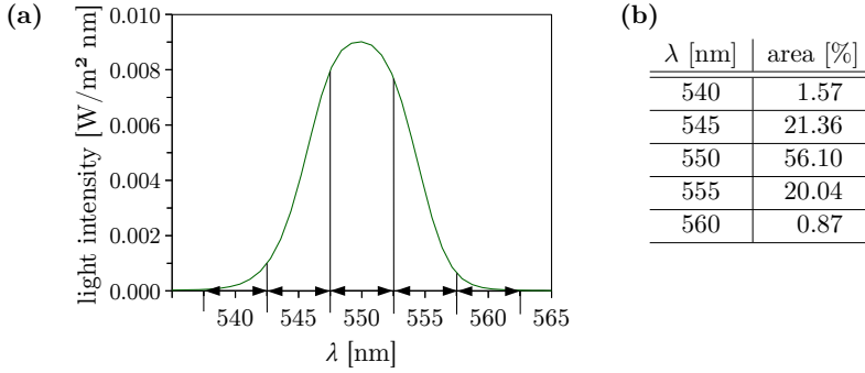
Fig. 10.5: Modeling the wavelength spectrum of the PM light source (cf. Fig. 7.1a): (a) The wavelength spectrum was sampled in steps of 5 nm. The area under the curve belonging to \lambda = \{540, 545, 550, 555, 560\} \text{ nm} was used to compute the contribution of these wavelengths to the spectrum. (b) The table lists the fractions of the total intensity for these wavelengths, which were used to compute the weighted sum of transmittance images representing the wavelength spectrum of the PM.
