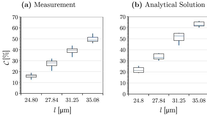
Fig. 10.15: Box-and-whisker diagrams for the contrast values of the USAF resolution target measured with the LAP for different line widths l . The blue lines indicate the median contrast values, the boxes contain 25–75 % of the contrast values, the ends of the whiskers represent the minimum and maximum contrast values: (a) measured contrast values (see Tab. 10.3 in italics), (b) analytically computed contrast values (see Tab. 10.3 in bold).
