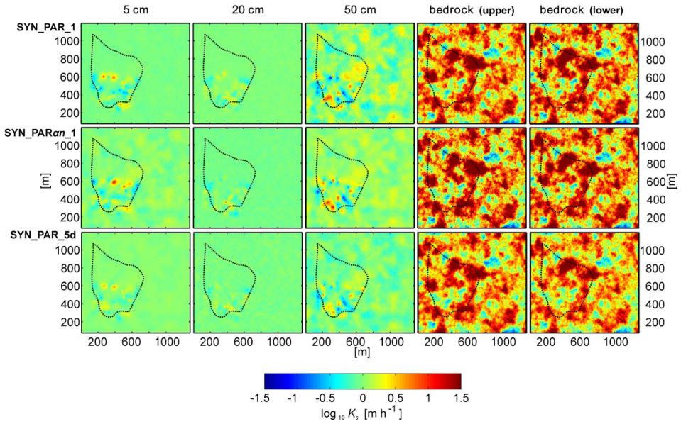
Figure 5.13: The ensemble averaged perturbation applied to the hydraulic conductivity field ( \log_{10}K_s ) during data assimilation for different synthetic simulation scenarios: Indicated are results for the soil layers at 5, 20, and 50 cm depth as well as the upper and lower bedrock layer. The dashed line marks the test site borders within the model domain.
