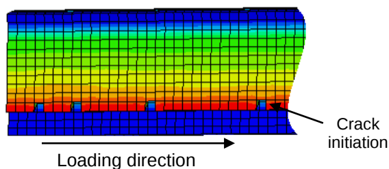
Figure 9. The view of EFTT specimen along the cut edge implies that the cracks initiated at the transition part from the fracture to the burr during the subsequent tensile test.
