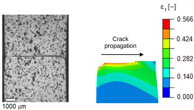
Figure 9. The view of EFTT specimen along the cut edge implies that the cracks initiated at the transition part from the fracture to the burr during the subsequent tensile test.
