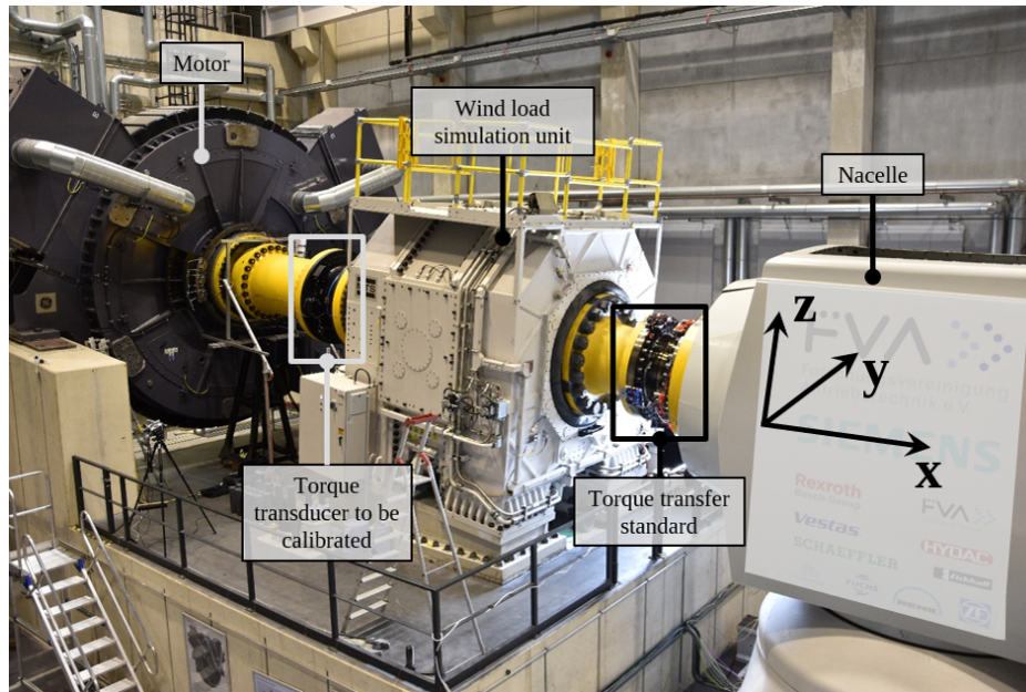
Figure 1. 5 MN m TTS, including its data acquisition system (DAQ) and telemetry system, mounted at the rotor hub flange of the wind turbine under test on the WTTB of the Center for Wind Power Drives at RWTH Aachen (edited from Weidinger et al., 2018a).
