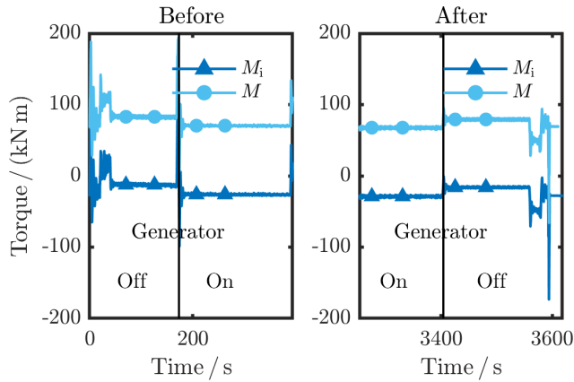
Figure 4. Zero signal determination under constant minimum rotation before and after each load cycle.
