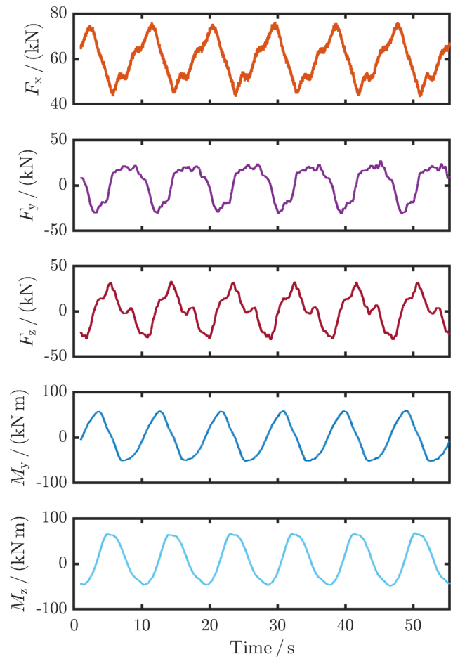
Figure 8. Additional multi-component loads during the calibration measurements due to the inaccuracy of the control system of the WTTB.
