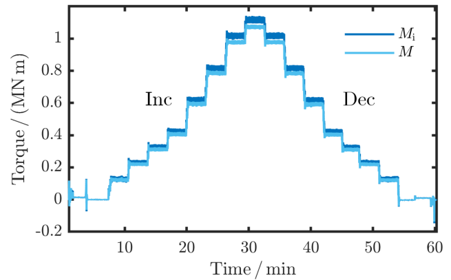
Figure 5. Tared measurement data of a load cycle with stepwise increasing (inc) and decreasing (dec) torque from 0 MN m up to 1.1 MN m.
