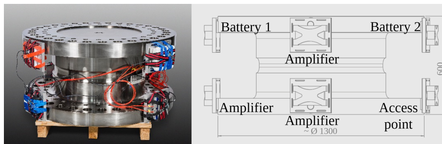
Figure 2. 5 MN m TTS equipped with a self-sufficient DAQ, and a telemetry system to transmit the measurement data in time.
