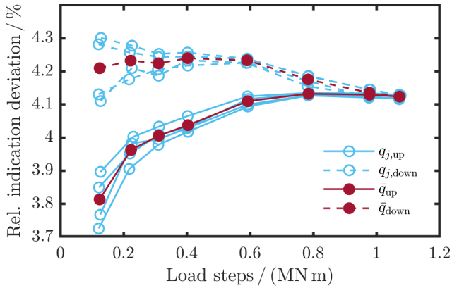
Figure 6. Relative indication deviation of the torque transducer in the WTTB as the result of the torque calibration under a constant rotation of n = 6.5 \text{ min}^{-1} .
