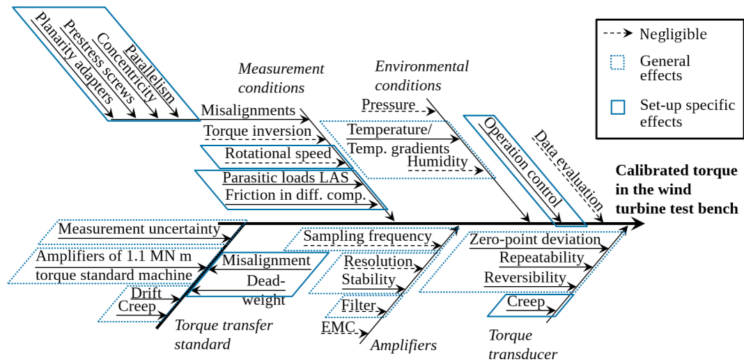
Figure 7. Ishikawa diagram listing the influences on the calibrated torque in the WTTB with the present set-up.
