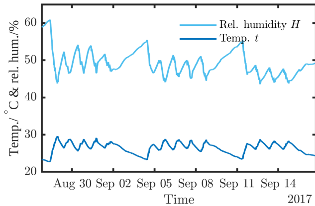
Figure 9. Temperature and humidity in the TTS during the torque calibration of the WTTB.
