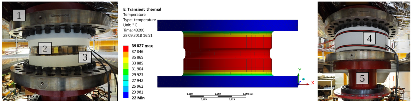
Figure 3. Heat blanket (3) around the 5 MN m TTS (1), which is installed in the 1.1 MN m torque standard machine (5) taped with five Pt100 sensors (2), and isolated by Basotect foam (4).
