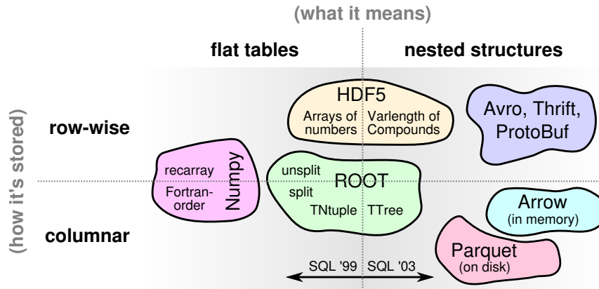
Figure 1. Existing data-formats used by ML communities.
