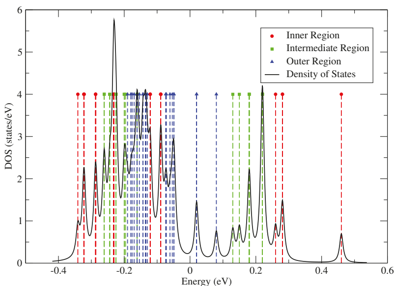
Figure 4. Each vertical line corresponds to one data point (due to symmetry, some points overlap). The colors correspond to the distances from the dislocation core, measured by the radius R . The red circles correspond to the 24 points closest to the dislocation core ( R < 2.87 \text{ \AA} ), the green squares are in the “intermediate range” ( 2.87 \text{ \AA} < R < 4.04 \text{ \AA} ), with the blue points belong are the outermost 24 points. The density of states (DOS) curve is generated by broadening the delta functions by a Lorentzian function of width k_B T/2 ( T = 300 \text{ K} ), with the integral under the DOS curve being normalised to 1.
