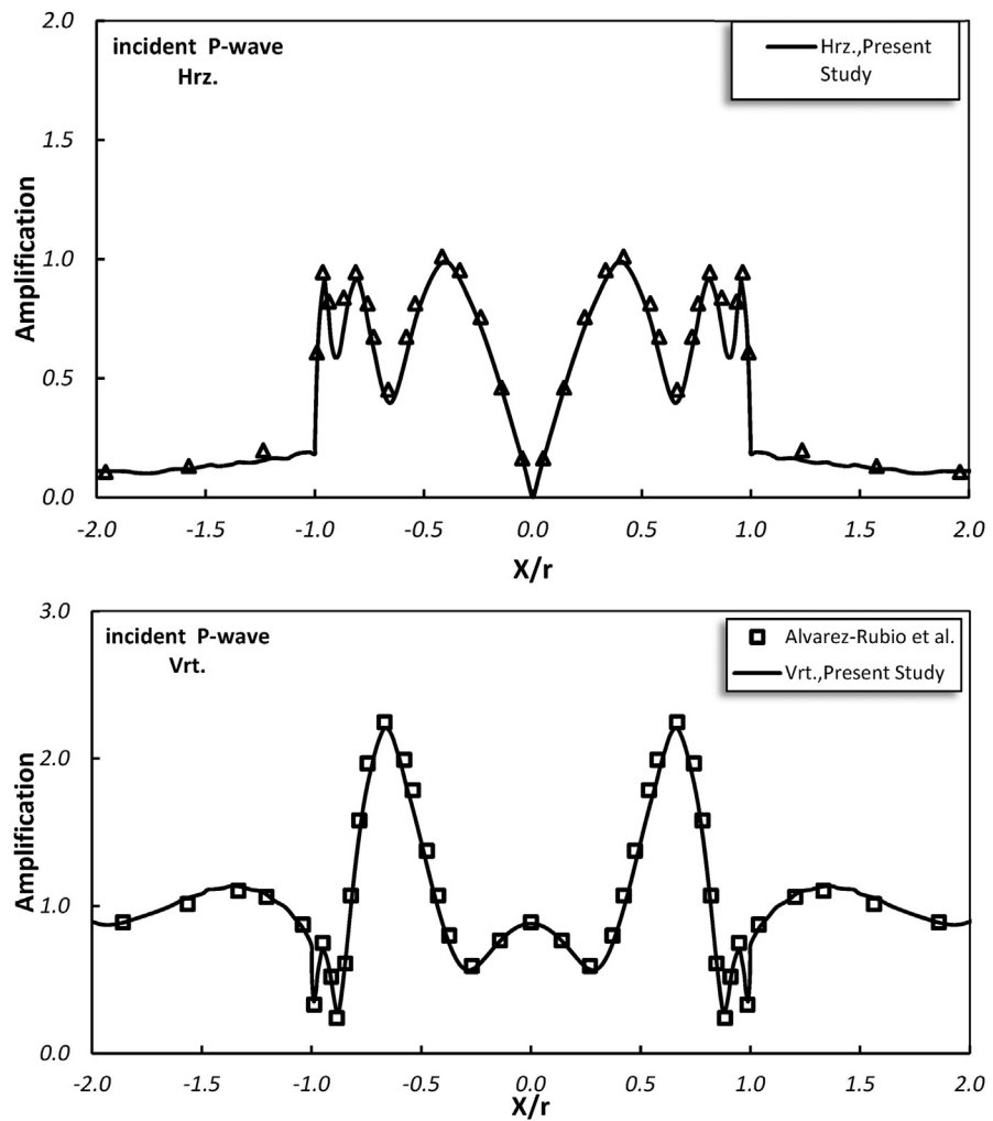
Fig. 6. Amplification of surface displacements for a semi-elliptical hill in the case of an incident P wave and \Omega = 1.5 . (The symbols “Hrz” and “Vrt” represent the horizontal and vertical components of amplification, respectively.)
