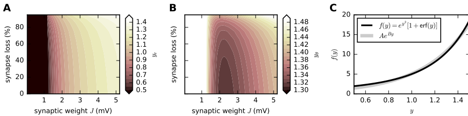
Figure 4.9: Approximation of f(y) = e^{y^2}[1 + \operatorname{erf}(y)] by an exponential function. A,B) Dependence of y_{ri} (A) and y_{\theta i} (B) on the synaptic reference weight J and the degree of synapse loss in the presence of unlimited firing rate homeostasis (mean-field theory). C) Graph of f(y) = e^{y^2}[1 + \operatorname{erf}(y)] (black) and exponential function Ae^{By} (gray; A = 0.4 , B = 2.5 ) fitted to f(y) in interval y \in [0.5, 1.5] . Same parameters as in network simulations (see Sec. 4.5.1 and Sec. 4.5.2).
