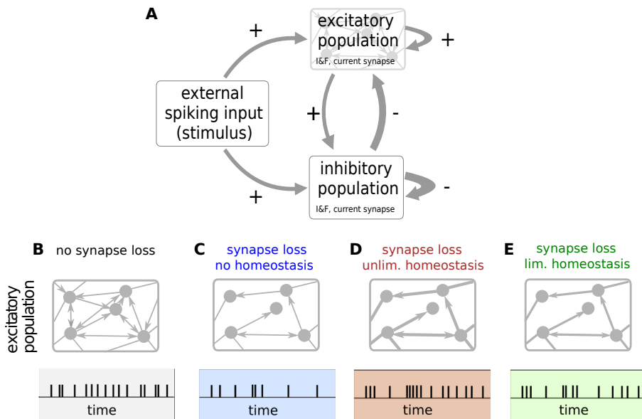
Figure 4.1: Sketch of the network model of Alzheimer's disease and homeostasis. A ) The network comprises two reciprocally and recurrently connected populations of excitatory (E) and inhibitory (I) integrate-and-fire neurons, excited by an external spiking input. Thickness of arrow indicates relative strength of the connection. In this study, Alzheimer's disease is modeled by removing connections between excitatory neurons (loss of EE synapses) and upscaling of the remaining EE synapses to maintain the average firing rate (firing rate homeostasis). B–E ) Sketch of EE connection density (number of arrows in upper panels), connection strength (thickness of arrows in upper panels) and resulting single-neuron spiking activity (lower panels). B ) Intact network (without synapse loss). C ) Synapse loss without homeostasis: removal of EE synapses and resulting reduction in firing rate. D ) Synapse loss with unlimited homeostasis: removal of EE synapses and increase in strength of remaining EE synapses to maintain the average firing rate. Synaptic weights are allowed to grow without bounds. E ) Synapse loss with limited homeostasis: removal of EE synapses and bounded increase in strength of remaining EE synapses. Here, synaptic weights cannot exceed 120% of their reference weight. The firing rate is therefore only partially recovered. For a complete description and parameter specification of the network model, see Sec. 4.4.1 and Supplementary Material (Sec. 4.5.1, Sec. 4.5.2).
