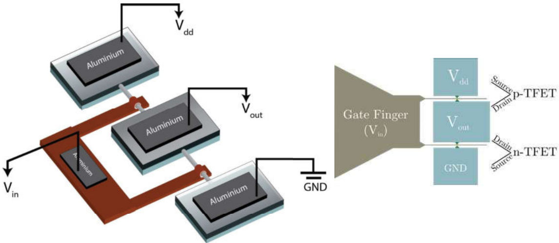
Figure 4.3: Schematics of single NW sSi GAA CTFET inverter with both transistors on the same mesa. Source and drain of n-TFET and p-TFET and their corresponding bias mode is specified.
