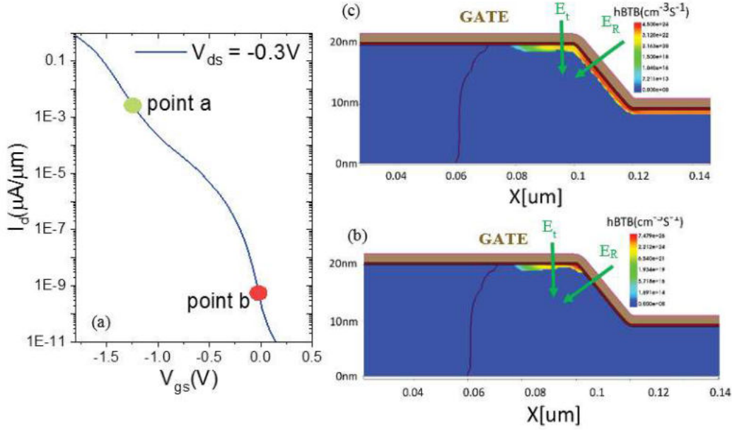
Figure 5.6: (a) Simulated transfer characteristics of the fabricated device at V_{ds} = -0.3\text{V} . (b), (c) show zoomed in contour of the device for different V_{gs} . Source is on the right side, while drain is on the left and gate extends all over the top section of the device. (b) Contour of BTB hole generation at V_{gs} = -0.1\text{V} shows that line-tunneling first occurs at the corner due to the high fringing field. (c) BTBT generation of carriers at V_{gs} = -1\text{V} shows that the hump in the characteristics is due to the late start of line-tunneling in the thinner area of source.
