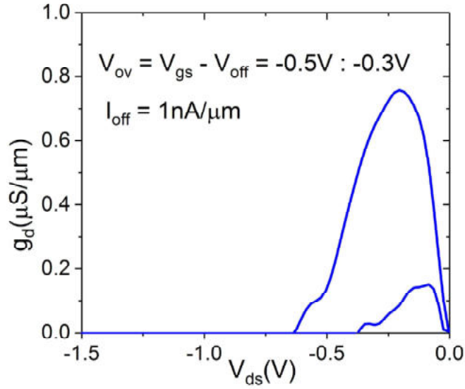
Figure 5.13: Extracted output conductance g_d from the output characteristics of device T1. g_d rapidly decreases to small values, indicating good current saturation.
