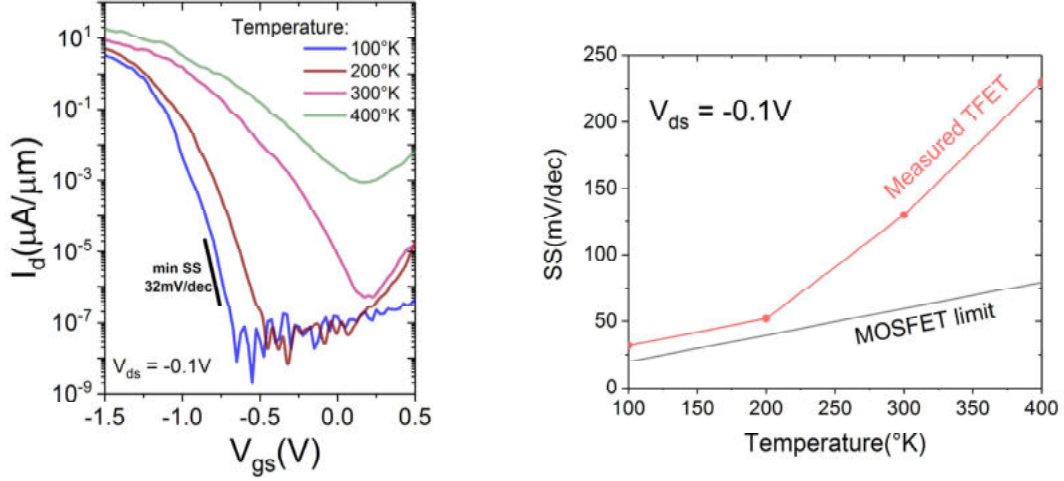
Figure 3.21: Transfer characteristics of silicon GAA single NW p-TFET with NW dimension of 35nmx10nm and gate length of 350nm measured for temperatures ranging from 400°K to 100°K (b) Measured minimum SS of the p-TFET as a function of T temperature. The theoretical limit of SS for MOSFETs is also shown for comparison.
