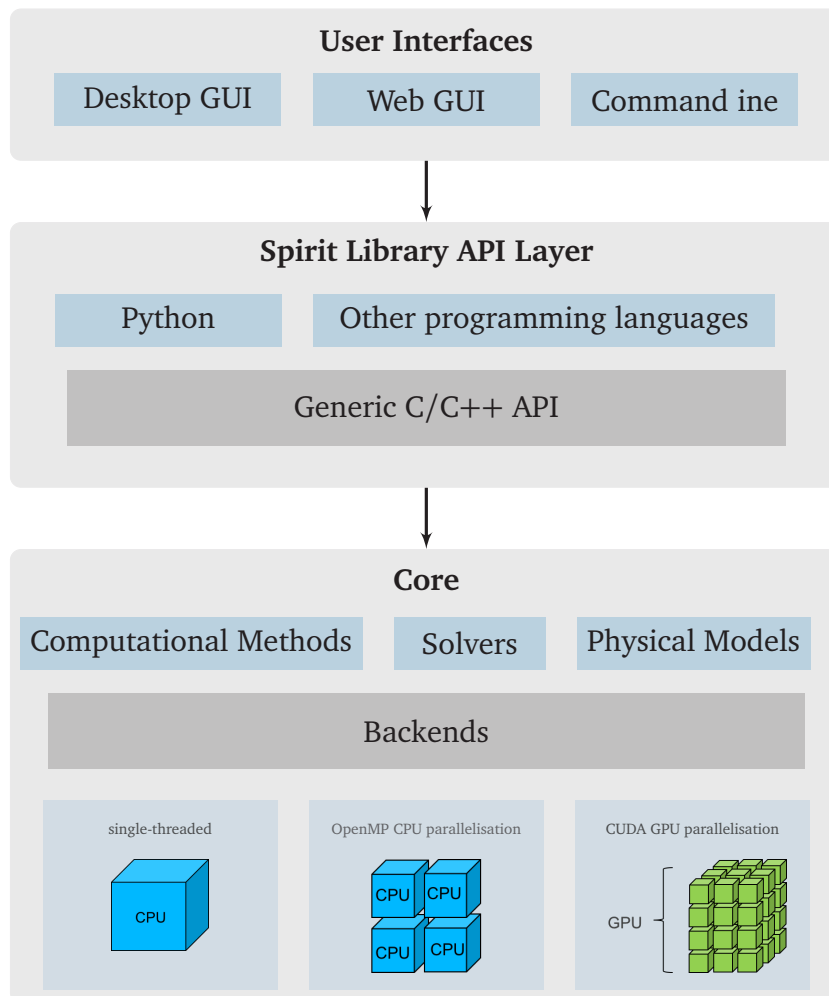
FIGURE 3.1 – Schematic of Spirit code structure
