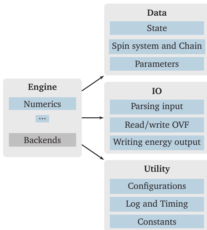
FIGURE 3.4 – Schematic of Spirit core library layout
