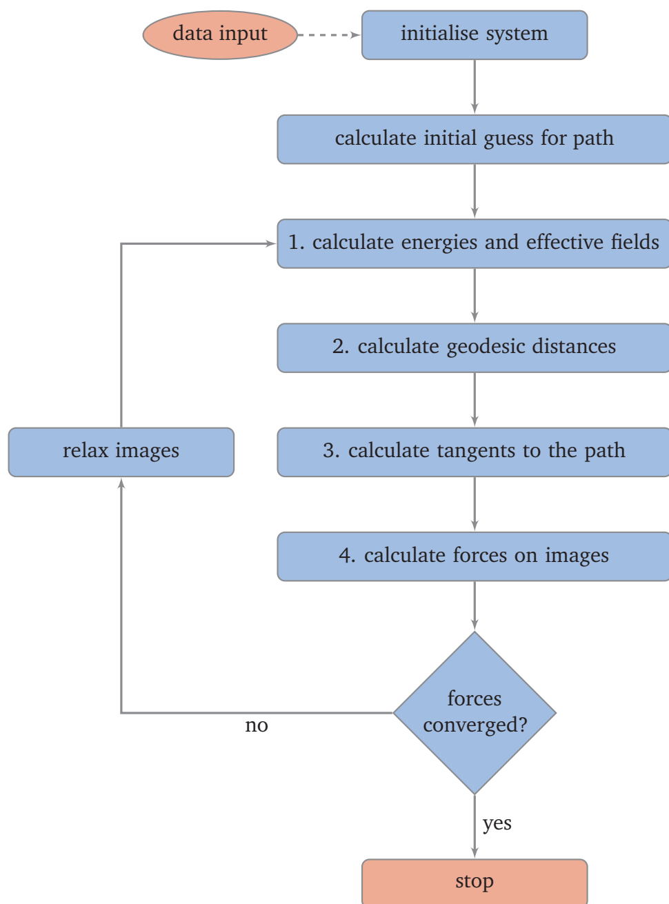
FIGURE 1.3 – Flow chart of the GNEB algorithm
