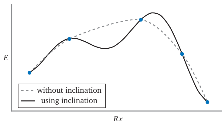
FIGURE A.1 – Interpolation with hermite polynomials
