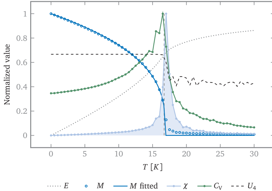
FIGURE I.13 – LLG temperature test system
