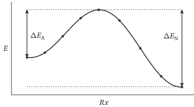
FIGURE 1.1 – Schematic energy barrier
