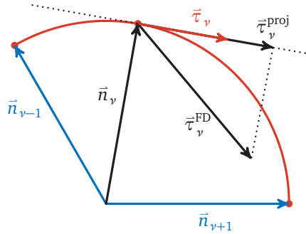
FIGURE 1.4 – Path tangents projection
