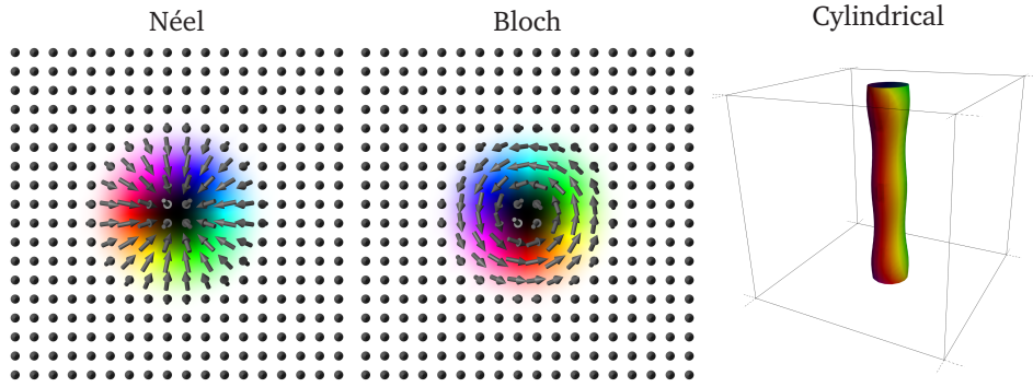
FIGURE 1.3 – Skyrmions in two and three dimensions
