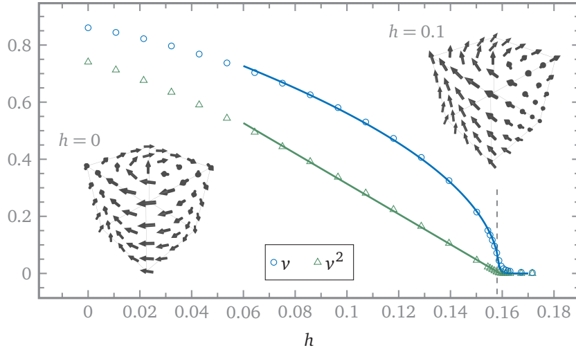
FIGURE 3.9 – Stray field-caused vorticity of a cube
