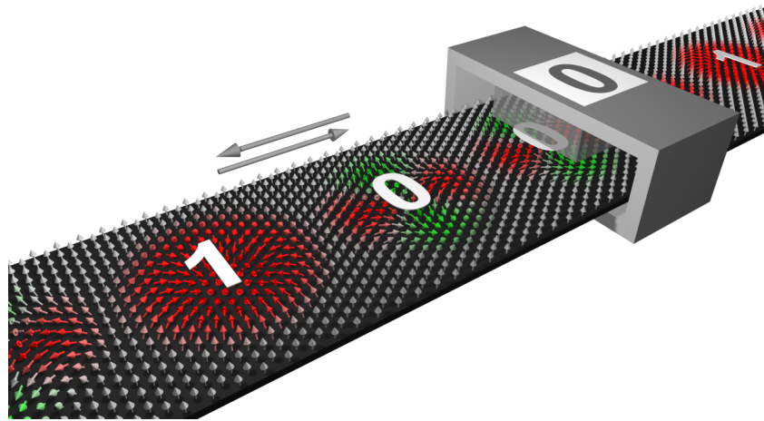
FIGURE I.4 – Skyrmions and antiskyrmions on a racetrack
