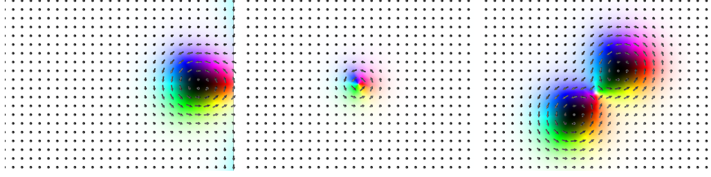
FIGURE 2.8 – Saddle points of three skyrmion transitions: escape, collapse and duplication
