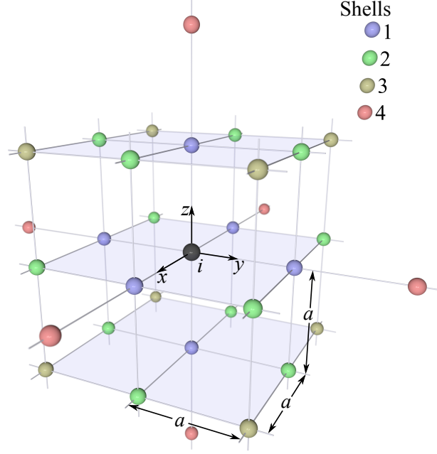
FIGURE I.6 – Visualisation of neighbour relations on a simple cubic lattice
