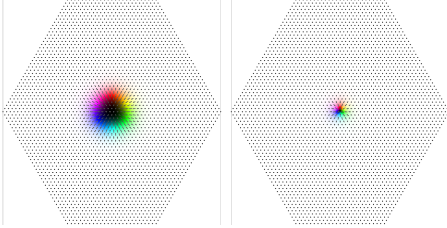
FIGURE 1.27 – Skyrmion and collapse saddle point in hexagonal lattice
