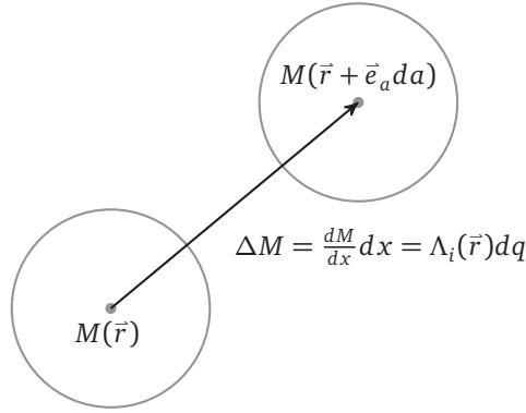
FIGURE 1.23 – Schematic visualisation of translational skyrmion mode
