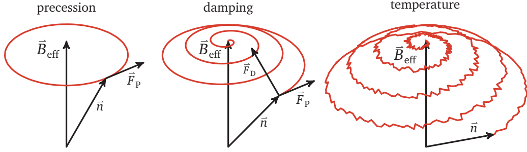
FIGURE I.10 – Schematic of spin movement under LLG equation
