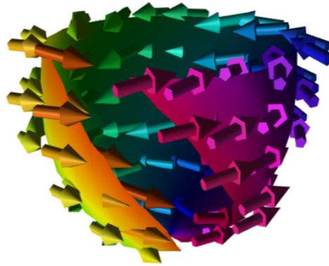
FIGURE 4.1 – Chiral bobber visualised in Spirit
