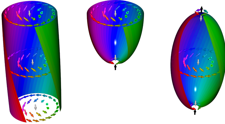
FIGURE 4.4 – Comparison of skyrmion bobber and globule
