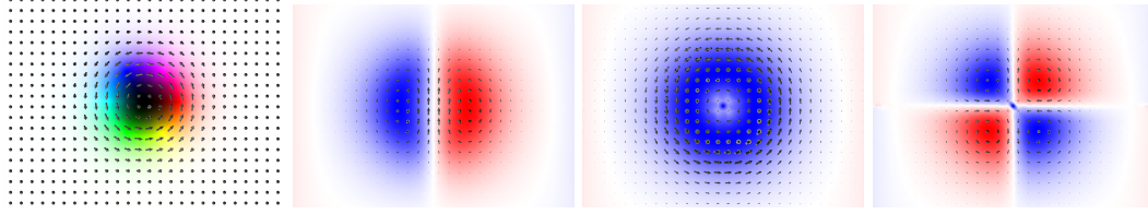
FIGURE 2.7 – Lowest three eigenmodes of an isolated skyrmion
