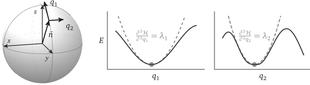
FIGURE 1.22 – Schematic of spin perturbation
