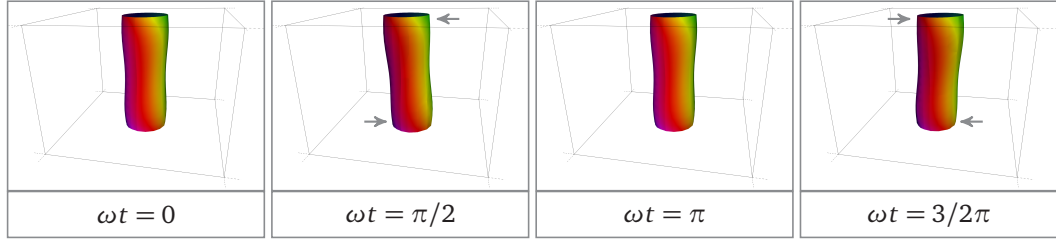
FIGURE 2.3 – Eigenmode of a skyrmion tube
