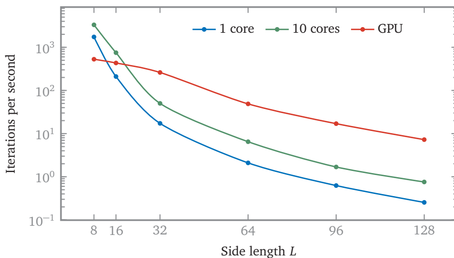
FIGURE 3.3 – Performance scaling of Spirit over system size
