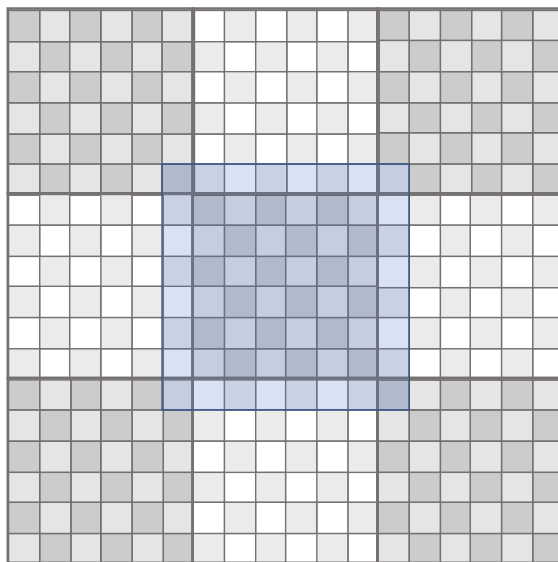
FIGURE 3.8 – Checkerboard domain decomposition for parallelised Monte Carlo
