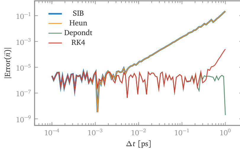
FIGURE 3.10 – Solvers' precession error over time step
