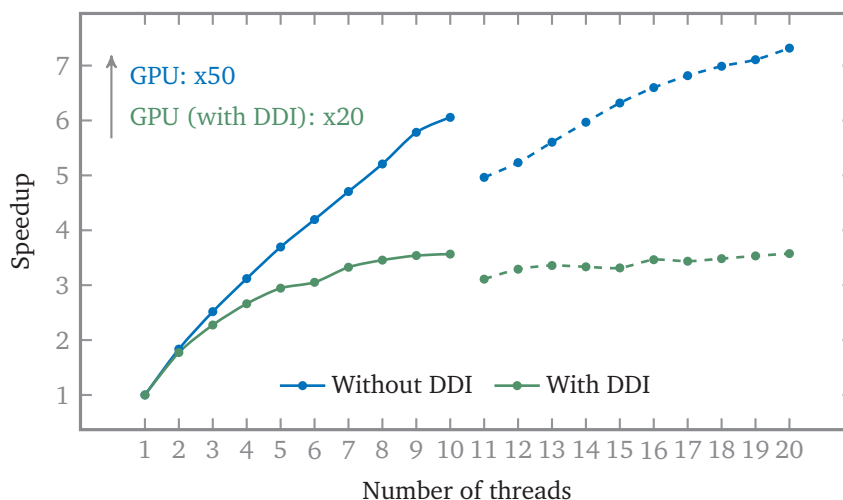
FIGURE 3.2 – Performance scaling of Spirit over number of parallel threads
