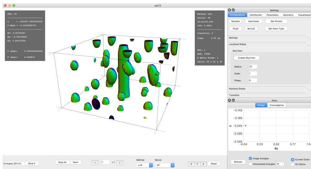
FIGURE 3.5 – Screenshot of Spirit graphical user interface (GUI)
