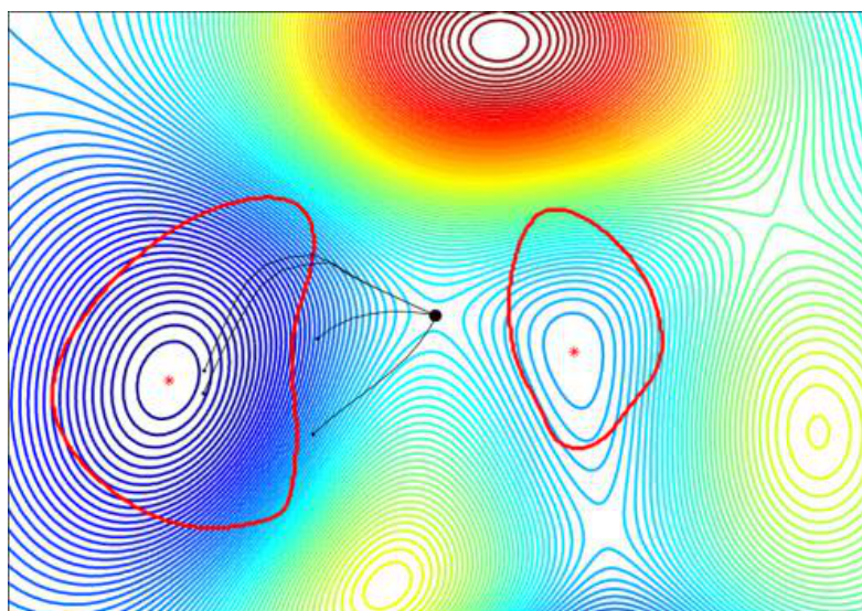
FIGURE 2.1 – MMF paths for atomic 2D system
