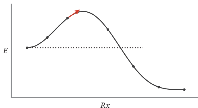
FIGURE 1.5 – Climbing image method
