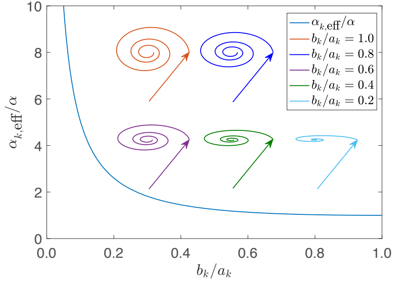
FIGURE 1.24 – Dynamical eigenmode trajectories of a single spin
