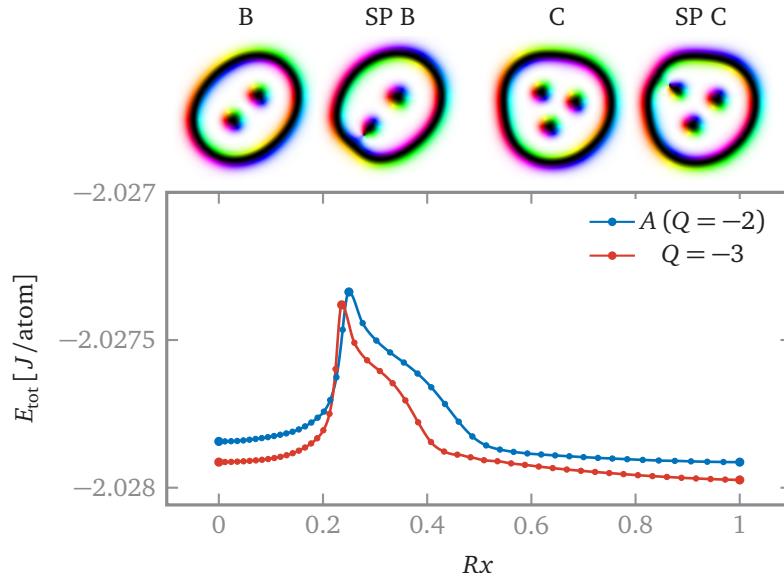
FIGURE 1.19 – Skymion colliding with the "sack" wall
