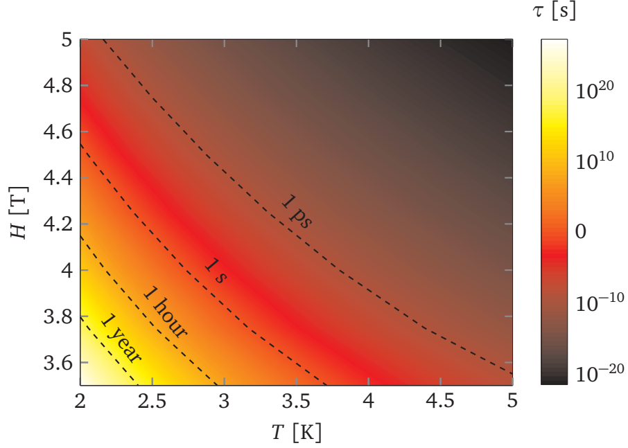
FIGURE 1.29 – HTST Arrhenius plot for the skyrmion collapse
