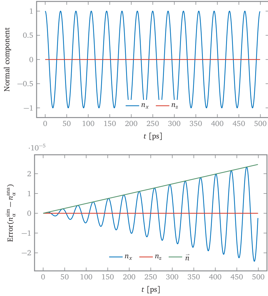
FIGURE I.11 – LLG dynamics: spin precession without damping
