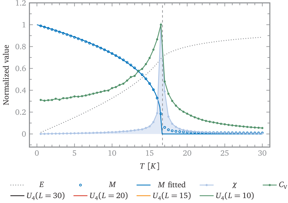
FIGURE I.8 – Monte Carlo test system
