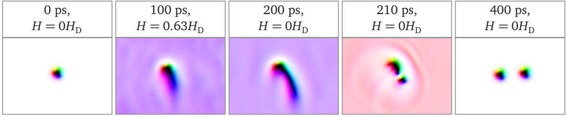
FIGURE 2.11 – Dynamics simulation of skyrmion duplication
