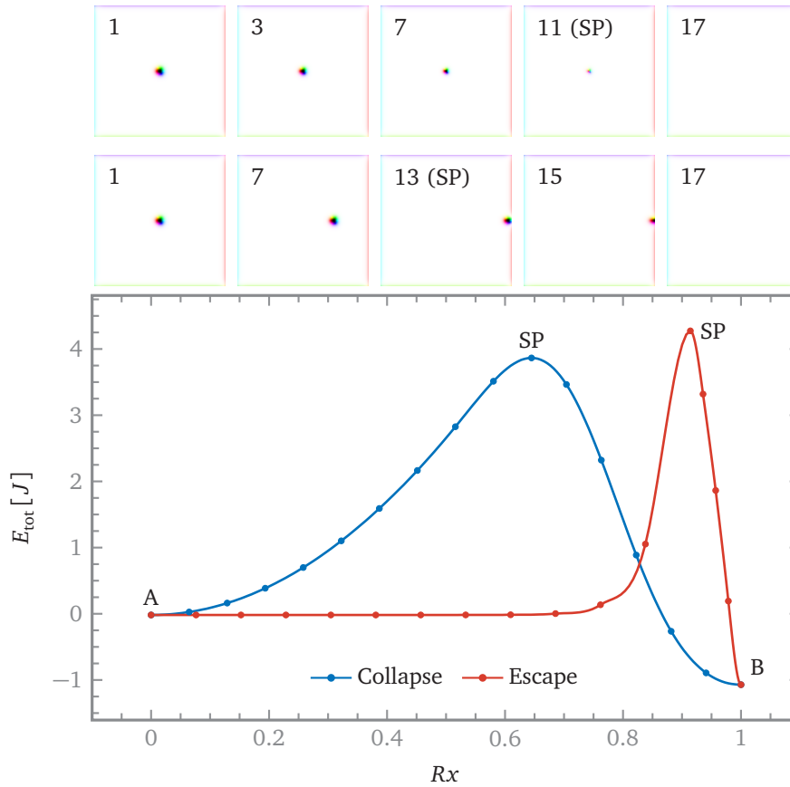
FIGURE 1.9 – Skyrmion transitions: minimum energy paths
