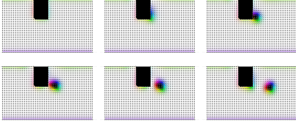
FIGURE I.15 – Skyrmion nucleation under current
