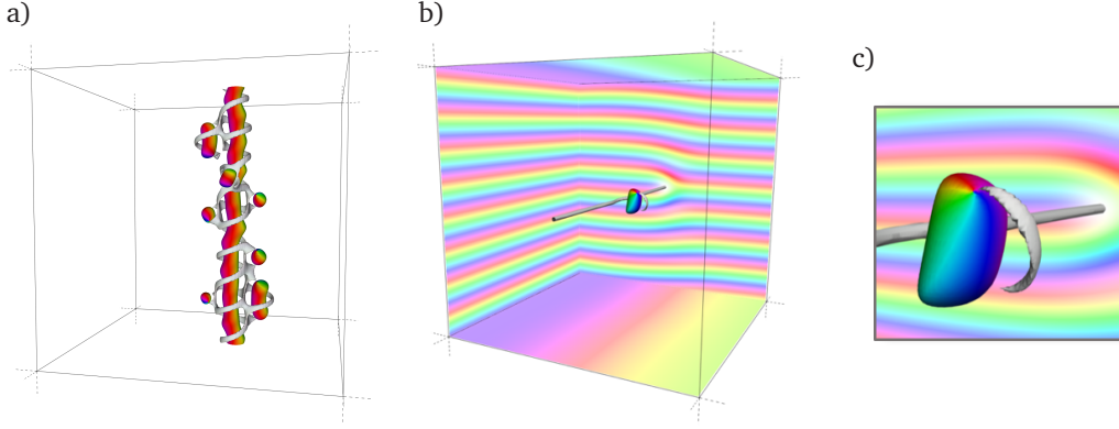
FIGURE 4.5 – Magnetic globules in bulk systems
