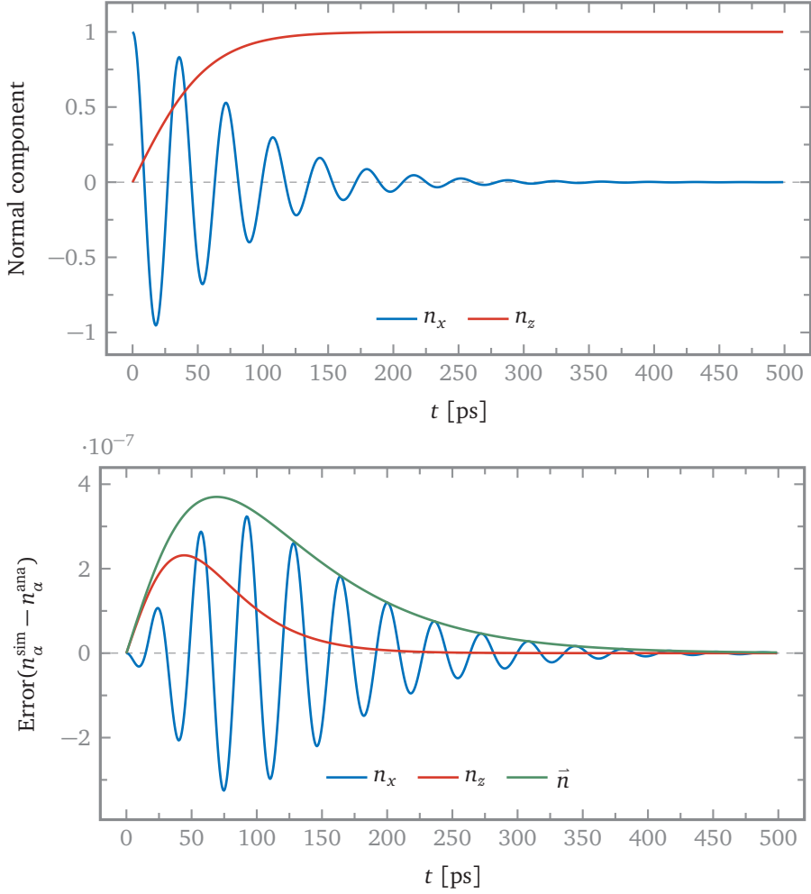
FIGURE I.12 – LLG dynamics: damped spin precession
