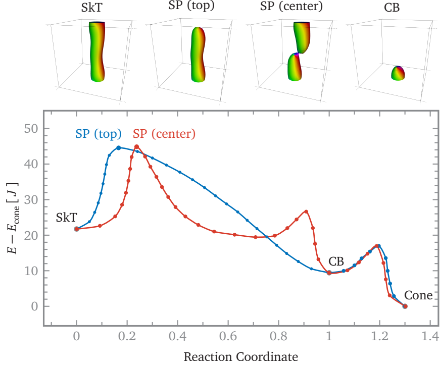
FIGURE 4.2 – GNEB path for skyrmion collapse with intermediate bobber
