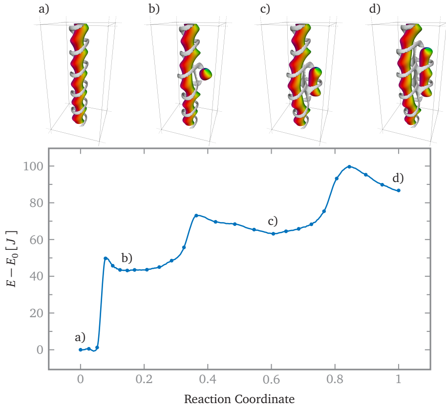
FIGURE 4.6 – Skyrmion-globule GNEB path in the bulk
