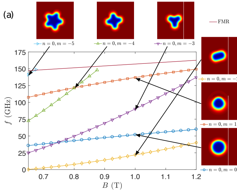
FIGURE 1.25 – Dynamical skyrmion modes
