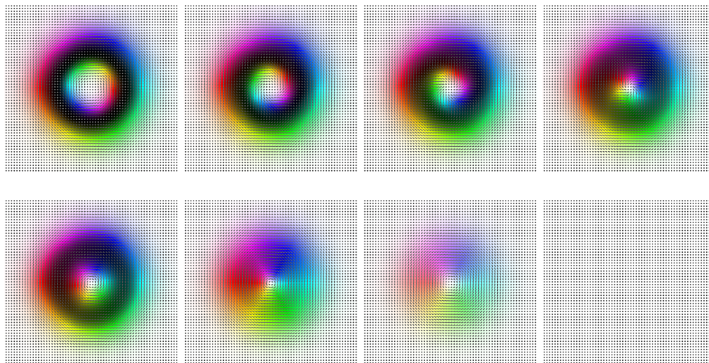
FIGURE 1.13 – Homotopy transformation of the skyrmionium
