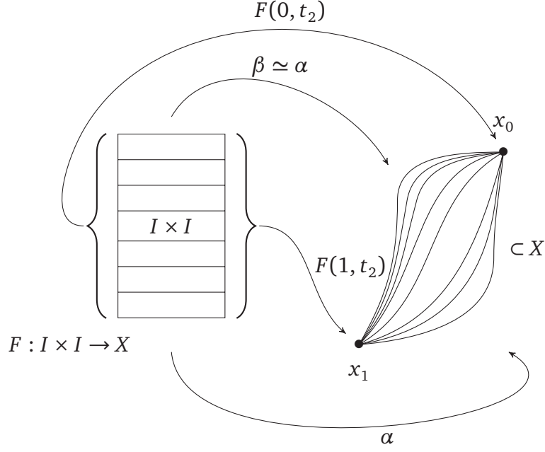
FIGURE 1.12 – Homotopy transformation
