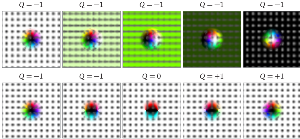
FIGURE 1.11 – Transformations between a skyrmion and an antiskyrmion
