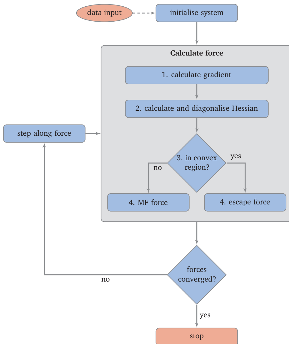
FIGURE 2.2 – Flow chart of the MMF algorithm
