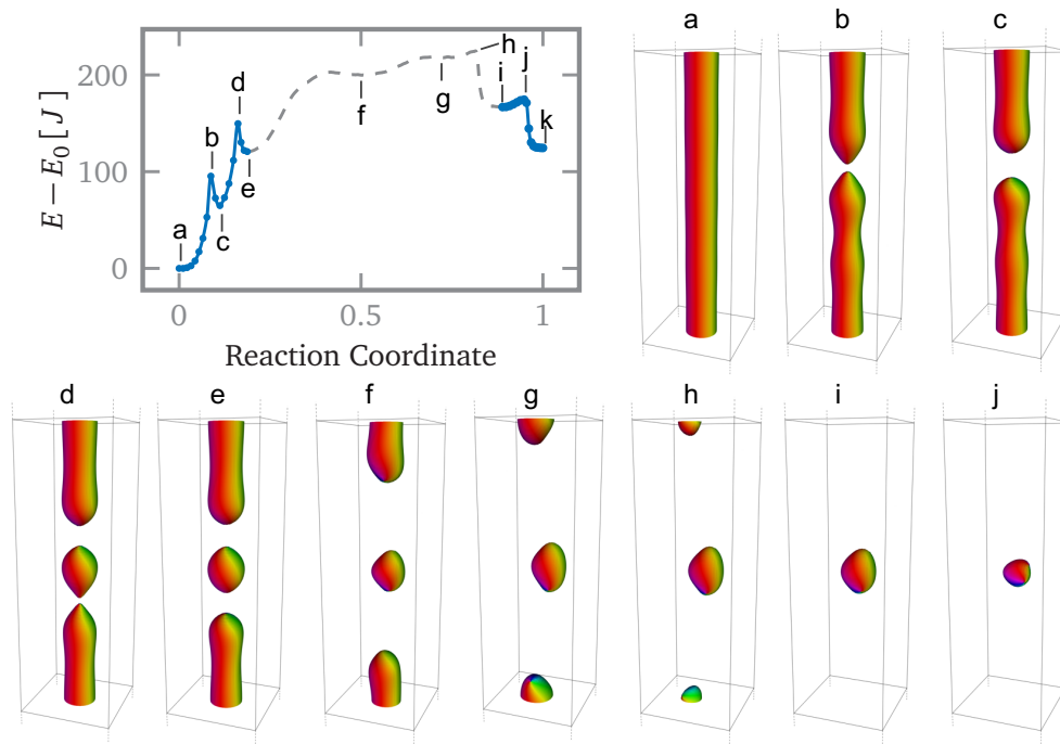
FIGURE 4.10 – Globule collapse GNEB Path
