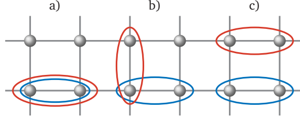
FIGURE I.7 – Quadruplet interactions
