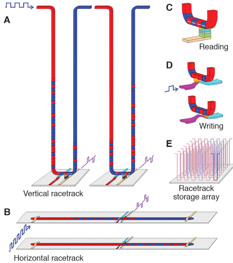
FIGURE 1.1 – Domain wall racetrack memory concept
