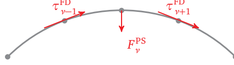
FIGURE 1.6 – Path shortening force to eliminate zero modes
