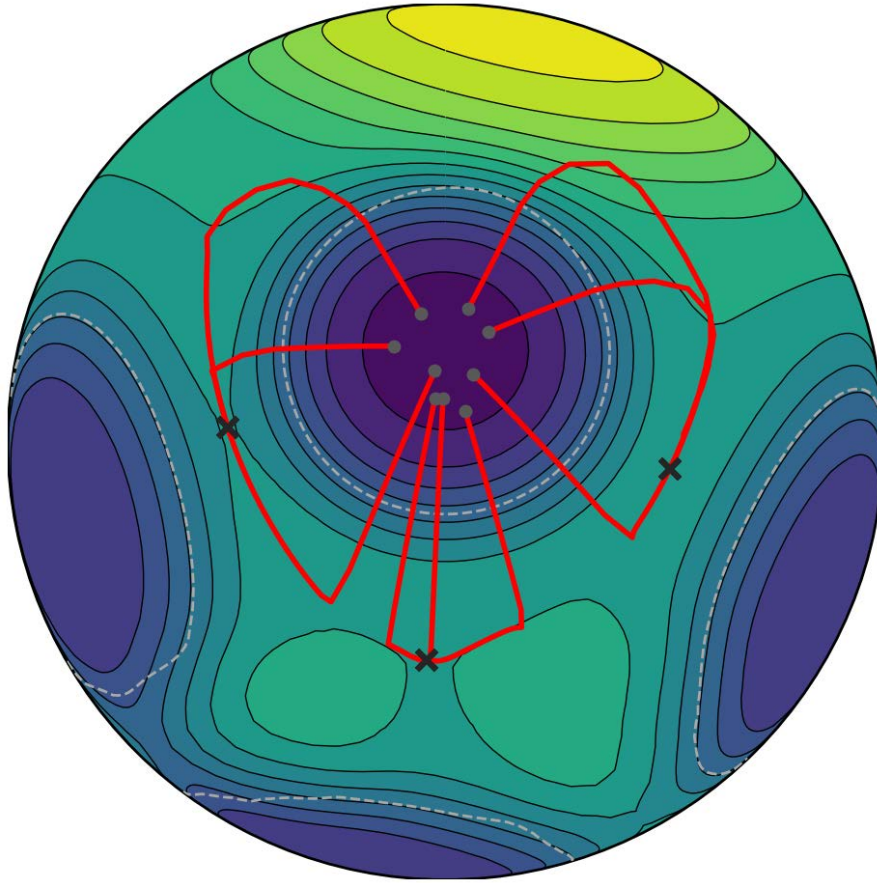
FIGURE 2.4 – Mode following path of a single spin
