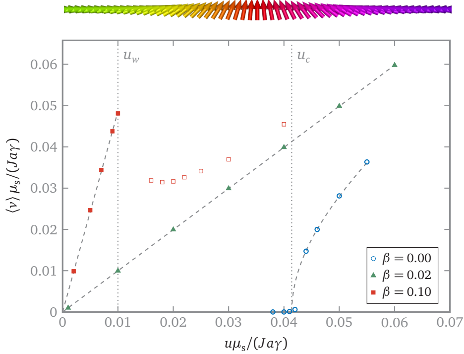
FIGURE I.14 – Domain wall motion under current
