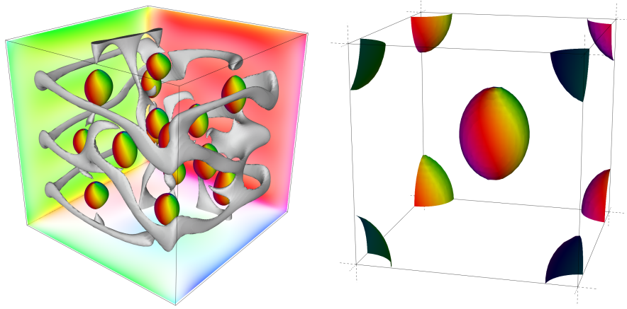
FIGURE 4.11 – Globule lattices
