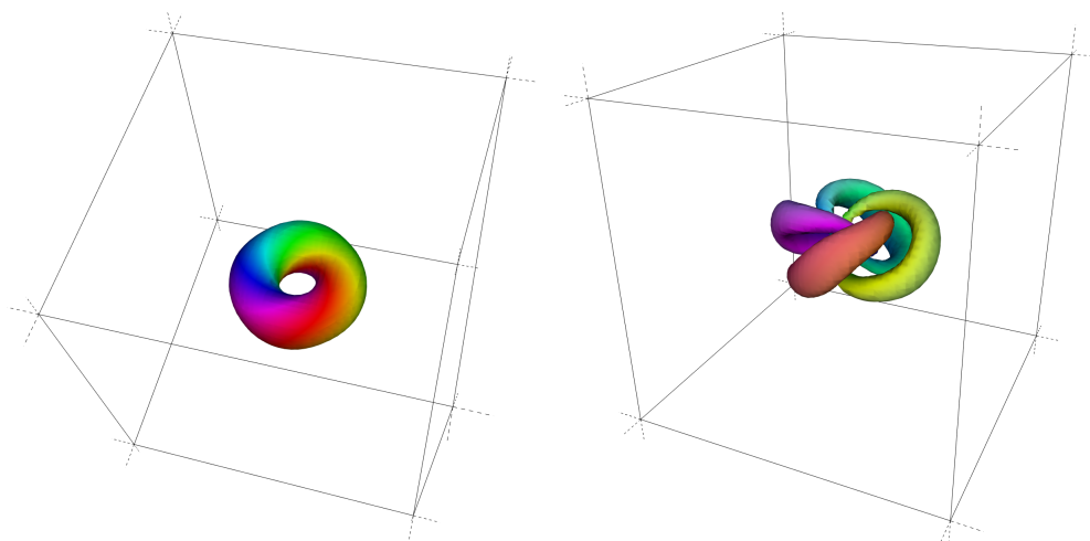
FIGURE 3.17 – Hopfion isosurface visualisations
