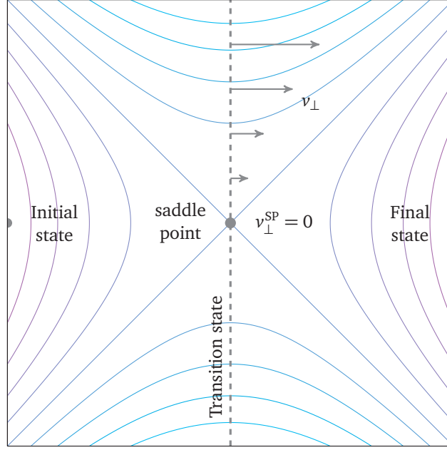
FIGURE 1.21 – Visualisation of the dividing surface in HTST
