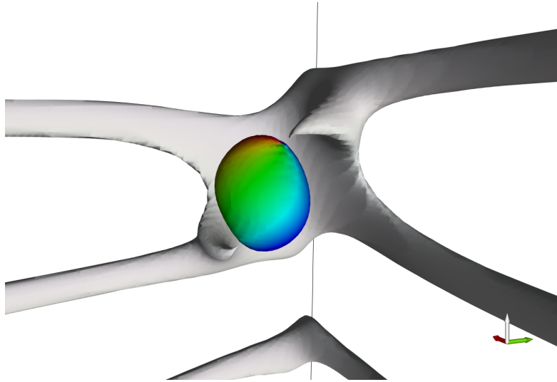
FIGURE 4.8 – Globule attached to nanowire edge state
