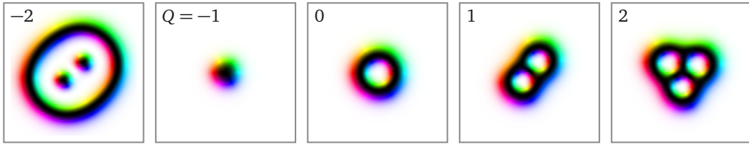
FIGURE 1.10 – Skyrmion "sacks"
