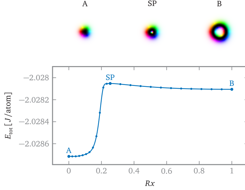
FIGURE 1.16 – Collapse of a skyrmionium to a skyrmion
