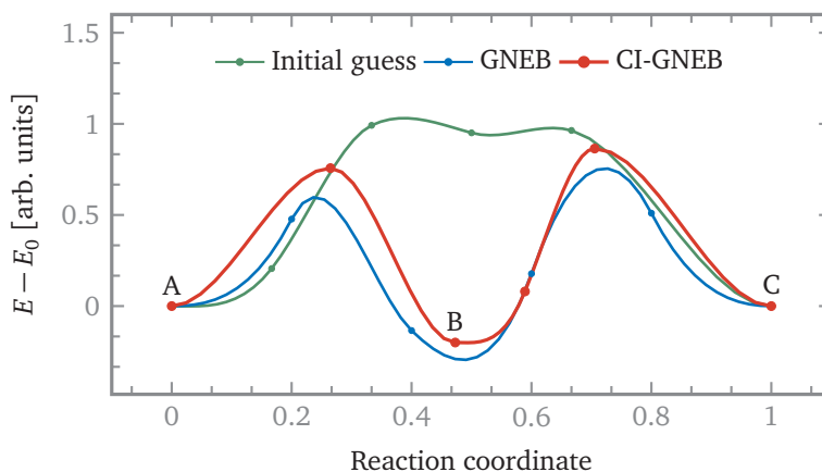
FIGURE 1.8 – Single spin energy barriers
