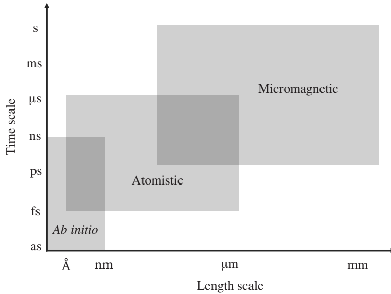
FIGURE I.5 – Hierarchy of time and length scales
