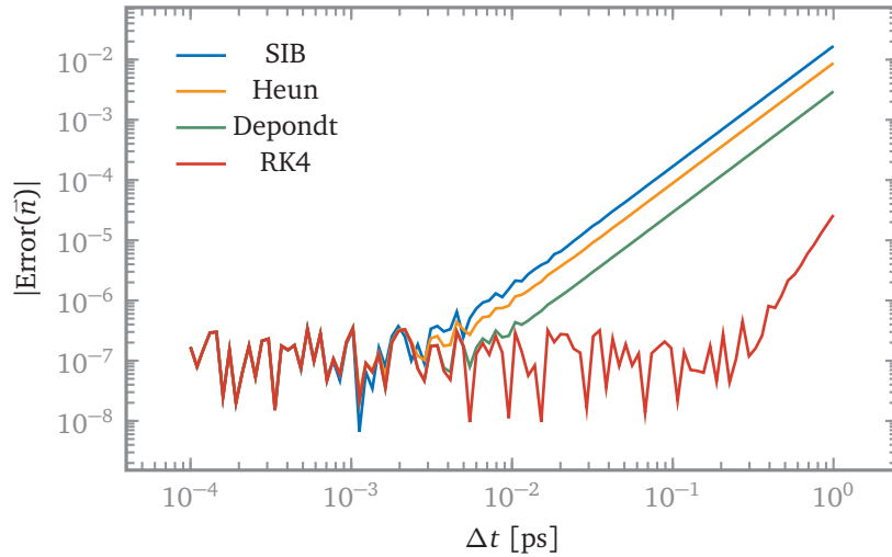
FIGURE 3.11 – Solvers' error dependence on time step
