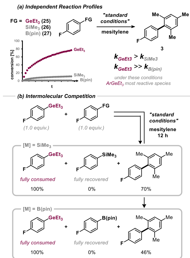
Figure 3. \text{ArGeEt}_3 , under these conditions most reactive site compared to \text{ArSiMe}_3 and \text{ArB(pin)} . Standard conditions: [(\text{Ph}_3\text{P})\text{Au}][\text{Cl}] (5.0 mol %), \text{PhI}(\text{OAc})_2 (1.5 equiv), \text{CSA} (1.5 equiv) in 1,4-dioxane (0.3 M) at 70 °C. Quantification by ^{19}\text{F} NMR analysis.
