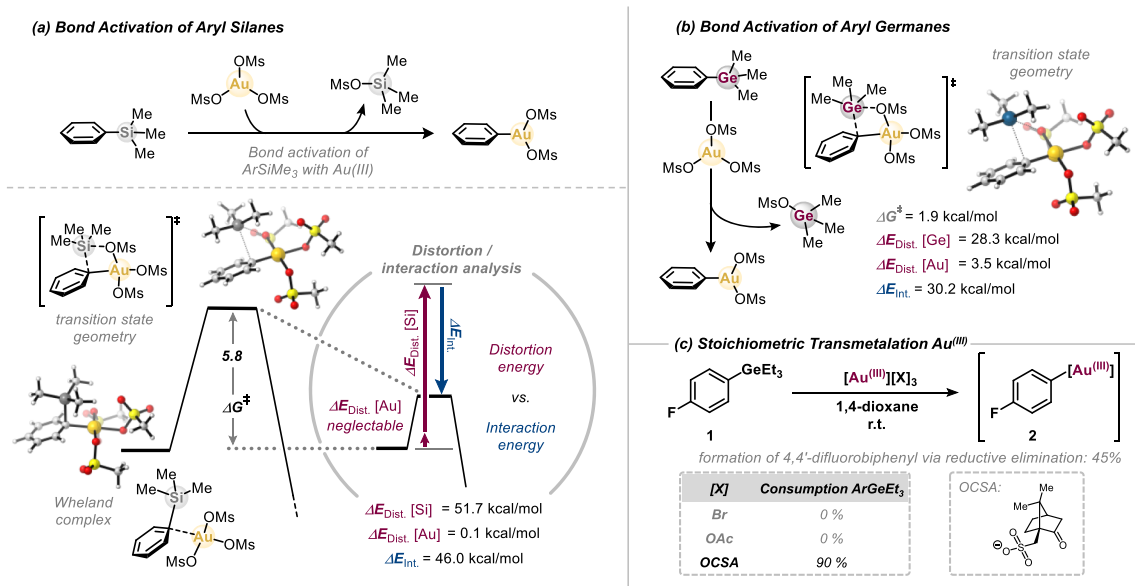
Figure 2. Computational and experimental investigation of bond activation of ArSiMe 3 and ArGeEt 3 with Au III . Transition-state barriers were computed at the CPCM (dioxane) M06L/6-311++G(d,p)//ωB97XD/6-31G(d) [with LANL2DZ for Au] level of theory. For computational and experimental details, see the Supporting Information . 12 OCSA = camphorsulfonate.
