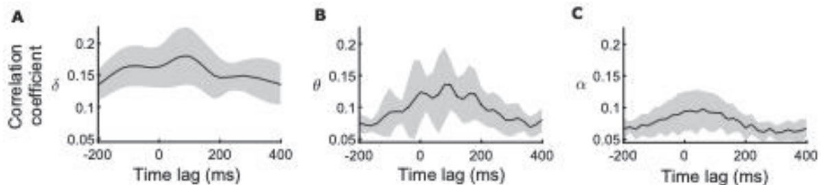
Figure 3 – Reconstruction of the speech envelope from EEG recordings. The correlation coefficient between the reconstructed envelope and the actual one measures the goodness of the reconstruction. We show the correlation coefficient for reconstructions using temporal lags from -200 ms to 400 ms, and for the delta frequency band (A), the theta frequency band (B), and the alpha frequency band (C).
