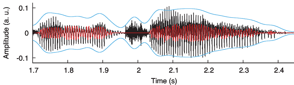
Figure 1 – Speech (black) is a complex signal. Two important quantities are its envelope (blue) as well as the fundamental frequency of the voiced parts of speech that give rise to the fundamental waveform (red).
