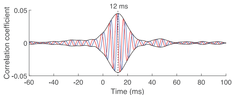
Figure 2 – The cross-correlation of the fundamental waveform of continuous speech with the scalp-recorded brainstem response (blue) peaks at around 12 ms. We show also its Hilbert transform (red) and the envelope (black).
