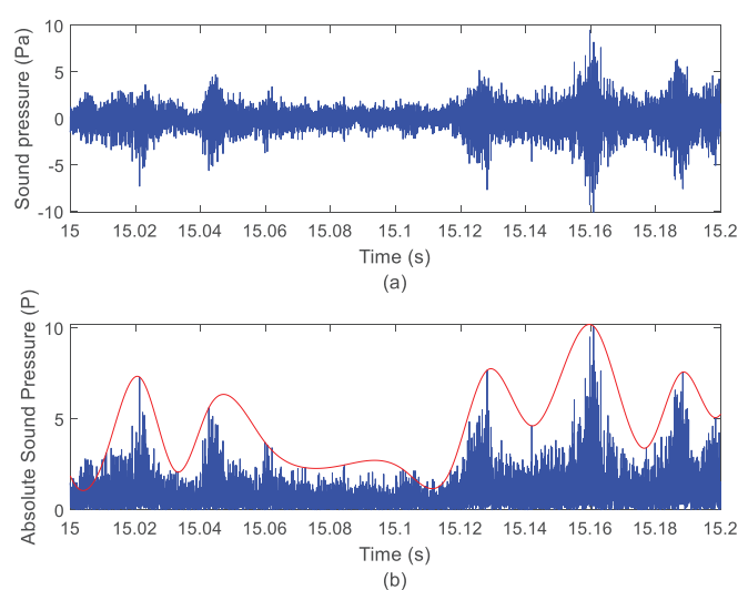
Figure 5 – (a) Measured sound pressure and (b) the estimated envelope on the absolute sound pressure.
