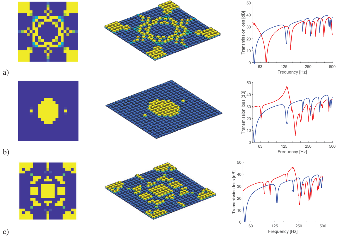
Figure 1. Thickness and sound insulation curve of of the plate optimized at a) 53, b) 132 Hz and c) 210 Hz. The sound insulation of the optimized plate is shown in red and the sound insulation of the reference plate is shown in blue. The frequency at which the optimization is performed is indicated with a dot.
