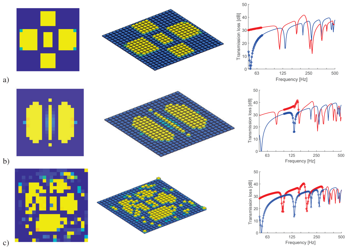
Figure 2. Thickness and sound insulation curve of of the plate optimized in a frequency band of a) 50-100 Hz, b) 100-150 Hz and c) 50-300 Hz. The sound insulation of the optimized plate is shown in red and the sound insulation of the reference plate is shown in blue. The frequencies at which the optimization is performed are indicated with a dot.
