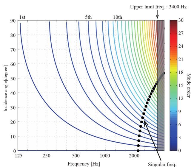
Figure 3 – Measurable frequency range and incidence angles in the chamber.
