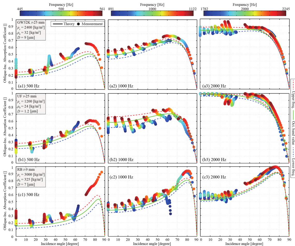
Figure 10 – Oblique-incidence absorption coefficients measured for three porous materials in 1/3-octave bands of 500, 1000 and 2000 Hz: (a) glass wool, (b) urethane foam, (c) rock wool board.
