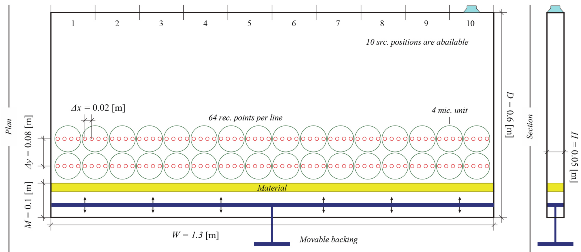
Figure 2 – Geometry of the thin chamber with two microphone arrays and a loudspeaker.
