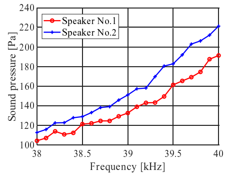
Figure 2. Frequency - sound pressure characteristics of speakers when input voltage is 2 V_{pp} .
