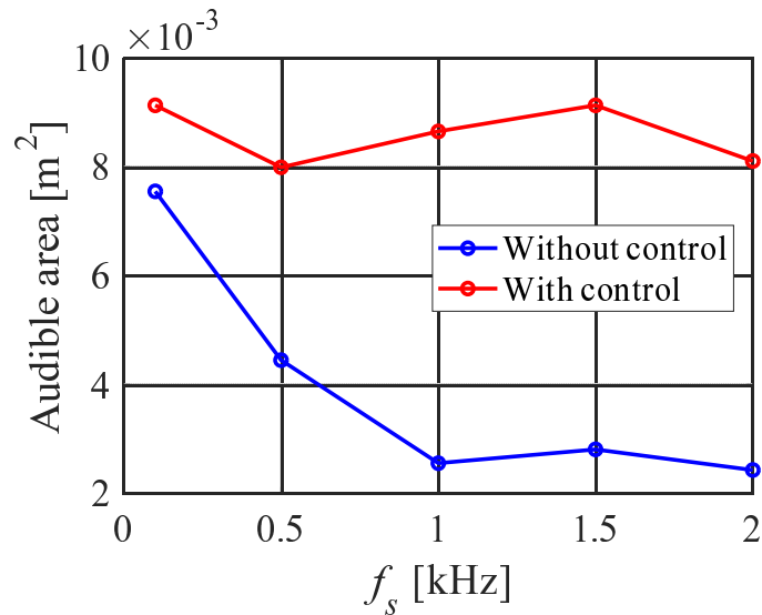
Figure 5. The area of audible spot.
