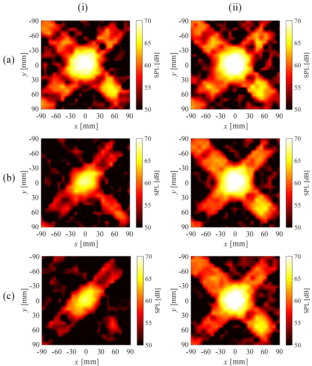
Figure 4. Measured sound fields when (a) f_s = 0.1 kHz, (b) f_s = 1 kHz, (c) f_s = 2 kHz. (i) Results without control, (ii) with control.
