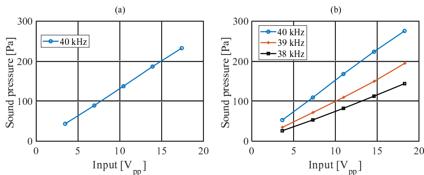
Figure 3. Input - sound pressure characteristics of (a) speaker No. 1, (b) speaker No. 2.
