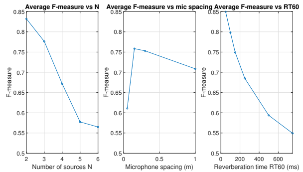
(b) Average F-measure of the proposed algorithm as a function of the number of sources (left), microphone spacing (center) and reverberation time RT_{60} (right) for the 2-channel dataset.
