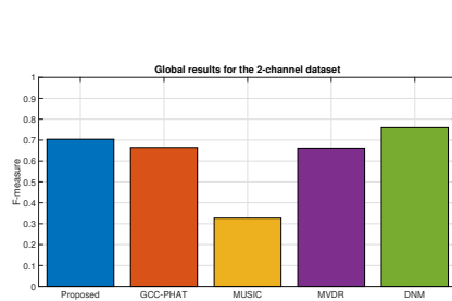
(a) Average F-measure of the proposed algorithm and the state-of-the-art methods for the 2-channel dataset.
