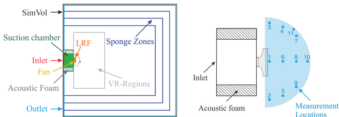
Figure 3 – Simulation model (left) and measurement locations (right)
