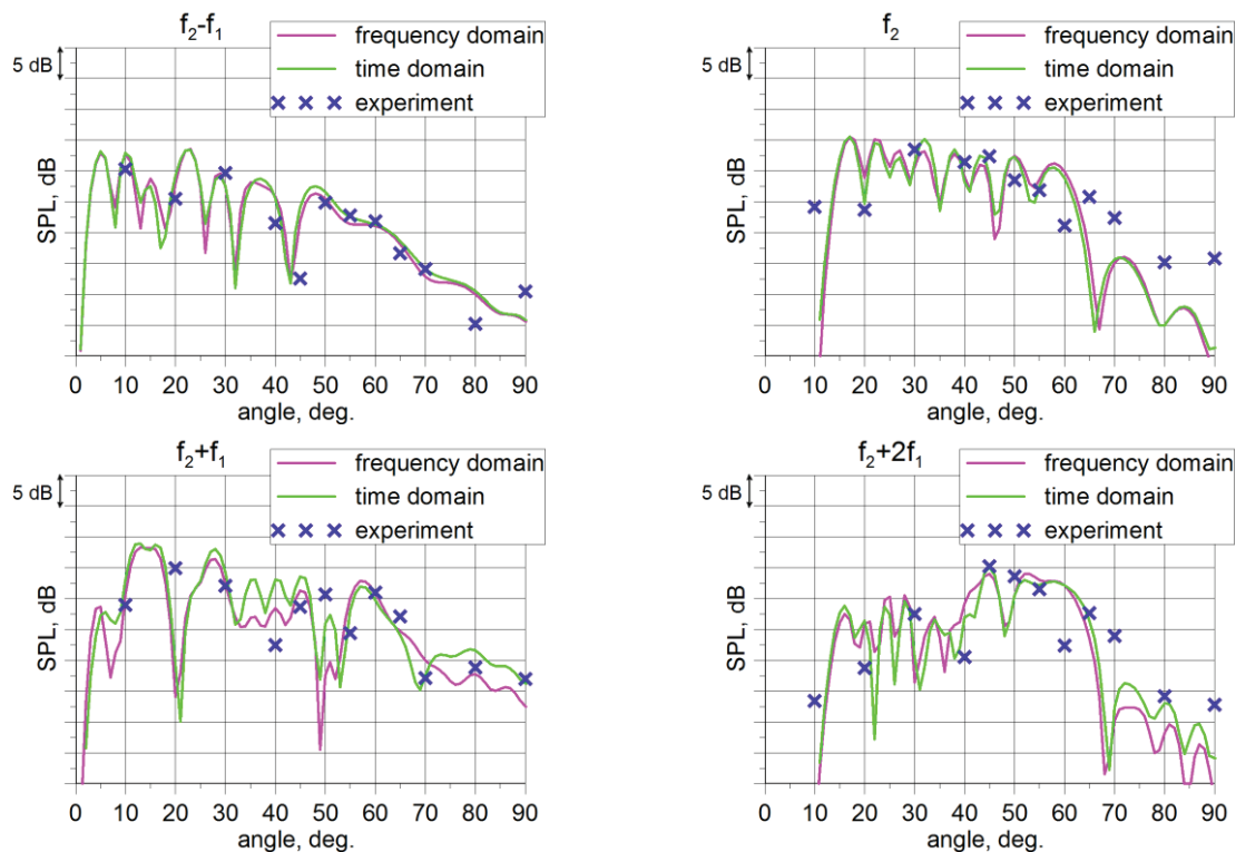
Figure 5. – Comparison between computational and experimental directivity diagrams in a forward hemisphere
