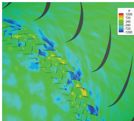
Figure 3. – Unsteady pulsations of static pressure field on the section of constant diameter d=0.5D
