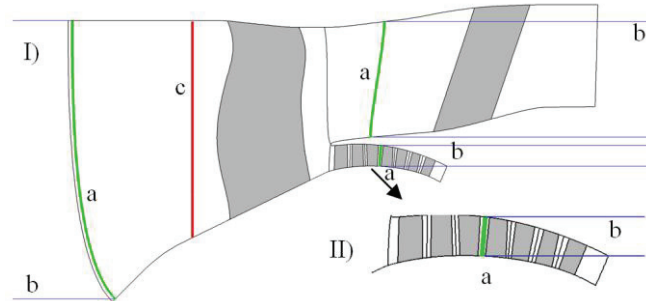
Figure 2. - Scheme of the computational domain: I) Low pressure compressor; II) Booster. Here: a - the boundaries of the fine grid region in the computational domain; b - the boundaries of buffer blocks (shown only partially); c - the surface for modal analysis upstream of the fan
