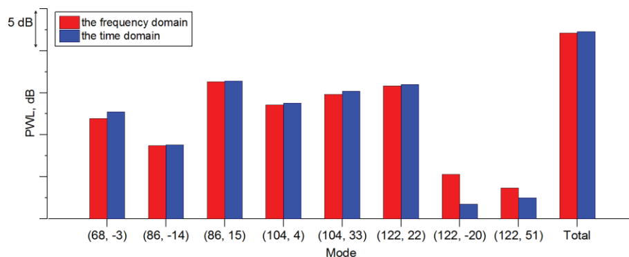
Figure 4. – Results of the modal analysis upstream of the fan. The modes are designated by the pair of integers (h,m) .
