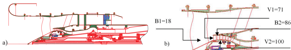
Figure 1. - Scheme of the fan model: a) general view; b) magnified fragment
